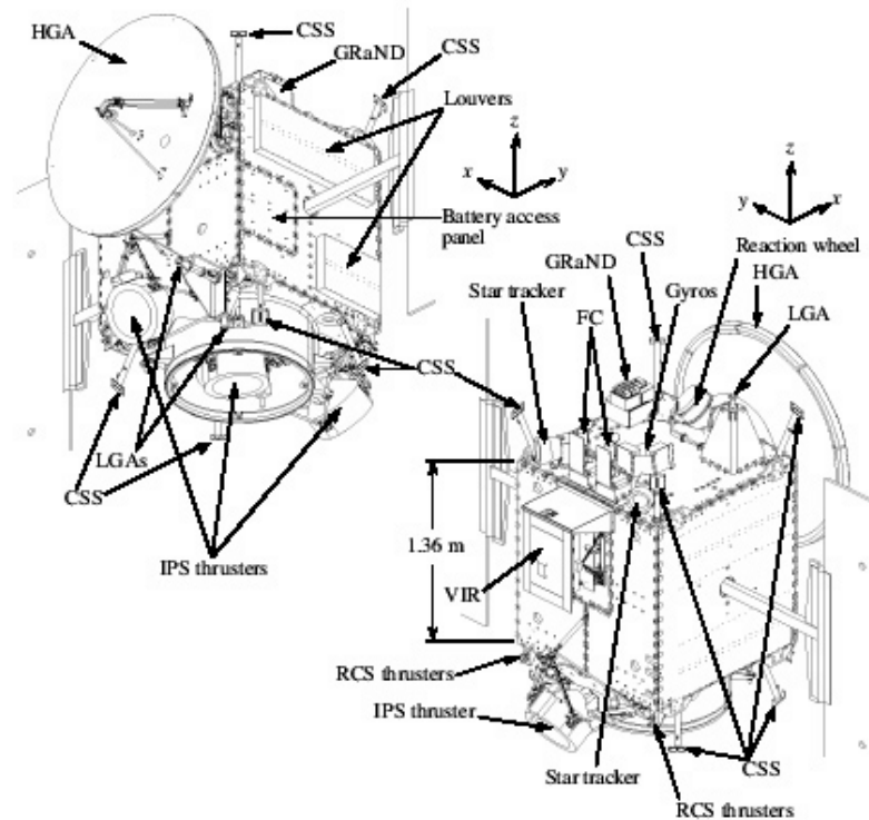
Figure 1.15: Diagram of Dawn spacecraft (from http://dawn.jpl.nasa.gov/mission/spacecraft.asp ). The upper left view shows the High gain antenna (HGA) used for communicating with Earth and the three Ion Propulsion Thrusters (IPS). The Z axis corresponds to the direction pointing towards the observed object during mapping orbits. The visible-infrared spectrometer (VIR) is set on the opposite panel to the communication antenna (lower right view). The pair of framing cameras (FC) seat just above VIR on the panel which is opposite to the main thruster. The Gamma Ray and Neutron Detector (GRaND) is the set on the same panel on the upper left corner.
