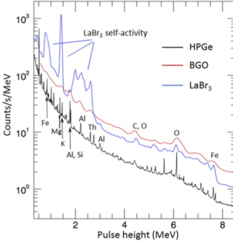
Figure 2.2: From [Prettyman, 2014]: "Comparison of whole Moon gamma ray spectra acquired by Lunar Prospector (BGO, red), Kaguya (HPGe, black), and Chang'E-2 (LaBr 3 , blue)". The spectral resolution of BGO spectra is \sim 20 times lower than HPGe and about two times lower than LaBr 3 . LaBr 3 has a self activity visible below E_\gamma \sim 3 MeV which masks low energy features such as K and Th peaks.
