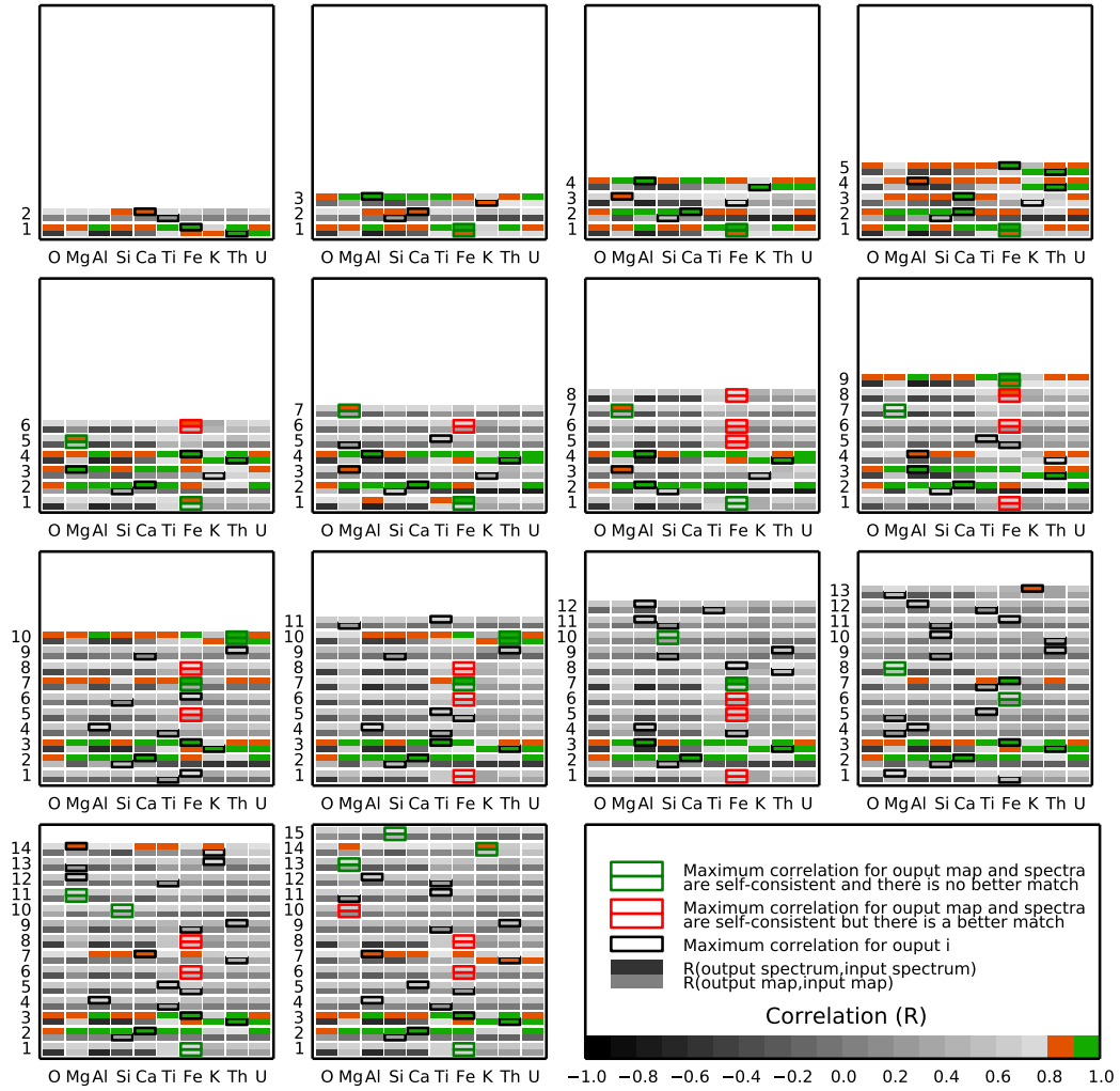
Figure A.4: Correlation matrices between library data and source extracted from the LP-GRS data by ICANMF as a function of the number of output sources from 2 to 15.
