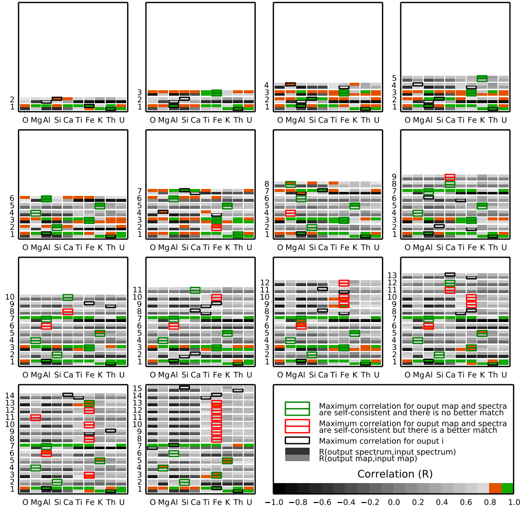
Figure A.2: Correlation matrices between library data and ICA-NMF outputs. The analyzed dataset was produced from the physical mixture model of equation 2.4, including all elements. The background gamma rays B_{pl} were not included.
