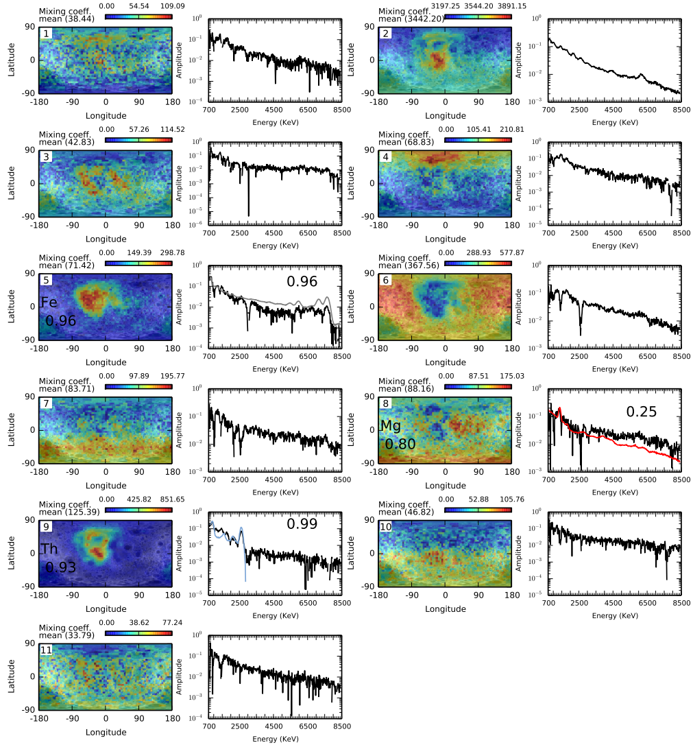
Figure 2.23: ICA-NMF applied to synthetic gamma ray spectra following the model of Prettyman et al. [2006] in the presence of a background. The number of output sources was set to 11. This case is shown because it corresponds to the situation where a maximum of elements can be recognized with a significant degree of correlation with theoretical elemental contributions. Each pair of plots shows the output sources (right) and mixing coefficients (left). Fe, Th and Mg are assigned by the element recognition procedure described in section 2.4.4.
