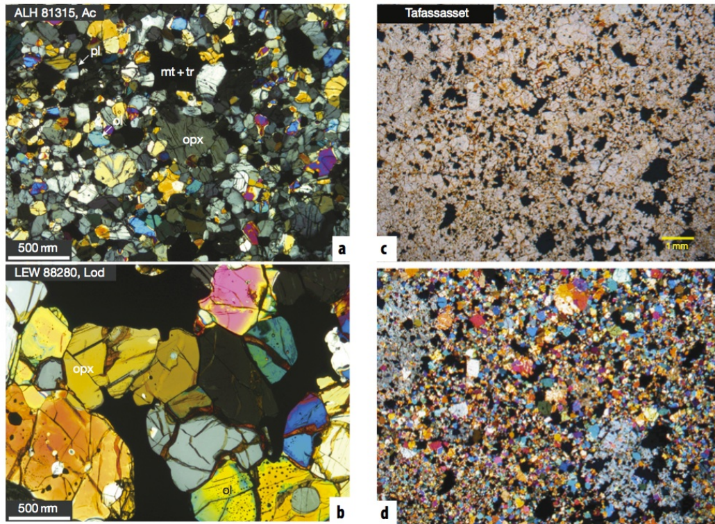
Figure 1.5: Photomicrographs of primitive achondrites from [Krot et al. , 2014] "a Aca-pulcoite ALH 81315 and b lodranite LEW 88280 have similar mineralogy (mostly orthopyroxene, olivine, Cr-diopside, Na-plagioclase, FeNi-metal, and troilite), but different grain size. Photograph courtesy of G. Benedix. c Plane-polarized and d cross-polarized light micrographs showing the general texture of Tafassasset. Tafassasset is dominated by olivine (70 vol%) with minor pyroxene and plagioclase. Opaque areas are dominantly FeNi-metal, which makes up 7% of the meteorite. Sulfide is minor (< 2%)."
