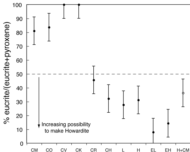
Fig. 4. Calculated proportion of eucrite (crust)/(eucrite+pyroxene) for each of the studied bulk compositions. Values of this parameter >50 (dashed line) make howardite formation unlikely due to a lack of pyroxene.
