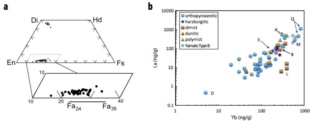
Figure 1.10: The variability of incompatible trace elements is strongly decoupled from that of the mineralogy in diogenites. a Compilation of pyroxene and olivine compositions from [McSween et al. , 2010] and references therein. b Compilation of trace element concentrations (La vs Yb) measured in diogenites from [Mittlefehldt et al. , 2011] and references therein. Most data points (blue dots) correspond to orthopyroxenitic lithologies. Dimict and polymict (brown rectangles and green triangles) are breccias where two or more petrological types of diogenites are mixed. Harzburgite here refers to diogenites including significant fractions of olivine ( \sim 30\% ). One dunite (90% Ol, orange triangle) sample is known in the HED collection.
