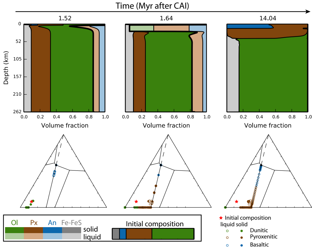
Figure 3.8: Predicted mineralogy inside Vesta as a function of depth and time. Vesta is assumed to be accreted instantaneously 1 Myr after the formation of CAIs, with an homogeneous composition. Soon after the onset of melting, a liquid rich in anorthite and pyroxene migrates upward, building a layer which accumulates below the conductive lid. Melt migration has the effect of concentrating fusible material in the subsurface region while the lower mantle enriches in refractory material. The subsurface liquid rich layer is modelled to homogenize when its liquid fraction exceeds 60% due to magma ocean convection. Overheating occurs in the subsurface region because it is enriched in anorthite which is the heat source carrier. This subsurface overheating leads to thermal erosion of the conductive lid, that is assumed to be recycled if it becomes thinner than 10 km. The competition between localized heating at ^{26}\text{Al} and cooling by surface recycling, takes place up to the decay of ^{26}\text{Al} . The more refractory olivine and pyroxene crystallize first and falls to the bottom of the magma ocean while rocks near the eutectic composition solidify in the uppermost layer (see text for details).
