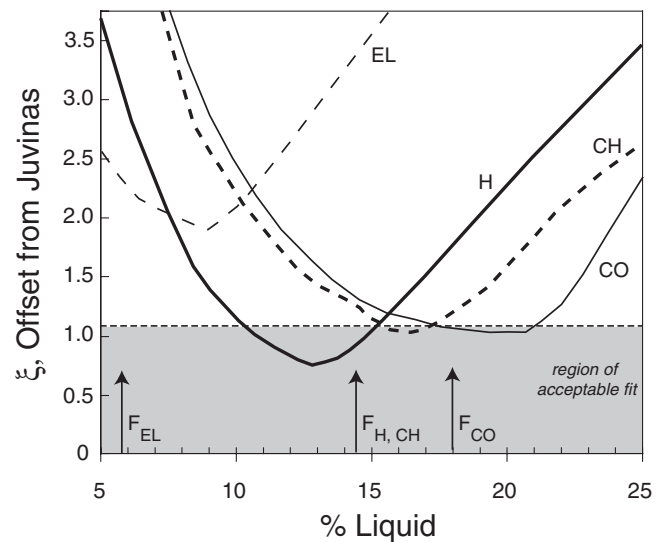
Fig. 5. Similarity of liquids predicted by MELTS to Juvinas, as a function of the fraction of liquid (see text for details), calculated for the silicate fraction of EL, H, CH, and CO groups. In all cases, the \text{Na}_2\text{O} content of the bulk composition was modified as described in the text. Values of \xi less than 1 indicate models that are indistinguishable from the composition of Juvinas at the 2 sigma level. Vertical arrows indicate the fraction of liquid expected for the EL, H, CH, and CO groups based upon analysis of their REE concentrations (see Table 1).
