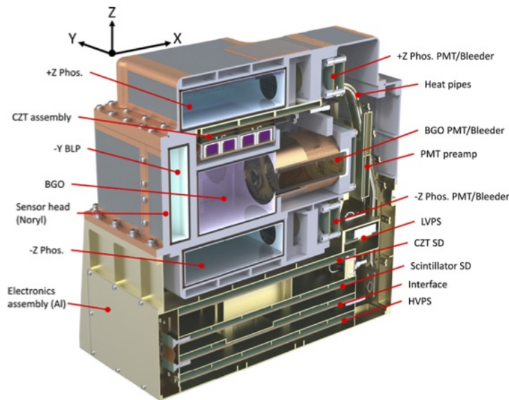
Figure 2.5: Cross section of the Gamma Ray and Neutron Detector onboard Dawn spacecraft from Prettyman et al. [2011]. The detection of gamma ray is enabled by the coupling of a BGO cristal (purple cube), which products visible light during interactions with gamma rays to a photomultiplier tube (PMT, orange cylinder) used to detect and amplify the light ouput from the scintillator.
