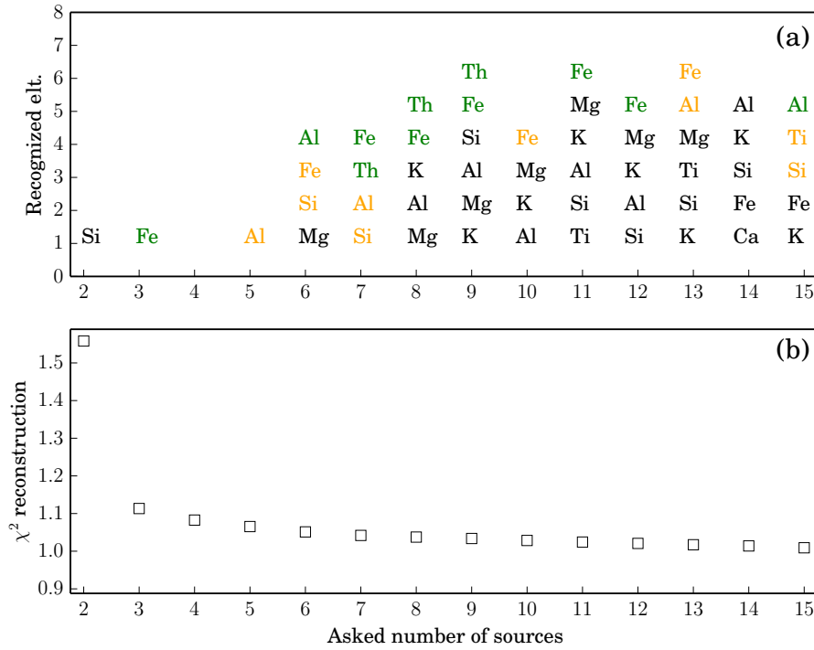
Figure 2.14: Performance of ICA-NMF applied to linear mixtures of ten elemental spectra. (a) Element recognized as a function of the number of output sources. (b) Average \chi^2_{red} between observed spectra \tilde{X}_{pl} and ICA-NMF reconstruction X_{rec}^{ICA-NMF} . Mg, Fe, K and Th can be reconstructed with a correlation better than 0.9 between the library data and the blind separation outputs when the number of output sources equals 9 and 10. Increasing further the number of sources does not seem to allow extracting more information as the signal reconstruction is not significantly improved.
