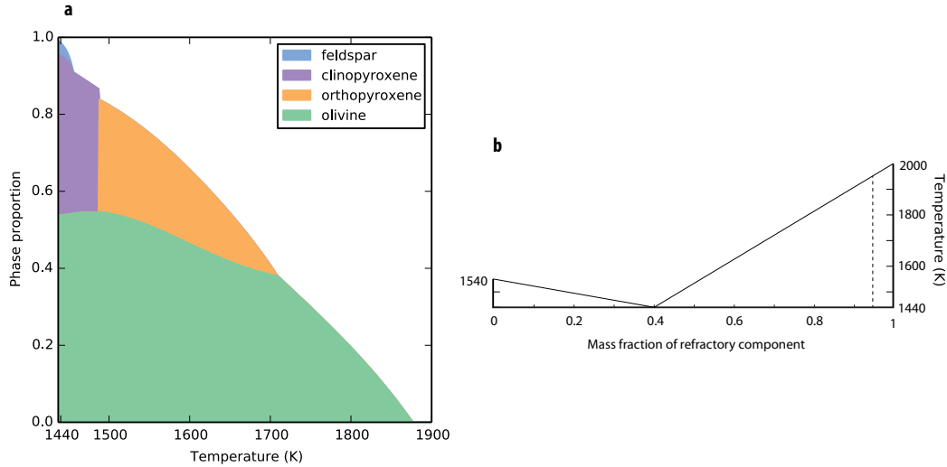
Figure 3.4: a: Fig. 11 from [Toplis et al. , 2013] "Phase proportions of liquid, olivine, pyroxene, and plagioclase as a function of temperature predicted by MELTS for equilibrium melting/crystallization of the silicate portion of an Na-depleted H-chondrite bulk composition capable of producing Juvinas-like liquid". b: An anorthite - refractory component binary eutectic phase diagram proposed to implement melting in 3.5. The initial composition used is overplotted with a vertical dashed line.
