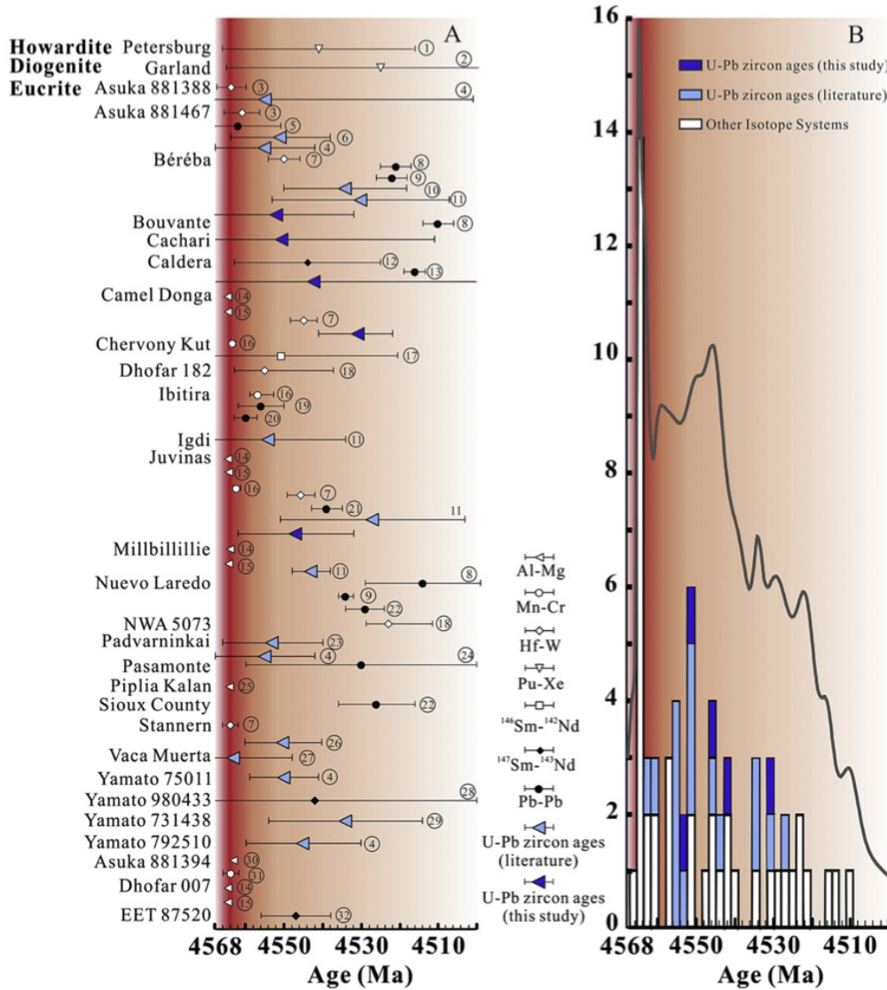
Figure 1.13: Chronology of magmatic activity of the HED parent body from Zhou et al. [2013] and references therein. "The chronological records of the first 50 Ma on Vesta based on radiometric age summary of HED meteorites, including one howardite (Petersburg), one diogenite (Garland) and 28 eucrites. Only high quality data with age uncertainty of less than 50 Ma are included. One of the two zircon grains found in a eucritic clast in Vaca Muerta (mesosiderite) is also included. Shown in dark blue, solid horizontal triangles are U-Pb ages of zircons from this study. Light blue horizontal triangles are U-Pb zircon ages from literature. Open (white) symbols of various shapes are based on short-lived chronometers, whereas solid symbols of various shapes are based on long-lived chronometers. (b) Histogram and the probability density curve of the same age data shown in panel a, showing the intensities and diminishing magmatic activities on Vesta during the first 50 Ma. Red backgrounds symbolize the evolving intensities of magmatic activities on Vesta, as revealed by the available chronological data."
