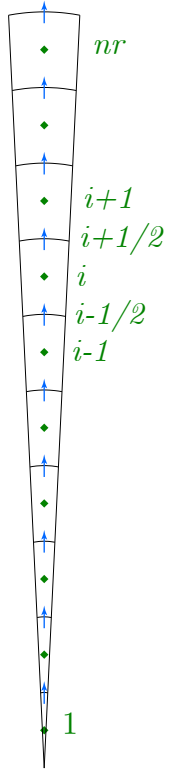
Figure B.4: Volume fractions and temperature meshing.
