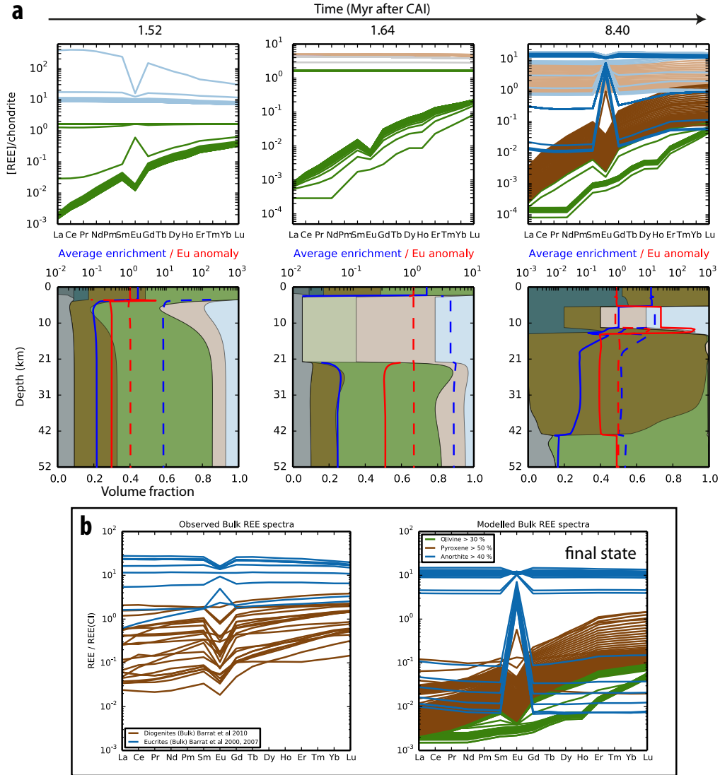
Figure 3.14: a REE enrichments (with respect to CI chondrites) versus time for the reference simulation of Figure 3.8. The REE spectra shown on the first row are colored as a function of the mineralogy of the silicates (basaltic/gabbroic in blue, pyroxenitic in brown and dunitic in green), spectra shown in light colors correspond to the liquid silicates while spectra of the solid silicates are shown in dark colors. The lower row shows the mineralogical profile for the last 52 km, to concentrate on what happens to the basaltic and pyroxenitic part of the "crust". The blue line which is overplotted corresponds to the average REE enrichment of the solid silicates (solid line) and of the liquid (dashed line). Similarly the red solid and dashed lines represent the Eu anomaly in the solid and liquid silicates. For instance, this allows to highlight the important Eu anomaly of the gabbroic rocks that crystallize at the bottom of the final magma ocean (8.4 Myr after CAI). b Comparison between observed REE enrichments measured in basaltic and cumulate eucrites (blue data from [Barrat et al. , 2000, 2007] and diogenites (brown data from [Barrat et al. , 2010]) and the final state of REE enrichments for the reference simulation (right).
