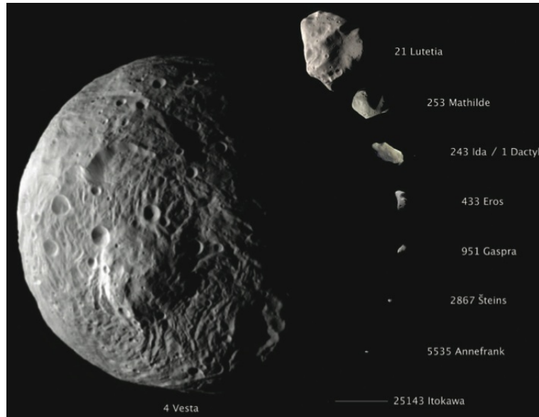
Figure 1.14: "Collage of Vesta in comparison with other asteroids visited to date for which good images exist. This south polar view of Vesta shows the south pole mountain and the Rheasilvia impact basin surrounding this central peak" [Russell et al. , 2012].
