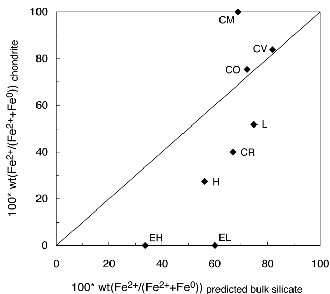
Fig. 9. Comparison of the bulk \text{Fe}^{2+}/(\text{Fe}^{2+} + \text{Fe}^0) ratio required to satisfy the geochemical constraints of a eucrite crust (this work) with values of bulk \text{Fe}^{2+}/(\text{Fe}^{2+} + \text{Fe}^0) for the different bulk chondrite groups as observed today.
