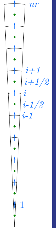
Figure B.1: Velocity mesh.
