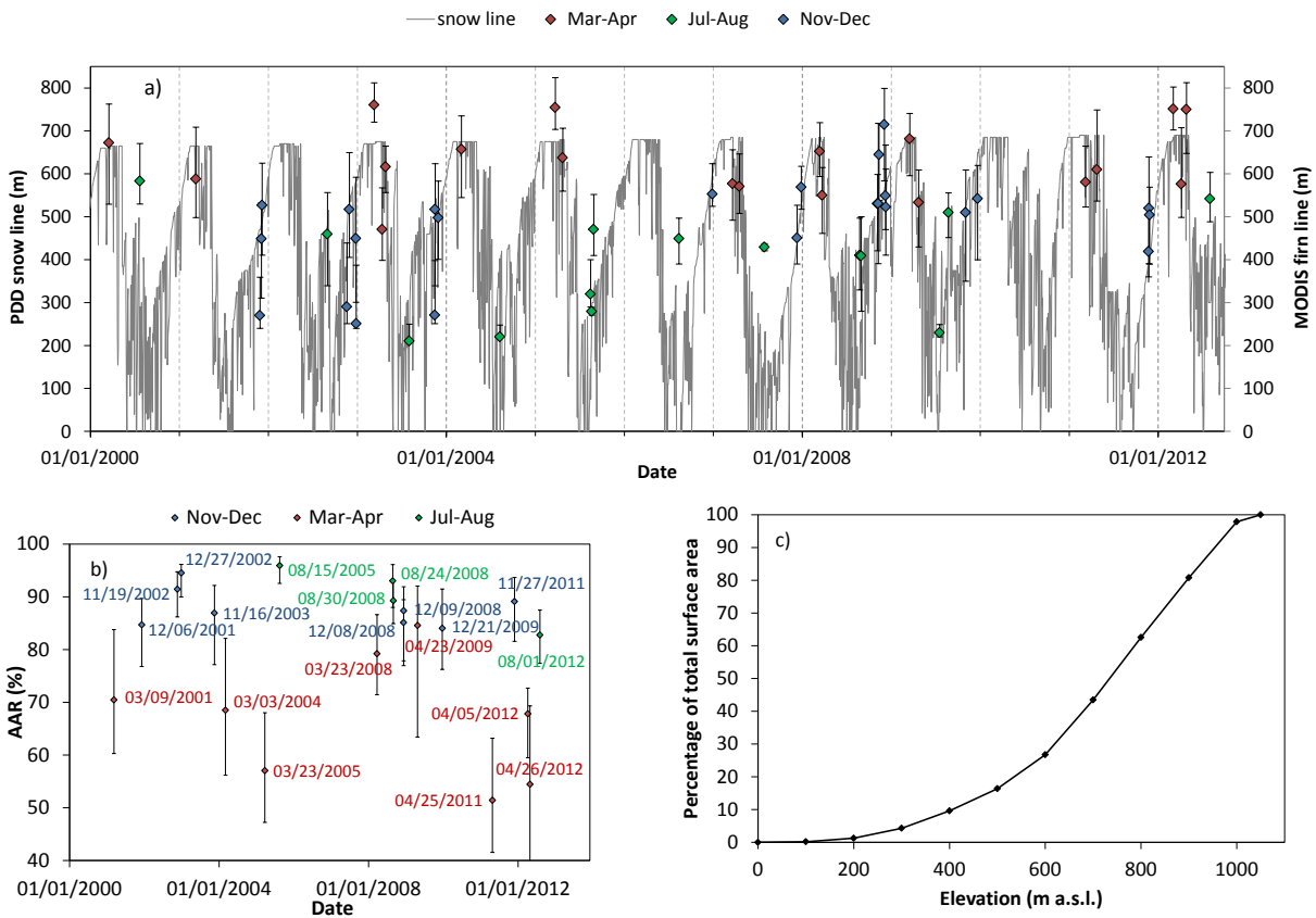
Figure 5. (a) Comparison between Ampere Glacier snow line computed with the PDD model and discrete firm line elevations for the Ampere Glacier obtained from albedo maps derived from MODIS images. Error bars are given for a firm albedo limit between 0.5 and 0.6 on the MODIS images. (b) Changes in the ratio of the accumulation area (firm- and snow-covered area) to the surface area of the entire ice cap between January 2000 and August 2012, for three periods : November-December (blue), March-April (red) and July-August (green) derived from clear-sky MODIS images. Error bars are also indicated for a firm albedo limit between 0.5 and 0.6 on the MODIS images. (c) Hypsometry of the Cook Ice Cap in 2009, i.e. the percentage of the surface area of ice cap below a given elevation.
