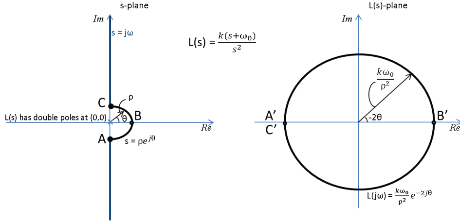
Figure 3.32: Nyquist plot of L(s) = \frac{k(s+\omega_0)}{s^2} for the detour s = \rho e^{j\theta} .
