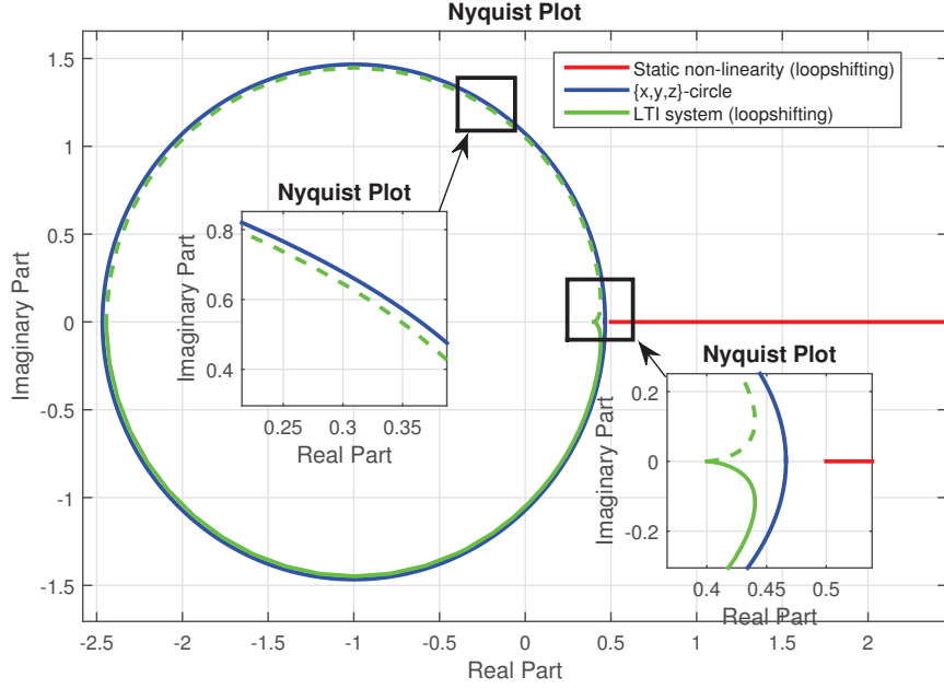
Figure 3.39: Nyquist plot with the circle separation.
