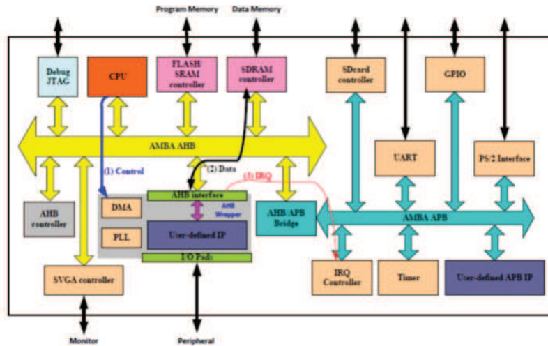
Figure 2.9: System-on-Chip for VENGME validation [Tran13B].
