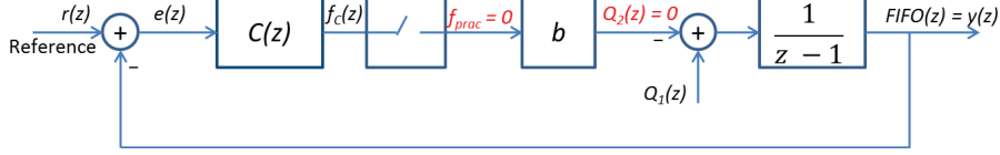
Figure 3.33: Open-loop system when the calculated f_C < 6.25 .
