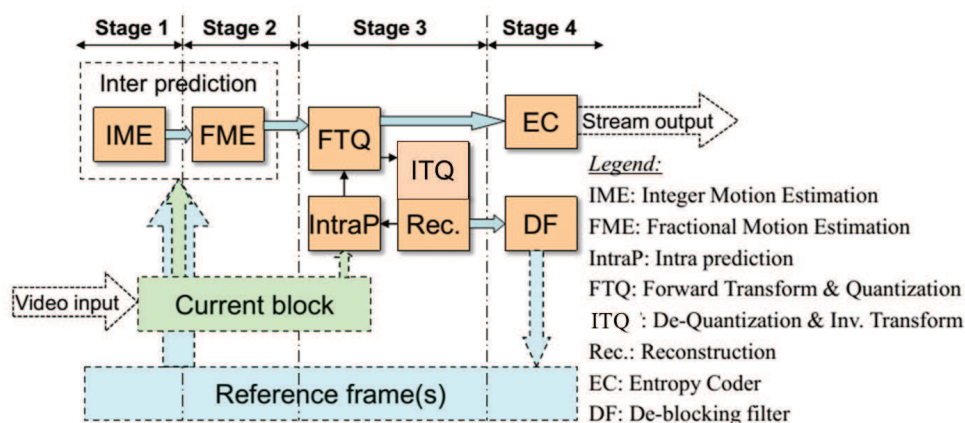
Figure 1.7: A conventional four-stage pipelining architecture for H.264 hardware encoder.
