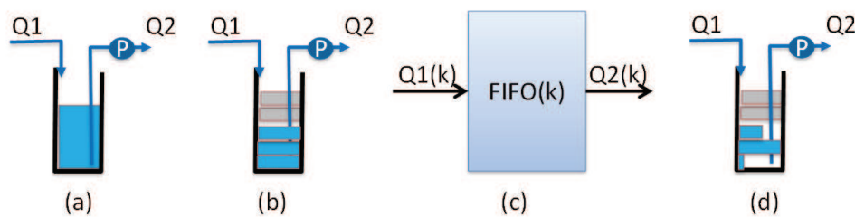
Figure 3.13: FIFO model.
