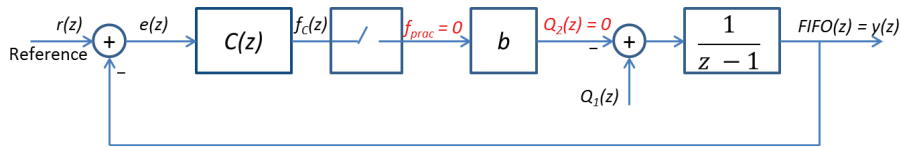
Figure 3.33: Open-loop system when the calculated f_C < 6.25 .
