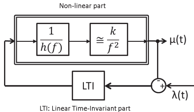
Figure 3.11: Closed-loop system with non-linearities in [Wu05V].
