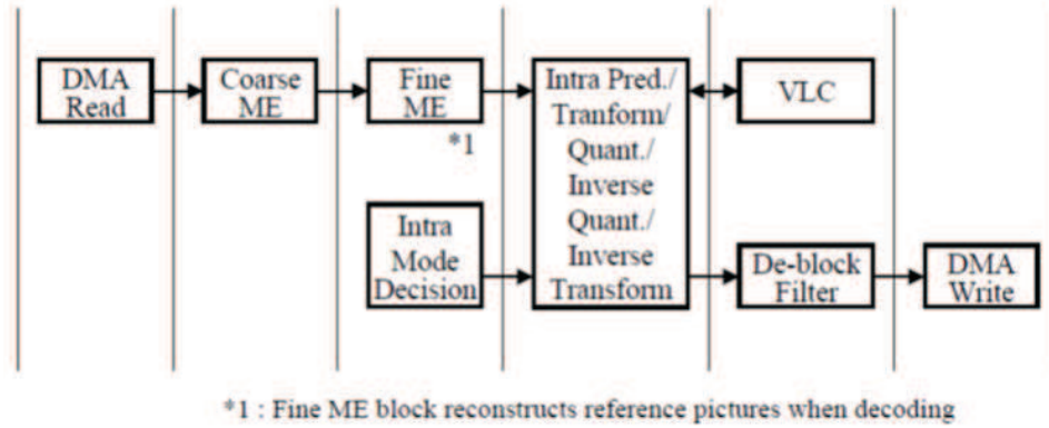
Figure 1.8: An pipelining architecture of H.264/AVC hardware encoder closed to the clasical pipeline [Moch07A].
