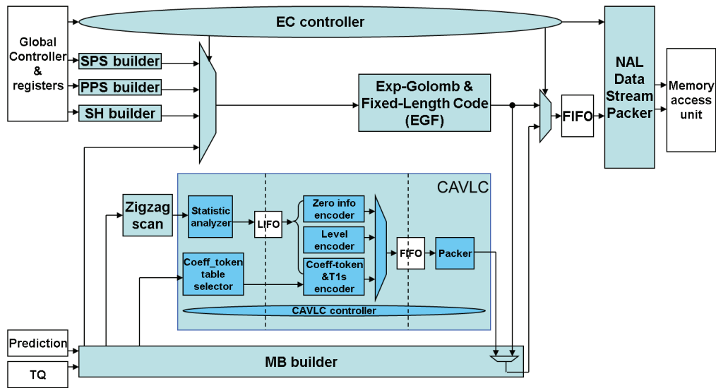
Figure 2.15: Entropy coder and data packer architecture overview.
