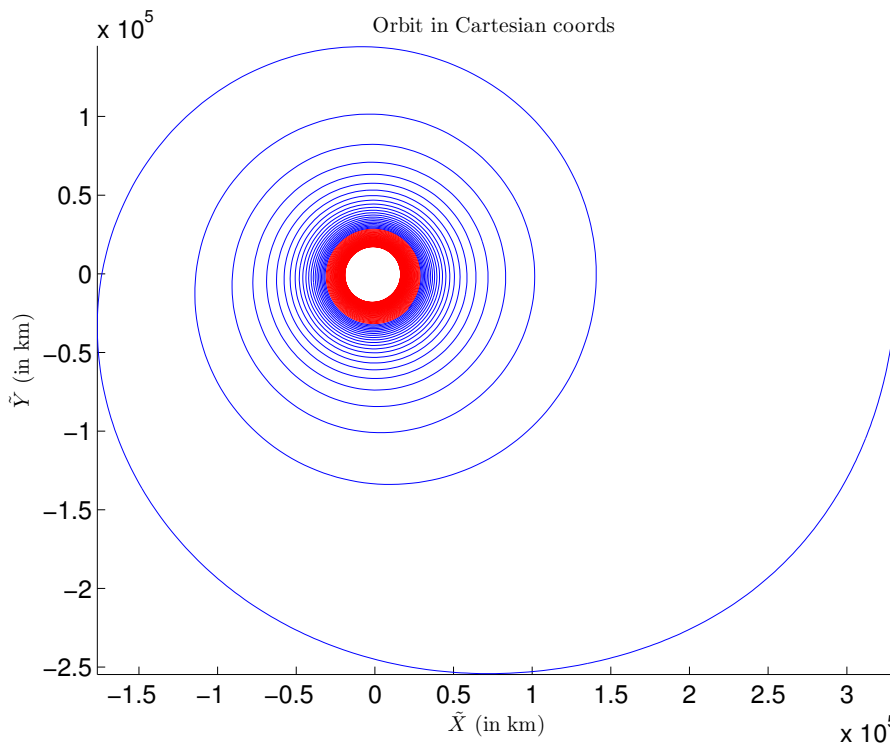
The solution of transfer (5.9) with averaging; orbit in Cartesian coordinates
