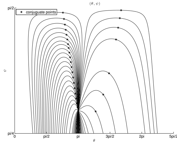
Figure 4.10: Projection of extremal trajectories in the perturbed case ( \lambda = 1 ) in (\psi, \theta) coordinates starting from the same initial point (\rho_0, \theta_0) = (0.60, \pi) . Conjugate points are indicated.
