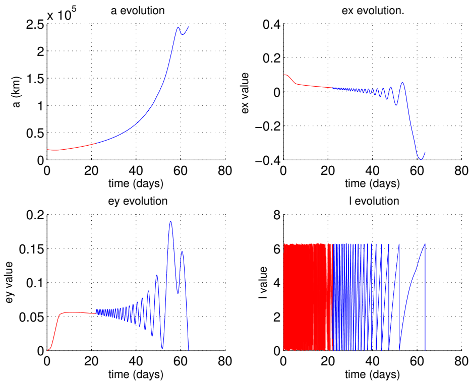
Components (a, e_x, e_y, \ell) of the solution of transfer (5.9) with averaging
