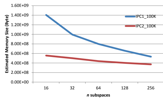
Figure 4.18: ipc100k
