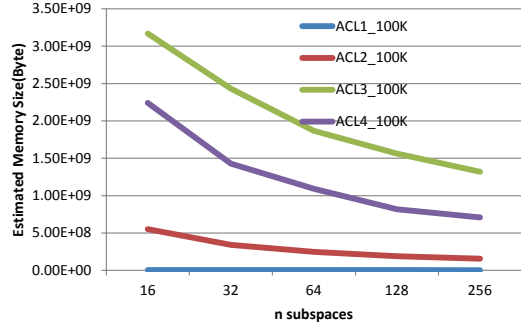
Figure 4.14: acl100k
