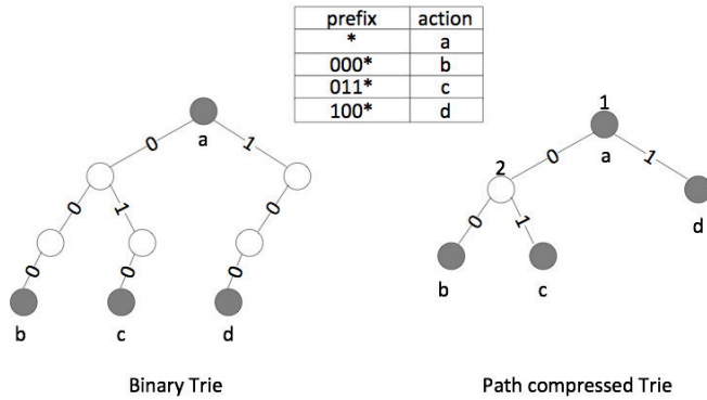
Figure 2.1: Path Compressed Trie
