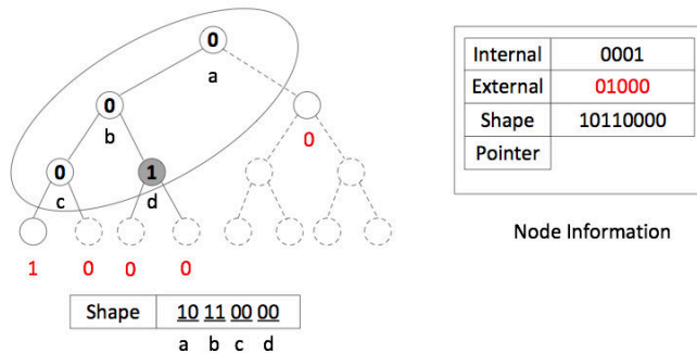
Figure 2.3: The Shape Shifting Encoding Scheme
