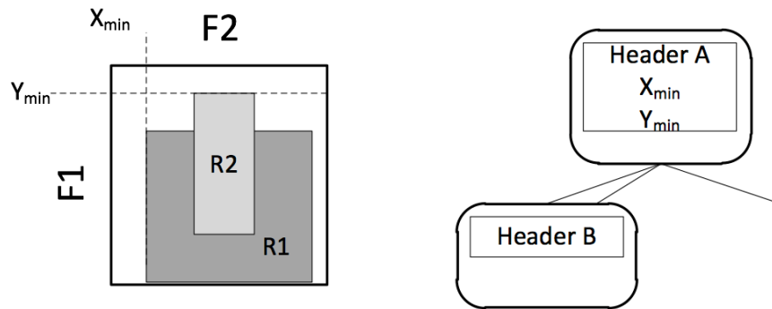
Figure 3.10: Region Compaction
