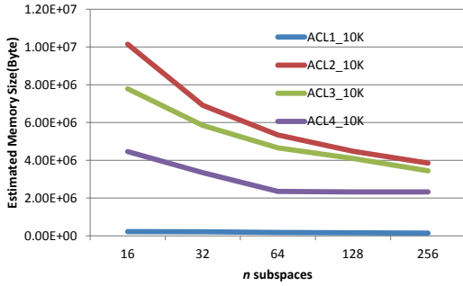
Figure 4.13: acl10k
