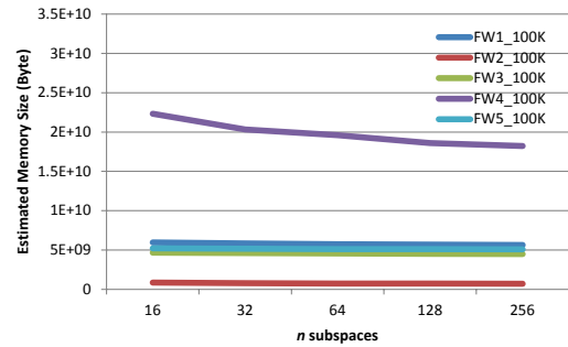
Figure 4.16: fw100k
