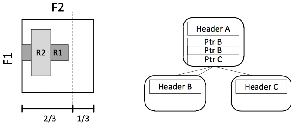
Figure 3.9: Node reuse
