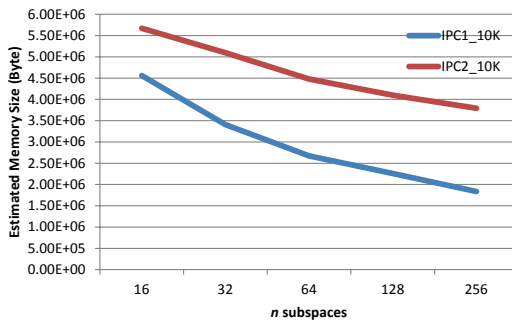
Figure 4.17: ipc10k
