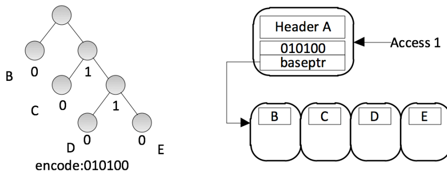
Figure 3.11: Shape encoding
