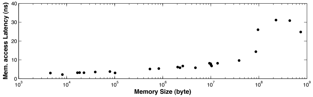
Figure 4.11: Average Memory Access Latency and Memory Size
