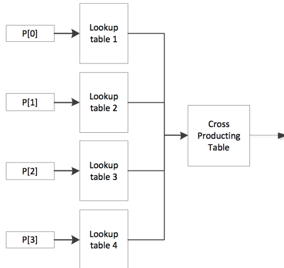
Figure 2.7: the Crossproducing algorithm
