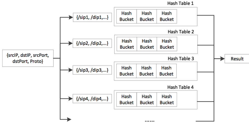
Figure 2.9: The Tuple Space Search algorithm
