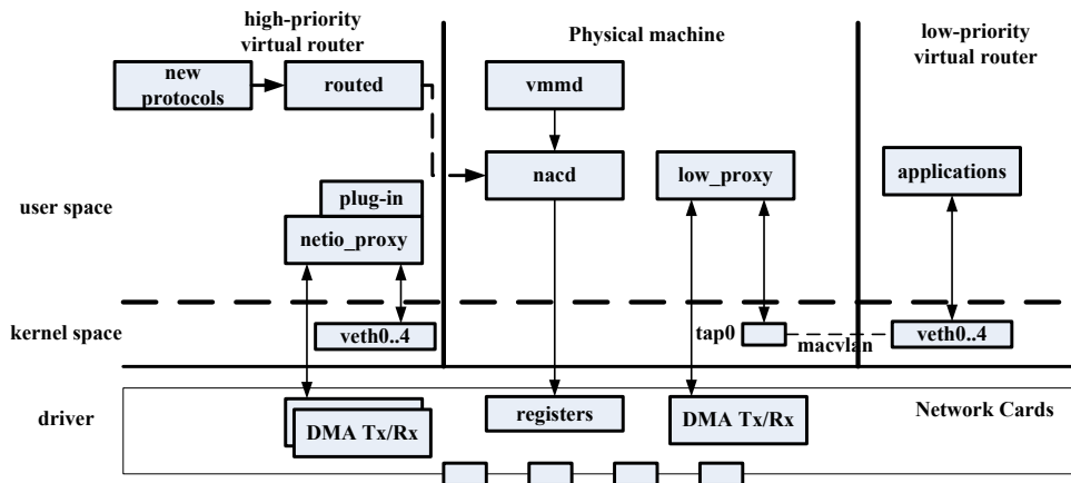
Figure 18- Architecture logicielle de PEARL
