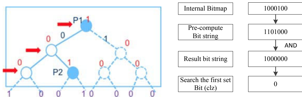
Figure 5.3: Fast internal bitmap checking
