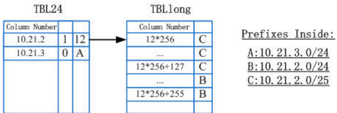
Figure 5.2: The DIR-24-8-BASIC Algorithm
