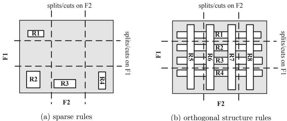
Figure 4.2: Geometric View of Packet Classification Rules
