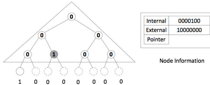
Figure 2.2: Tree Bitmap encoding
