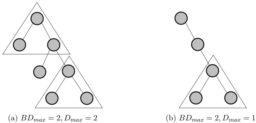
Figure 4.9: the measurement results of two interval trees
