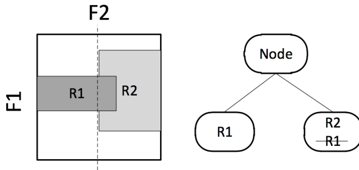
Figure 3.6: Rule Overlap
