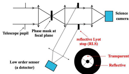
FIG. 1.—Schematic of the Lyot-based low order wavefront sensor (LLOWFS) consisting of a high performance coronagraph combined with a reflective Lyot stop (RLS) with a geometry that can be adapted according to the telescope pupil shape (central obstruction and spider arms) and diffraction pattern created by phase mask at focal plane. See the electronic edition of the PASP for a color version of this figure.
