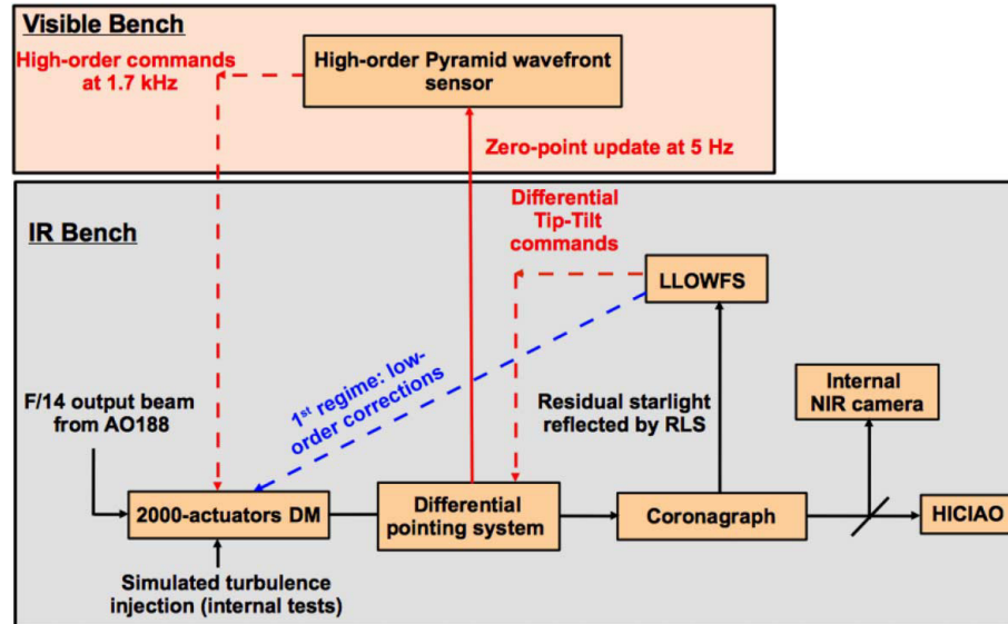
FIG. 13.—Flowchart of the LLOWFS functioning in two configurations on SCEXAO. The black arrows depict the common flow of the low-order control loop in both regimes. Configuration 1 ( blue arrow ) is when the LLOWFS is used directly with the DM to correct for the low-order aberrations as presented in § 3.1. Configuration 2 ( red arrows ) is when LLOWFS, after sensing differential tip-tilt errors in IR channel, updates the zero-point of the PyWFS using a differential pointing system. To compensate for the beam shift in the visible channel, the high-order loop commands the DM to correct for the chromatic errors. See the electronic edition of the PASP for a color version of this figure.
