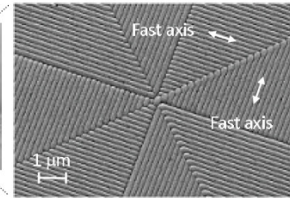
Figure 1: A picture and a scanning electron microscope image of a photonic-crystal coronagraphic mask. (manufactured by the Photonic Lattice, Inc.)
