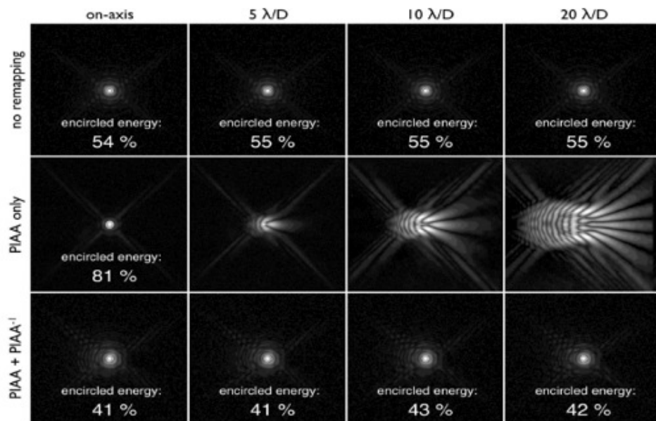
Figure 1.17: Concept of the PIAA coronagraph (Guyon et al. , 2010b; Lozi et al. , 2009). See text for detailed description of the figure.
