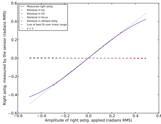
(c) Right astig. measurement
