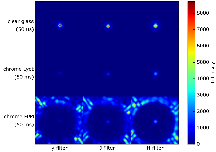
Figure 3.12: The first row of images present PSFs through clear glass of the RLS (exposure time 50\ \mu\text{s} ) in three different bands. The second row shows PSFs through the chrome coated region of the RLS (exposure time 50 ms) and the bottom row is the chrome coated amplitude FPM (§3.4.3). The middle row shows negligible transmission through the chrome layer comparatively to the clear region of the RLS.
