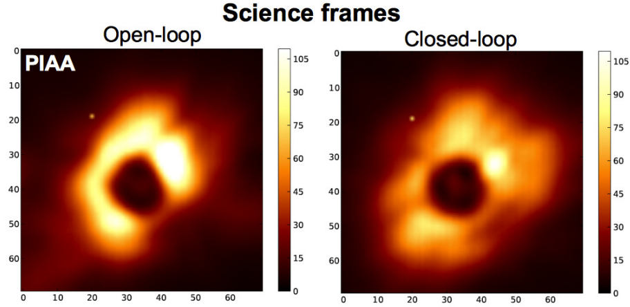
Figure 4.25: On-sky open- and closed-loop processed images of the internal science camera. LLOWFS corrected 5 Zernike modes with PIAA coronagraph in J-band. These images are the standard deviation per pixel of 61 simulated frames of HiCIAO.
