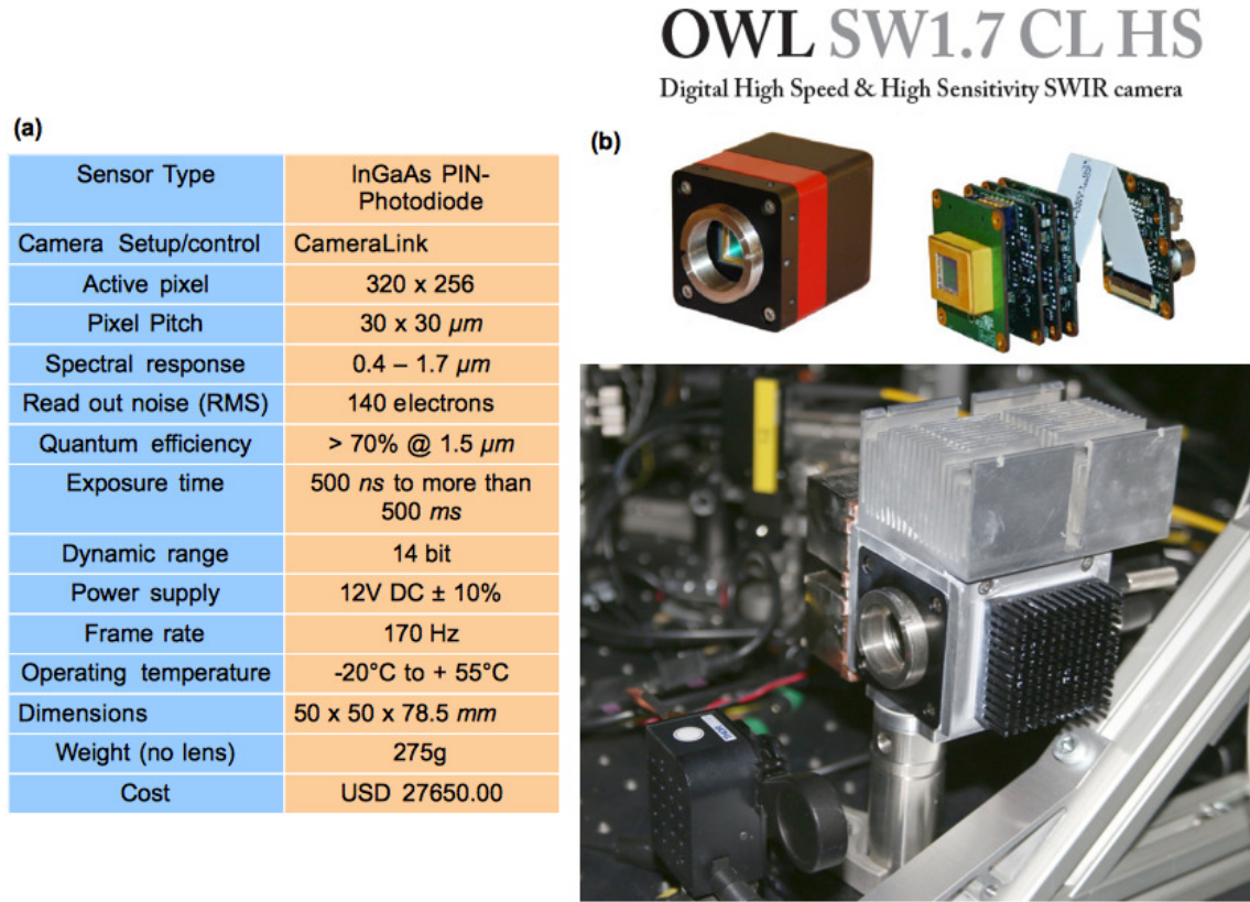
Figure 3.18: Specifications of the LLOWFS camera on SCEXAO instrument.
