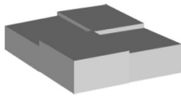
Figure 2: Representation of a FQPM. The \pi phase shift is obtained for wavelengths that verifies (n-1)d = k\lambda/2 where k is an odd integer
