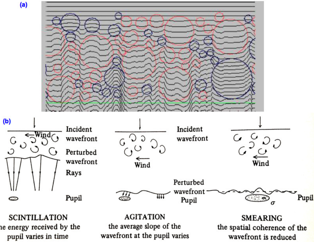
Figure 1.6: Effects of atmospheric turbulence on the images. (a) Incident plane waves when enters the turbulent region of the atmosphere get perturbed. Courtesy of Roddier (2004) (b) Three type of distortions encountered by the wavefront while crossing the turbulent atmosphere ( Lena, 1988 )
