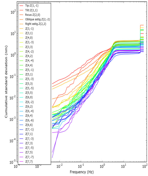
(d) Cumulative standard deviation of 35 modes for EOPM in closed-loop
