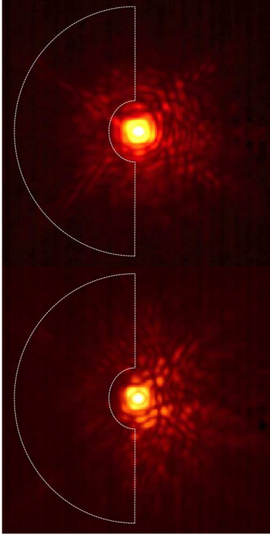
FIG. 7.—Top: RX Boo with no speckle nulling applied. Bottom: RX Boo with speckle nulling performed on the region enclosed by the white dashed line. Each image is a composite of 5000, 50 \mu\text{s} frames which have been shifted and added together. Each panel has a square root stretch applied to it and the maximum and minimum values are clipped for optimum viewing contrast. See the electronic edition of the PASP for a color version of this figure.
