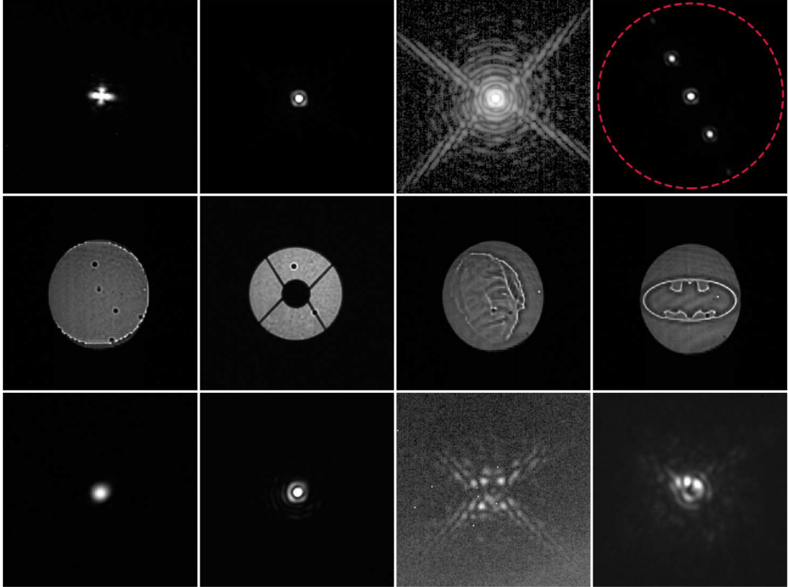
FIG. 5.—Top row: PSF of SCEXAO at 1550 nm with the unpowered DM surface (left). Strong astigmatism is clearly visible. An image of the instrument PSF with the optimum flat map applied with linear (middle-left) and logarithmic (middle-right) scaling. The image is diffraction-limited and numerous Airy rings can be seen. Image with several artificial speckles applied (right). The dashed ring designates the edge of the control region of the DM corresponding to a radius of 22.5\lambda/D or 900 mas at 1550 nm. Second row: Pupil images showing the unmasked surface of the DM with five dead actuators (left), the internal spider mask in place masking several actuators (middle-left), an image of the PI Guyon (middle-right), and the bat symbol (right). These two images demonstrate the resolution of the DM. Bottom row: Image of the PSF taken in the laboratory with a laser at 1550 nm, after the conventional PIAA lenses (left), with the IPIAA lenses (middle-left) as well as with the achromatic focal plane mask (AFPM) ( 1.9\lambda/D IWA) (middle-right). Right: An image with the PIAA, IPIAA, and AFPM is shown taken on-sky on the night of July 25, 2013, with the full H-band. See the electronic edition of the PASP for a color version of this figure.
