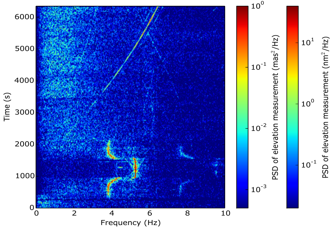
Figure 5.19: On-sky evolution of the closed-loop PSD depicting strong vibrations in Elevation direction. The vibration at 3.8 Hz occurred at pre-/post- transit of the target and its frequency shifted to 5.2 Hz and with 2 times more power during the transit.
