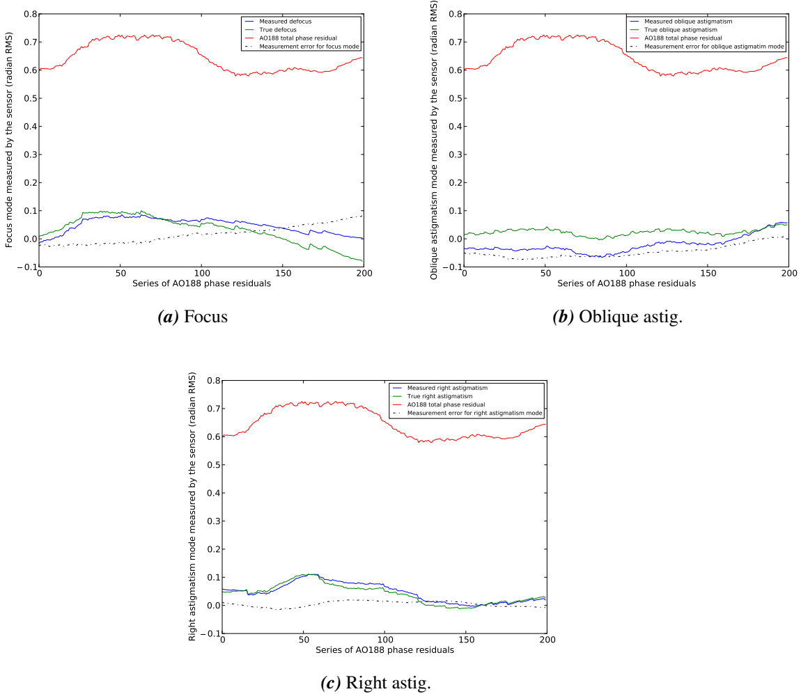
Figure 2.8: Sensor response to (a) Focus, (b) Oblique and (c) Right astigmatisms present in the realistic phase residuals of the Subaru Telescope AO188. The x-axis plots the simulated series of 200 post-AO phasemaps with unknown high- and low-order modes having \approx 180 nm phase rms over the Subaru pupil. The y-axis in (a, b, c) shows the total error in radian RMS (red), the true amplitude of each aberration (green), the corresponding LLOWFS measurements (blue) and the measurement error (dashed line) per mode.
