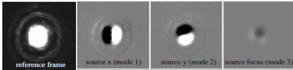
Figure 1.33: (Left to Right) Measured CLOWFS reference image and influence function for the tip, tilt and focus mode. Figure courtesy of Guyon et al. (2009) .
