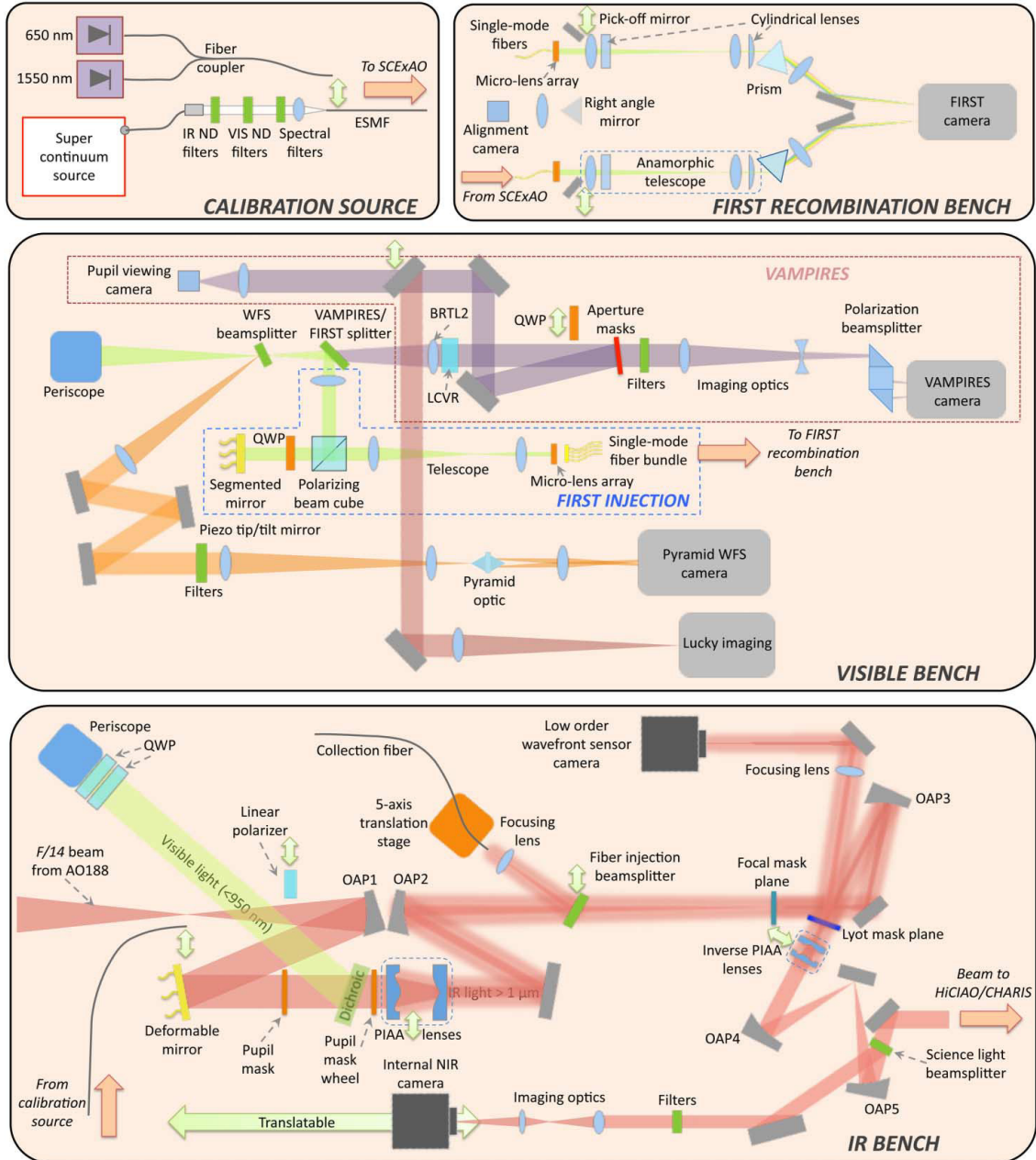
FIG. 3.—Schematic diagram of the SCEAO instrument. Top box (left): Portable calibration source layout. Top box (right): FIRST recombination bench. Middle box: layout of the visible optical bench which is mounted on top of the IR bench. Bottom box: IR bench layout. Dual head green arrows indicate that a given optic can be translated in/out of or along the beam. Orange arrows indicate light entering or leaving the designated bench at that location. See the electronic edition of the PASP for a color version of this figure.
