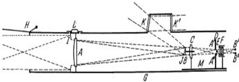
Figure 1.30: Schematic optical diagram of the coronagraph of Bernard Lyot in 1931 (Lyot, 1932) showing a reflective FPM (labelled as “JB”).
