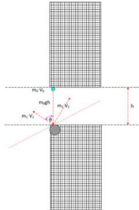
Figure A1- 2: Interval distance determination schema
