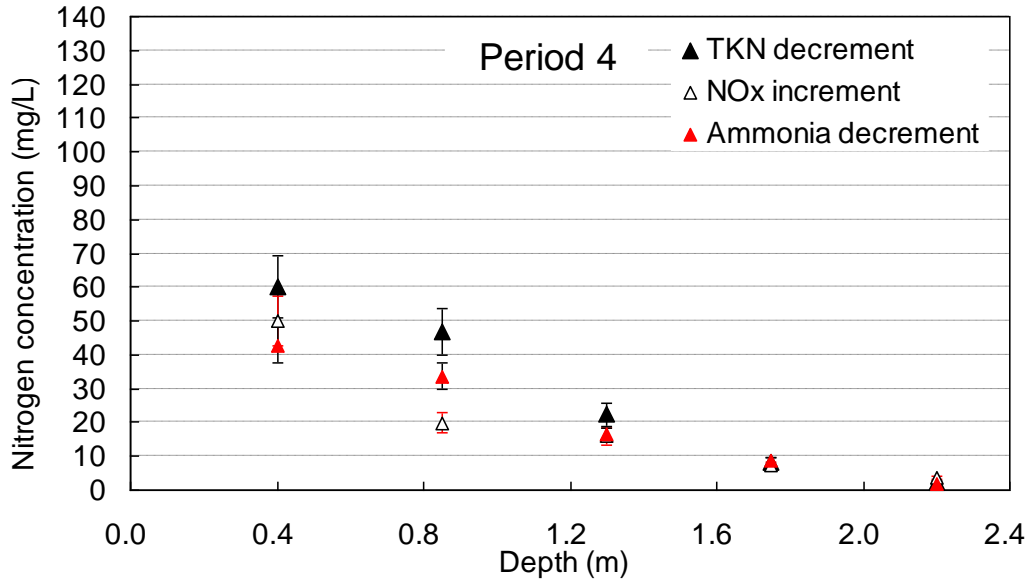
Figure IV- 30: Calculated TKN consumed, nitrate produced and ammonia consumed for each period of time. Period 4, high loading, Viandox
