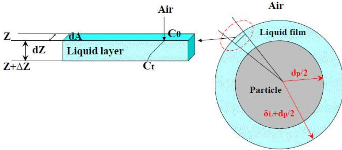
Figure II- 4: Schematic of oxygen transfer
