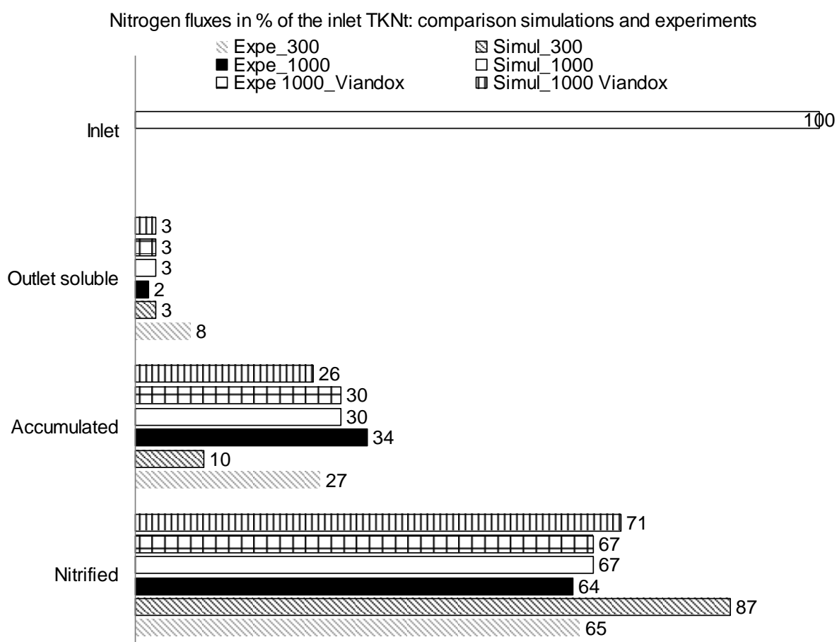
Figure V- 25: General simulation results comparison of ammonia removal and nitrite & nitrate production under various conditions, both simulation and biological experiments
