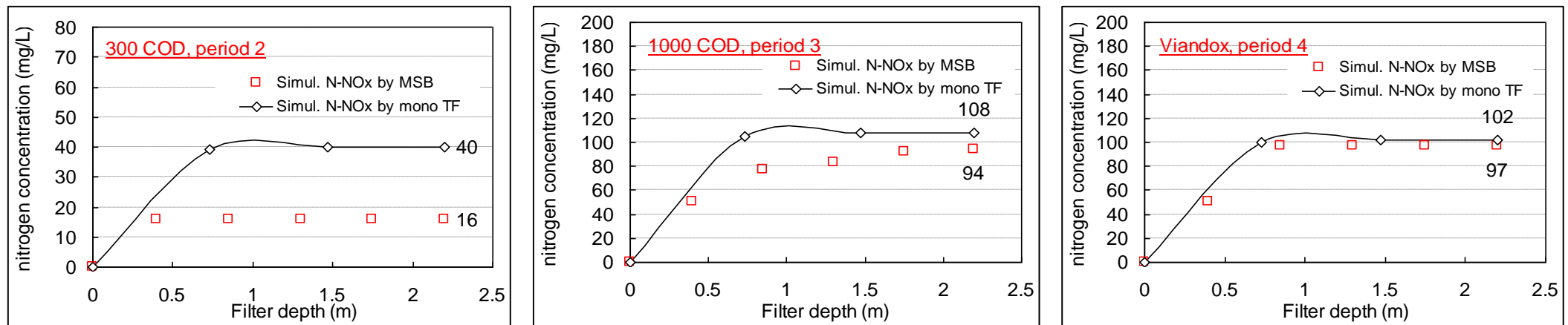
Figure V- 22: Nitrite &amp; nitrate profiles inside the filter, comparison between simulations by MSB and mono TF
