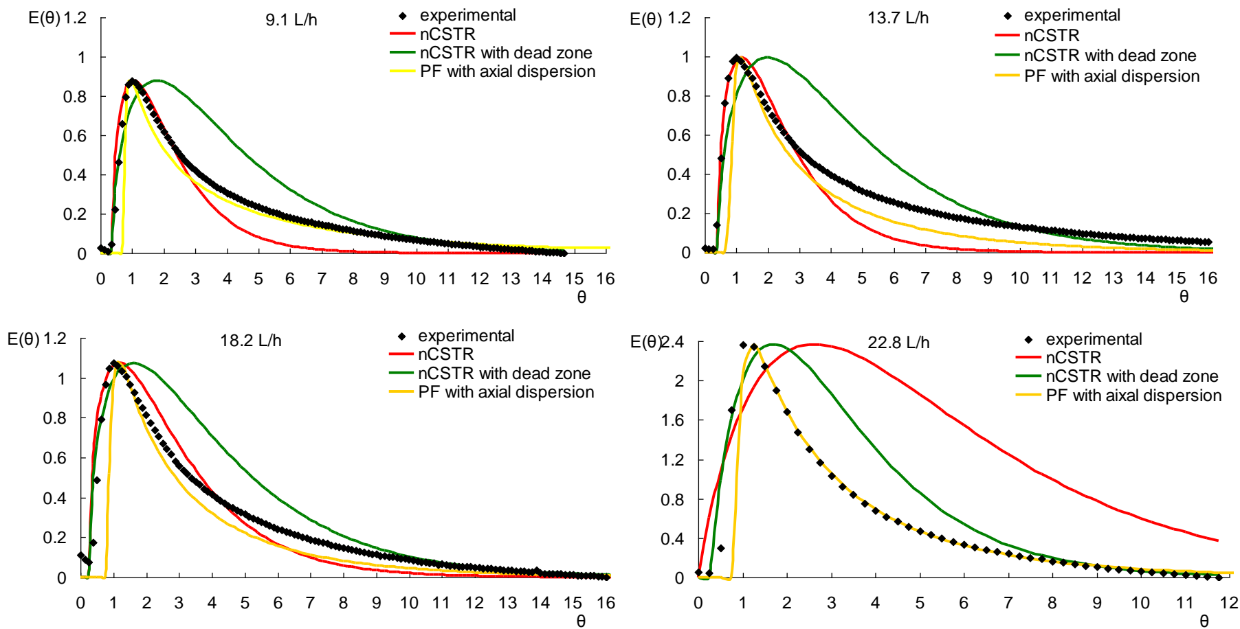
Figure A6-2: Experimental RTD and RTD models in the cases with thick biofilm
