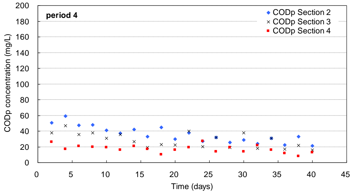
Figure IV- 13: Time-evolution of CODp concentration in section 2-section 4. Period 4, high loading condition, Viandox
