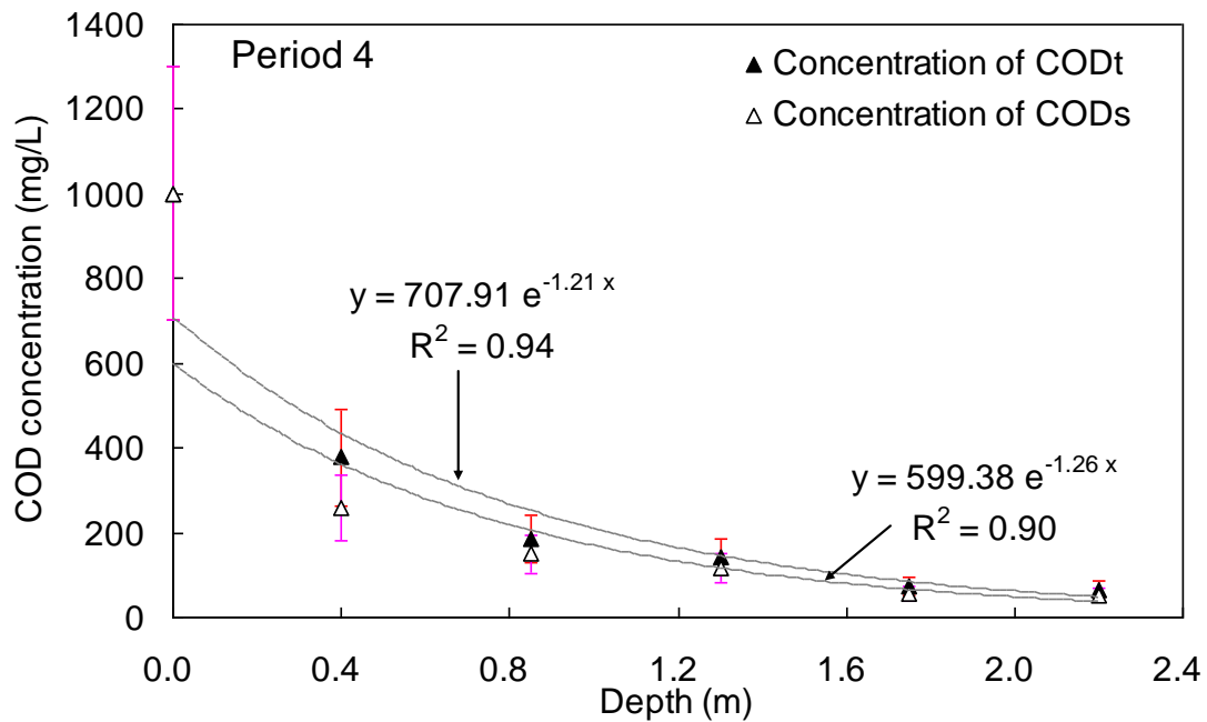
Figure IV- 16: CODt and CODs along the filter. Period 4, high loading condition, Viandox
