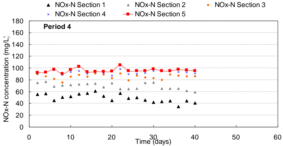
Figure IV- 26: Nitrate and nitrite time-evolution concentration in each section. Period 4, high loading condition, Viandox
