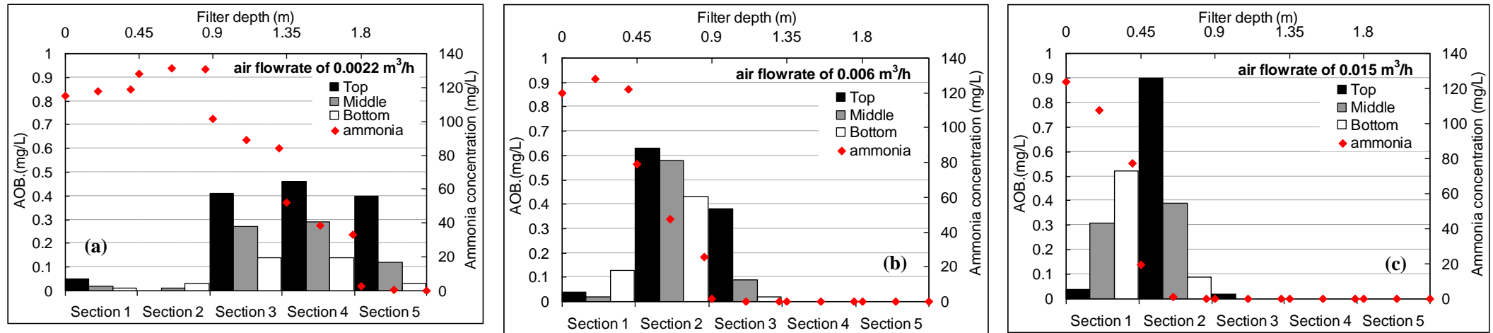
Figure V- 12: Distribution of ammonia and AOB biomass
