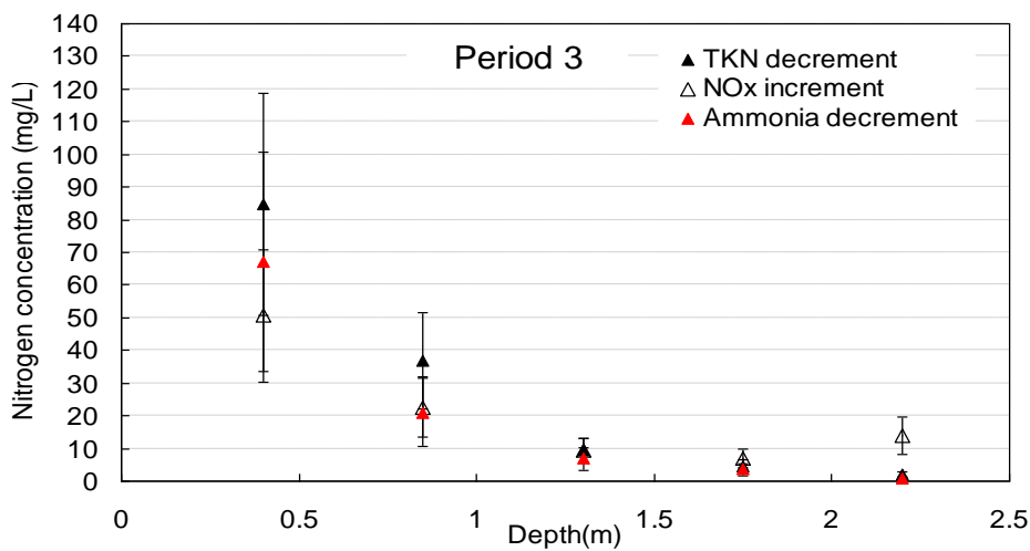
Figure IV- 29: Calculated TKN consumed, nitrate produced and ammonia consumed for each period of time. Period 3, high loading, real WW
