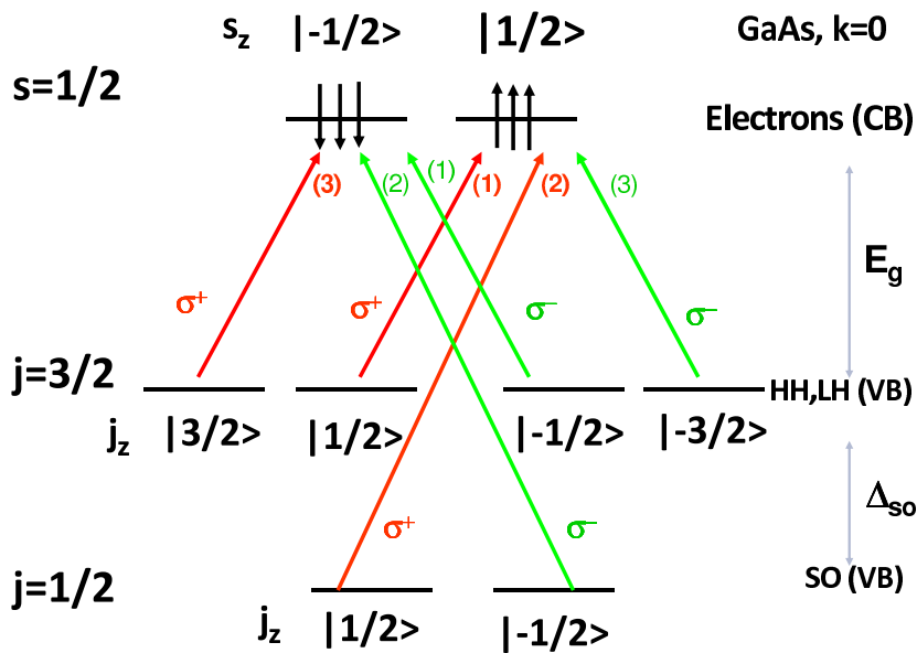
Figure 4.4: Selection rules in the \Gamma valley
