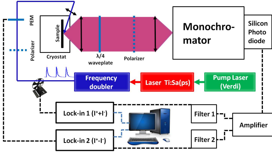
Figure 2.5: Polarized Photoluminescence Excitation Spectroscopy Set-up
