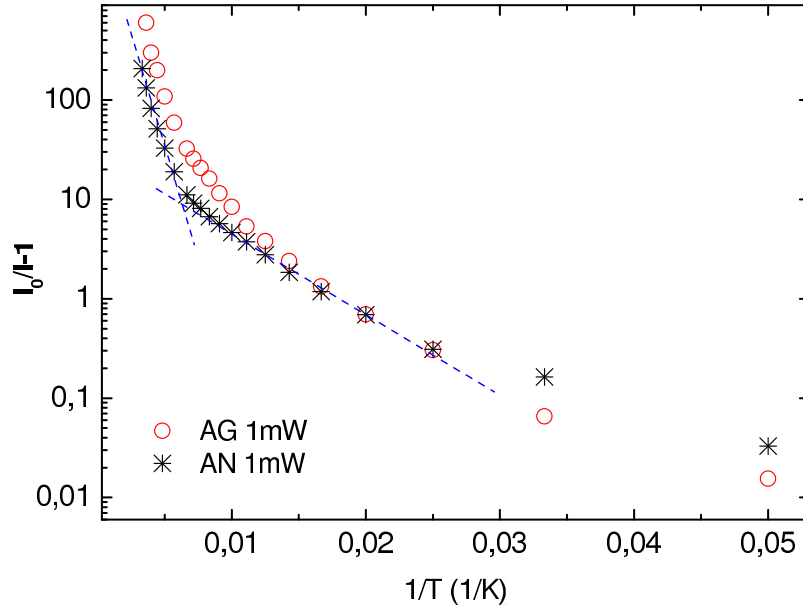
Figure 5.5: Arrhenius plots for the as-grown sample (empty circles) and the annealed (crosses) sample at 1 mW. The dashed lines represent the fitting lines for the calculation of the defects' activation energies in the annealed sample.
