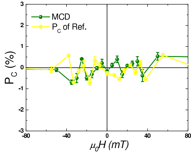
Figure 3.22: MCD measurement from the PMA spin-LED as a function of magnetic field at 25 K. P_C of the EL for a reference sample without CoFeB layer as a function of magnetic field at 25 K.
