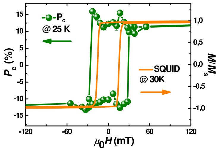
Figure 3.20: P_C as a function of the out-of-plane magnetic field measured at 25 K for a spin-LED with 1.2 nm CoFeB/MgO injectors, which is compared to the corresponding out-of-plane M-H hysteresis loop at 30 K by SQUID in PMA optimized conditions.
