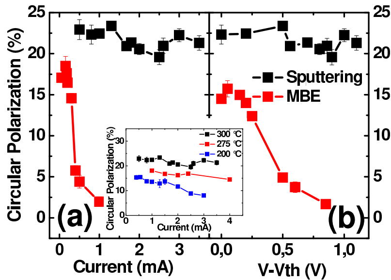
Figure 3.10: (a) Spin-LED with a sputtered and a MBE grown tunnel barrier annealed at 300^{\circ}\text{C} . T=25 K. B=0.8 T : EL Circular polarization as a function of the current. Inset: P_C as a function of the current for sputtered samples at different annealing temperatures. (b) Spin-LED with a sputtered and a MBE grown tunnel barrier annealed at 300^{\circ}\text{C} . T=25 K. B=0.8 T : EL Circular polarization as a function of \Delta V = V - V_{th} .
