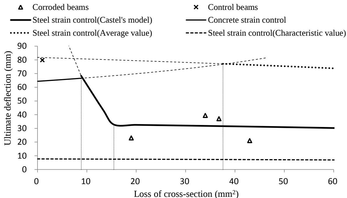
Figure 6-11 Ultimate deflection of the beams
