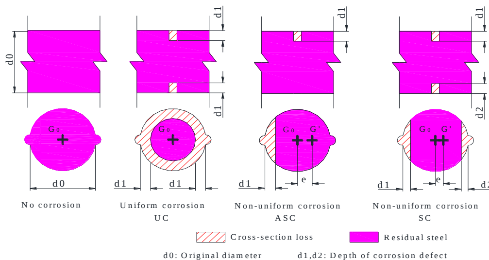
Figure 4-14 Residual cross-section of the corrosion simulations
