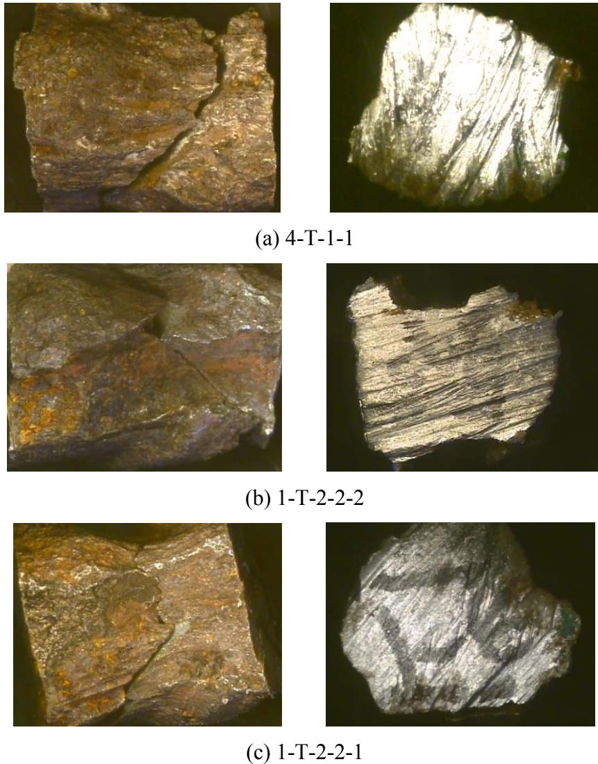
Figure 4-7 Failure points of the corroded bars
