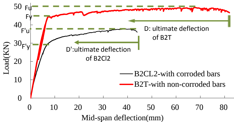
Figure 4-13 Force-deflection curves for the beam
