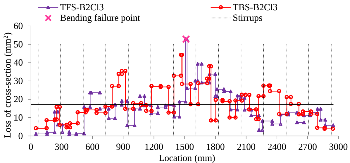
Figure 5-13 Cross-sectional loss of the tension bars of B2Cl3
