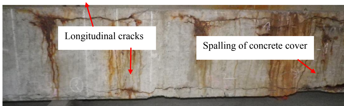
Figure 6-1 Visible damage due to corrosion for beam B2Cl2 at the age of 26 years
