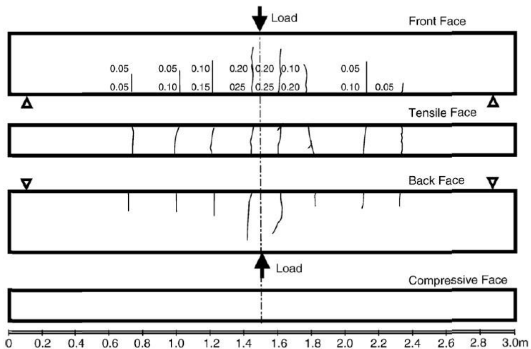
Figure 3-4 Cracking maps of beam B2Cl2 after 28 days of storage[4]
