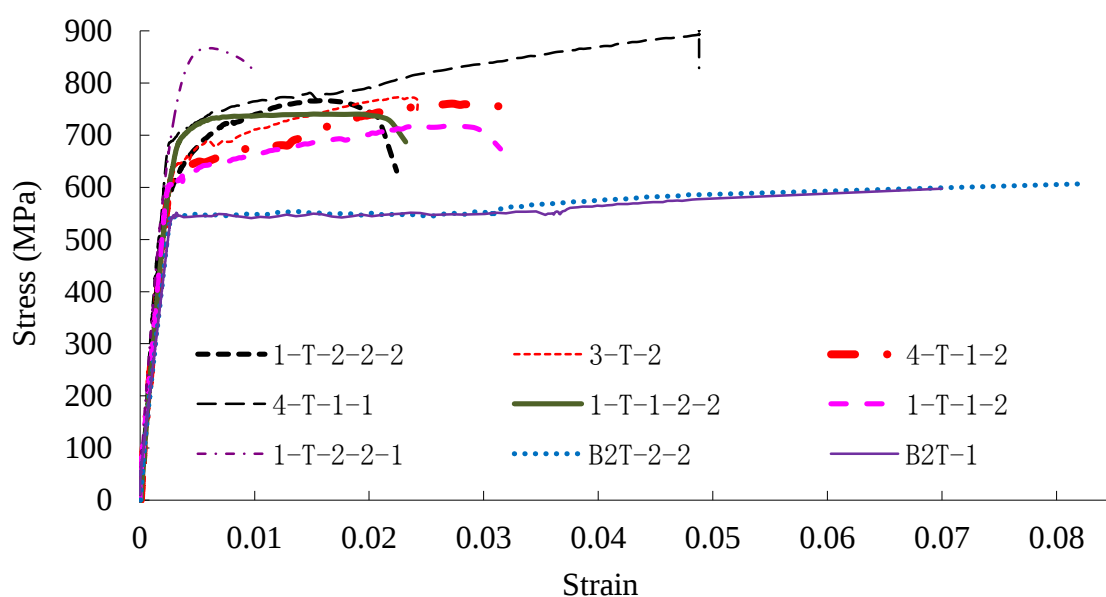
Figure 4-6 Stress-strain curves of the tension tests
