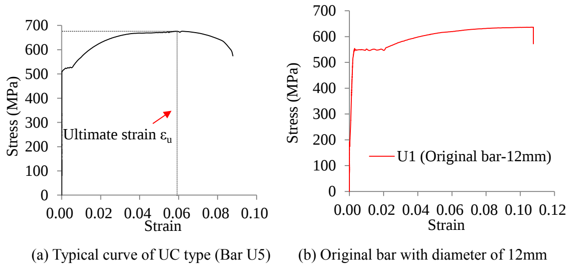
Figure 4-16 Comparison of the stress-strain curves of bars in UC type and original bar
