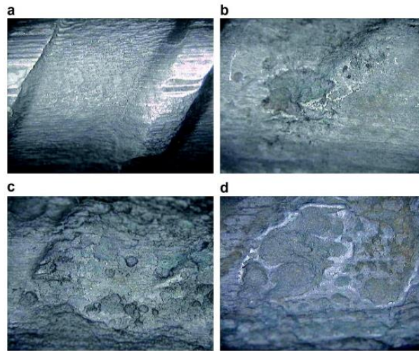
Figure 2-1 Corrosion distribution of the reinforcement[13]
