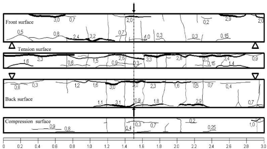
Figure 3-8 Cracking maps of beam B2Cl2 after 23 years of storage[10]
