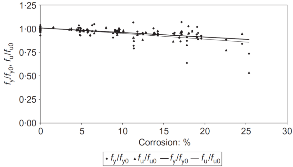
Figure 2-10 Residual strength of corroded bare bars[14]
