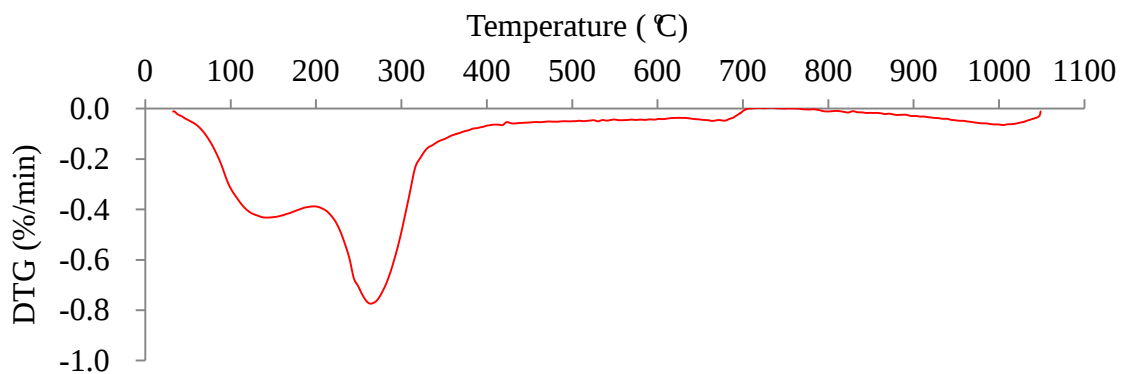
(b) TBS-IV
