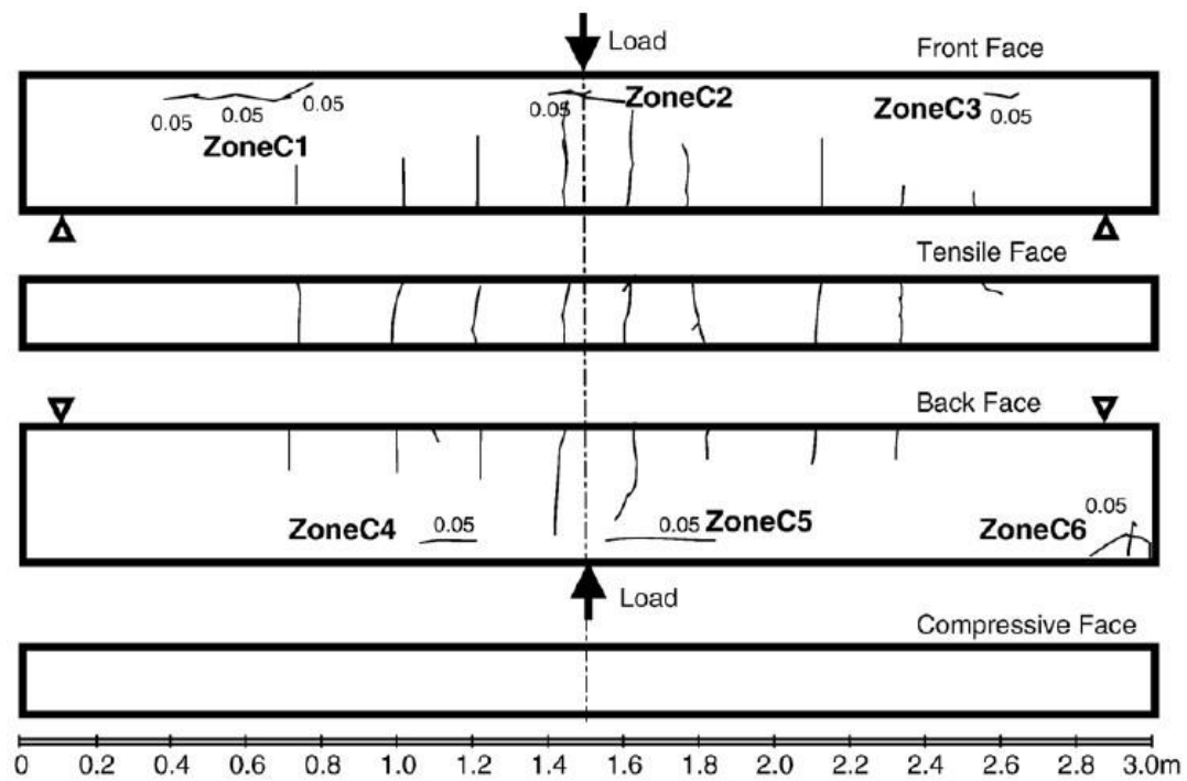
Figure 3-5 Cracking maps of beam B2Cl2 after 6 years of storage[4]
