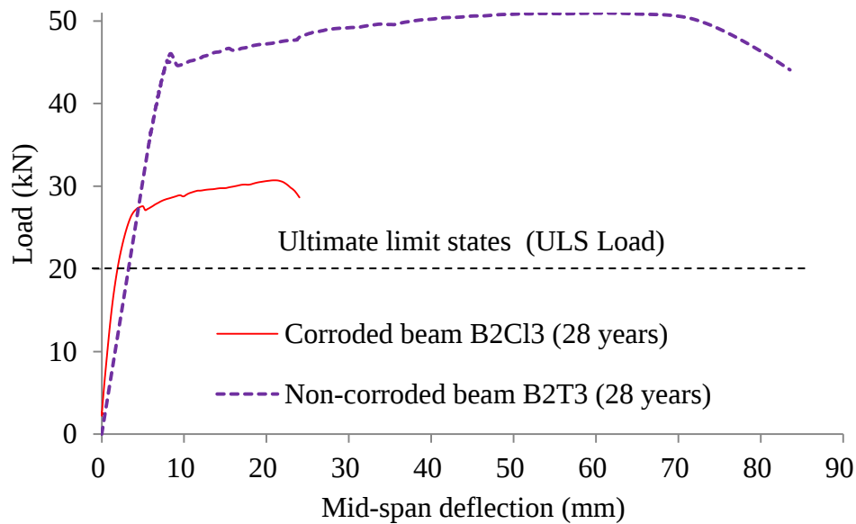
Figure 5-15 Experimental results for the beams B2Cl3 and B2T3 (28 years)
