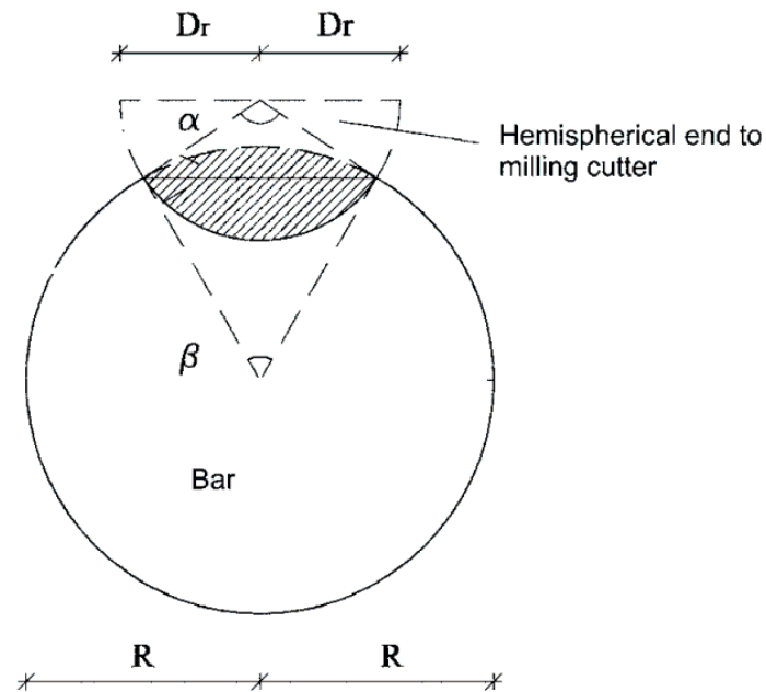
Figure 2-7 Schematic of machined defect geometry[2]
