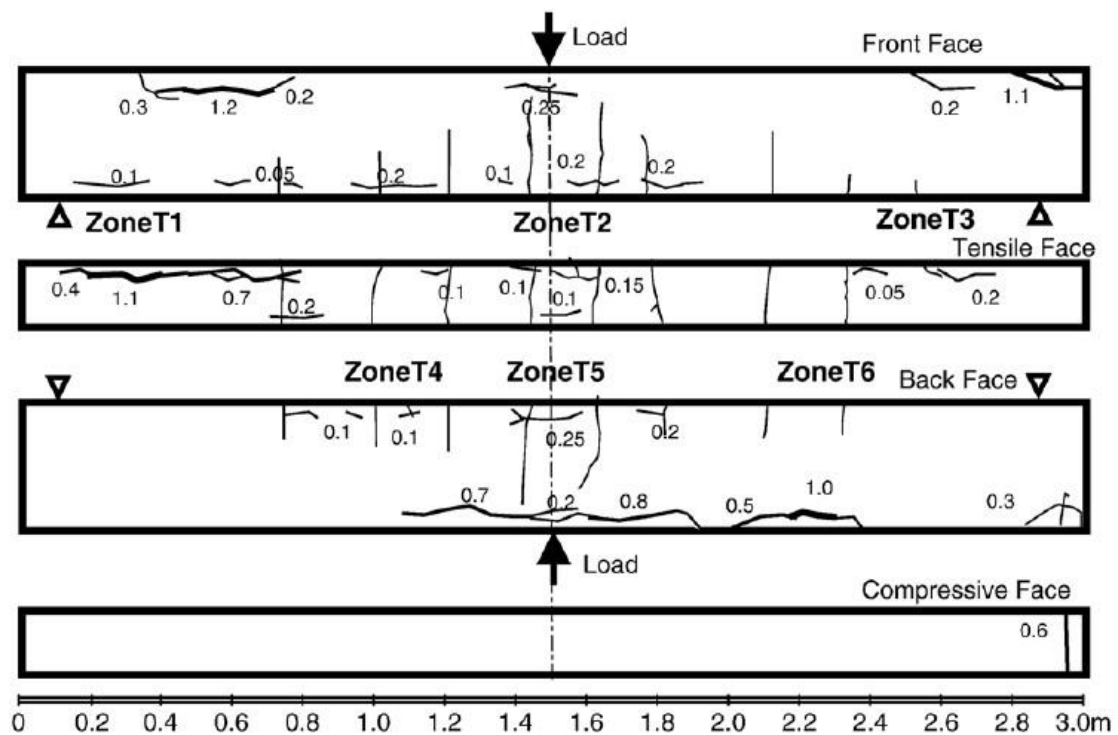
Figure 3-6 Cracking maps of beam B2Cl2 after 14 years of storage[4]
