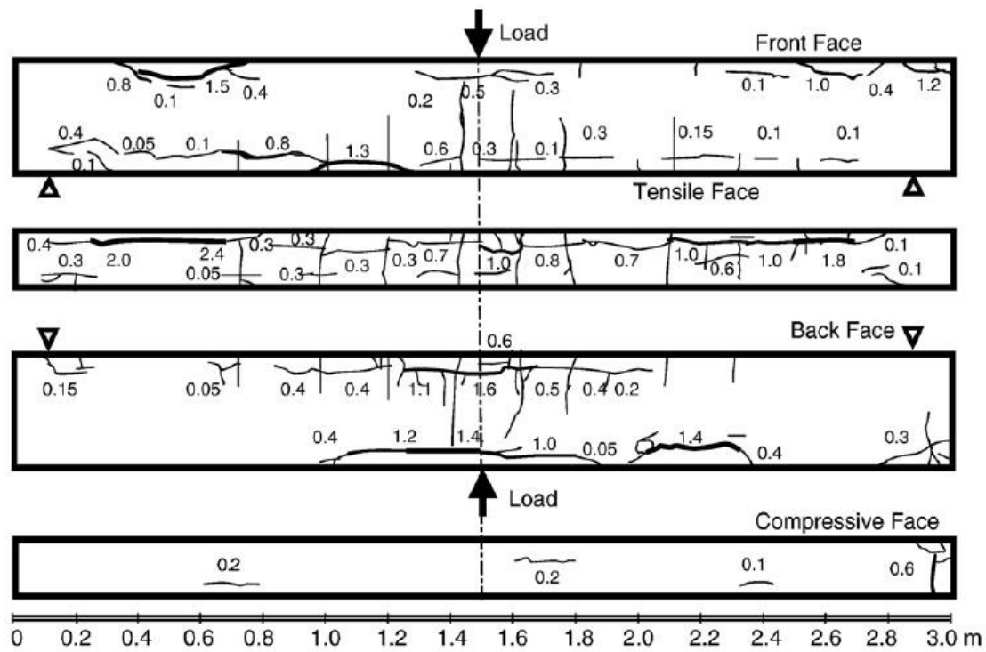
Figure 3-7 Cracking maps of beam B2Cl2 after 17 years of storage[4]
