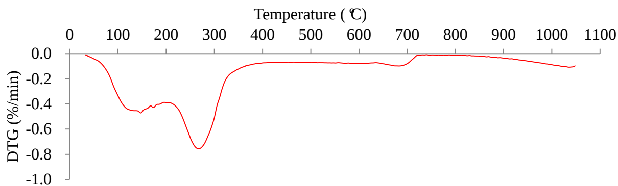
(a) TFS-IV
