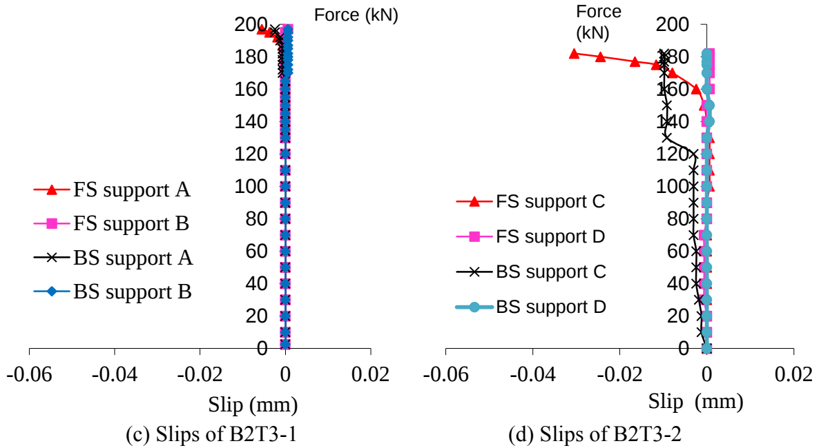
Figure 7-10 Load-slip behaviour for mechanical tests of the non-corroded beams
