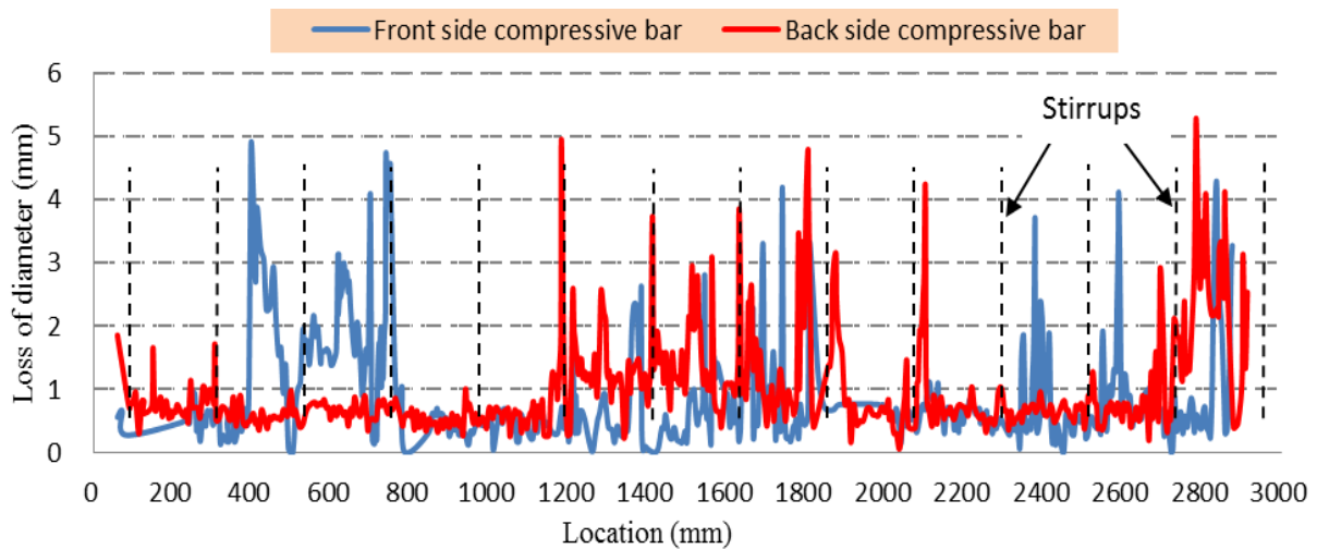
Figure 5-10 Diameter loss of compressive bars by vernier caliper measurement (B2Cl2)
