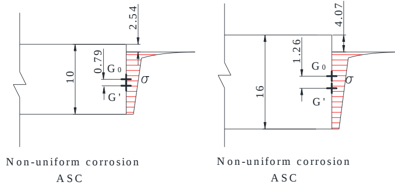
Figure 4-26 Stress distribution of steel bars with different diameters
