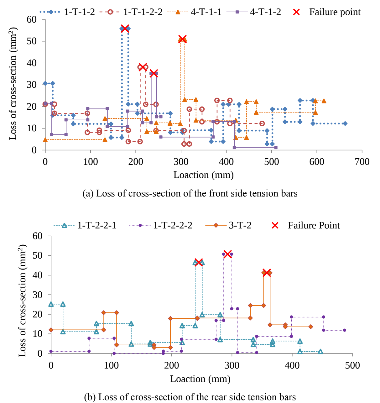
Figure 4-5 Loss of cross-section of the corroded tension bars
