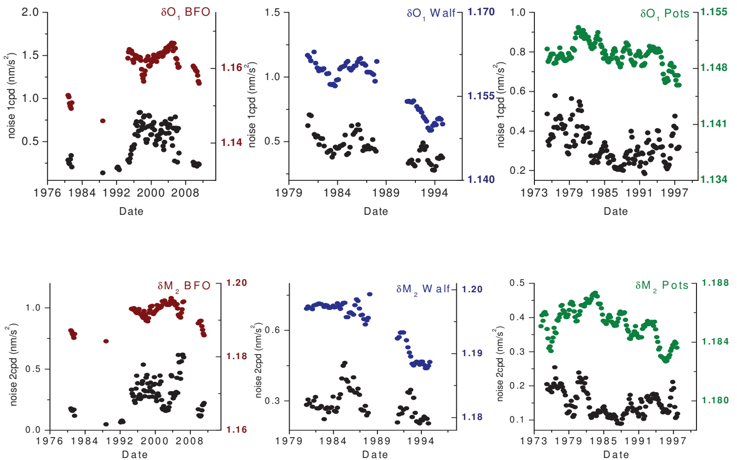
Fig. 4.7: Time evolution of diurnal gravimetric factor ( O_1 ) compared with time evolution of the noise level in the 1 cpd frequency band (upper plots), and of semidiurnal gravimetric factors ( M_2 ) compared with noise level in the 2 cpd
