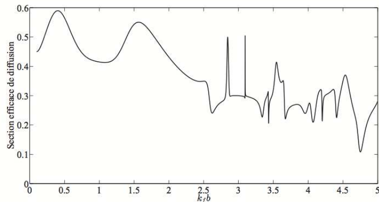
Figure 1.12: Scattering cross section \sigma of a circular ABH (from [5]).
