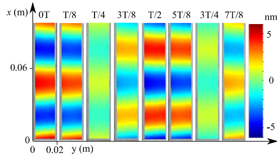
Figure 2.8: Displacement field of the free extremity of an uniform beam at 2330 Hz [45].
