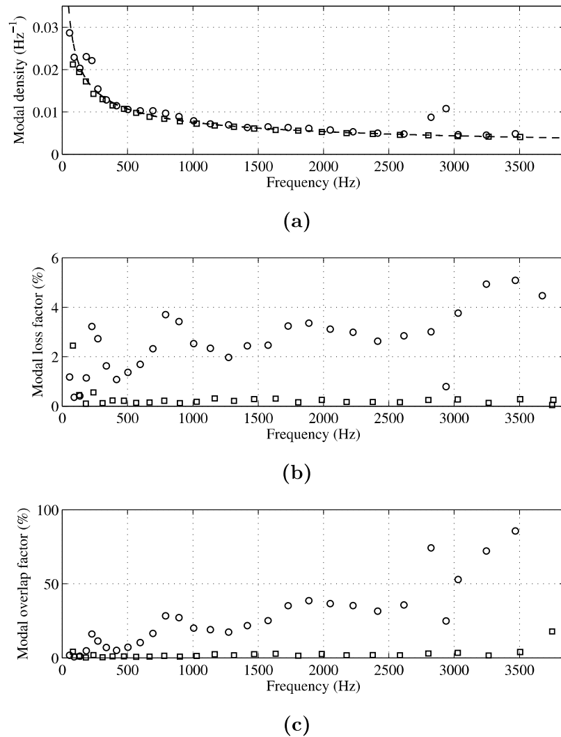
Figure 2.5: Comparison of experimental results between the aluminium reference beam ( \square ) and the aluminium ABH beam ( \circ ): (a) Modal densities n and theoretical prediction for flexural waves in a uniform beam according to Eq. (2.4) (dashed line), (b) modal loss factors \eta , (c) Modal Overlap Factor MOF (published in [38]).
