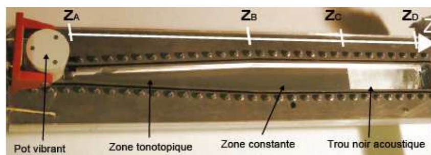
Figure 1.15: Experimental setup showing an artificial cochlea implementing an ABH (indicated as Trou Noir Acoustique , from [52]).
