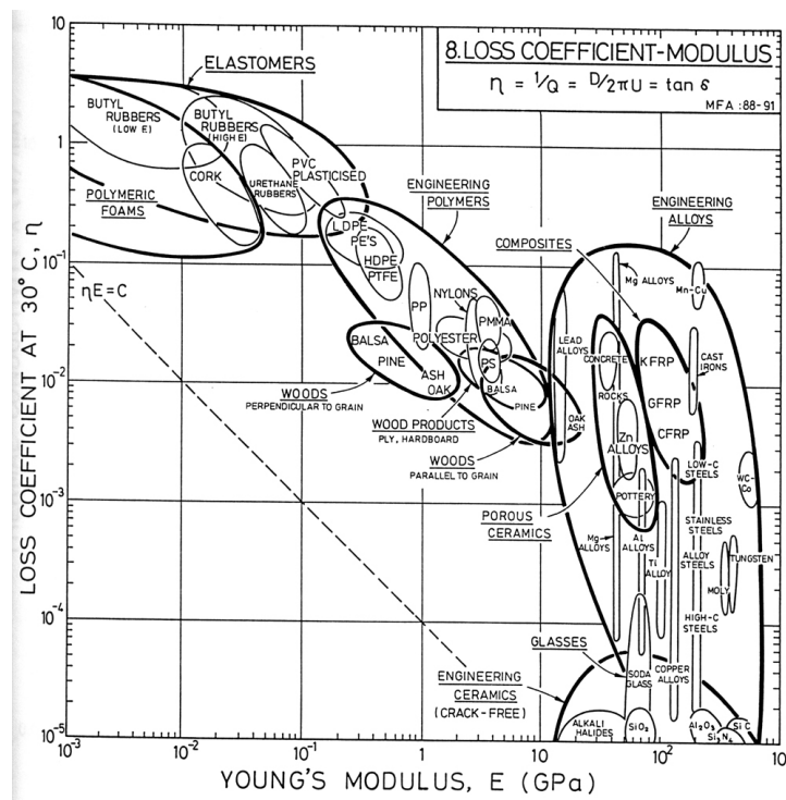
Figure 1.5: Ashby diagram for loss coefficient / Young's modulus (from [8]).
