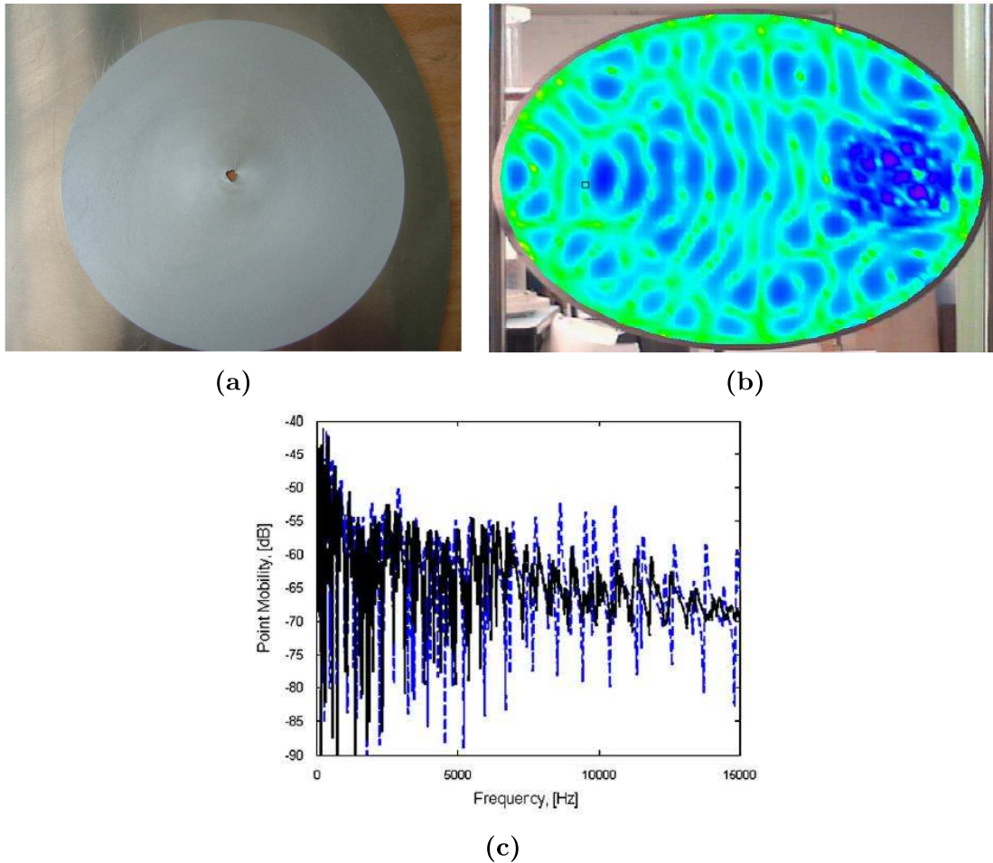
Figure 1.11: (a) Black hole pit presenting a small truncation radius at its centre. (b) Displacement field of an elliptic plate containing a circular ABH in one of the foci. (c) Mobility transfer function of the same plate (from [57]).
