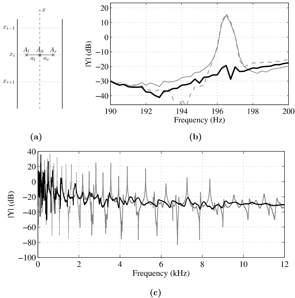
Figure 2.12: (a) Left, centreline and right measurement points A_l , A_0 and A_r at abscissa x_i . (b) Transfer mobility measurement Y(A_l, E) (full grey line), Y(A_r, E) (dashed grey line) and Y(A_0, E) (thick full black line) on the uniform aluminium beam (dB, ref. 1 \text{ m}\cdot\text{s}^{-1}\cdot\text{N}^{-1} ). Force is applied at x_f = 0.58 \text{ m} , velocity is measured at x_i = 0.3 \text{ m} (see Fig. 2.11) (c) Transfer mobility measurement Y(A_0, E) for uniform (grey line) and ABH (black line) beams made of aluminium (dB, ref. 1 \text{ m}\cdot\text{s}^{-1}\cdot\text{N}^{-1} ). Force is applied at x_f = 0.58 \text{ m} , velocity is measured at x_i = 0.3 \text{ m} .
