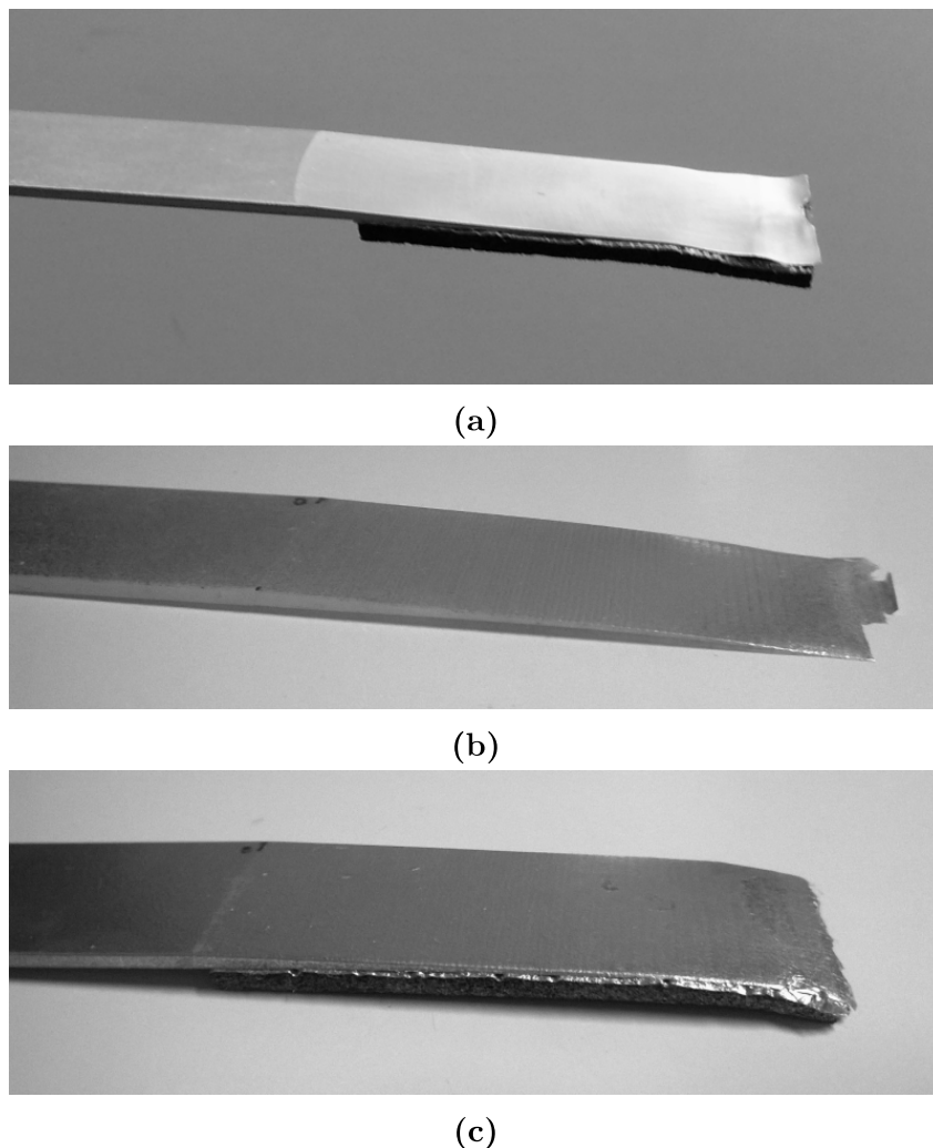
Figure 2.2: Pictures of ABH extremities (a) made of aluminium and covered, (b) made of polymer and non covered and (c) made of polymer and covered.
