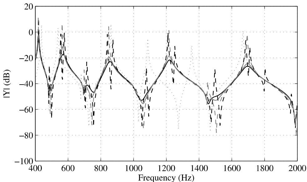
Figure 4.17: Mobility transfer function of homogeneous plate (dotted), ABH plate (dashed grey), ABH plate with damping layer (full grey), imperfect ABH plate (dashed black) and imperfect ABH plate with damping layer (full black).
