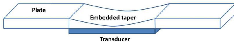
Figure 1.16: Plate embedding an ABH and a surface-mounted transducer (from [138]).
