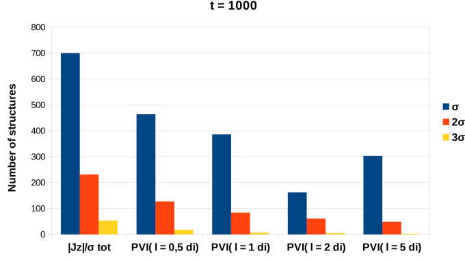
Figure 22: The total number of structures with |J_z|/\sigma and PVI value higher than \sigma is represented with blue histograms, higher than 2\sigma with red histograms and higher than 3\sigma with yellow histograms. Four different scales are considered for PVI \ell = 0.5 d_i, 1 d_i, 2 d_i, 5 d_i .
