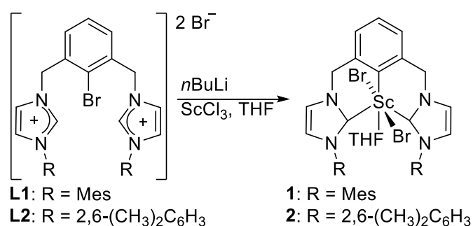
Scheme 1. Sc(III) complexes bearing chelating bis-NHC ligands. 3-4
