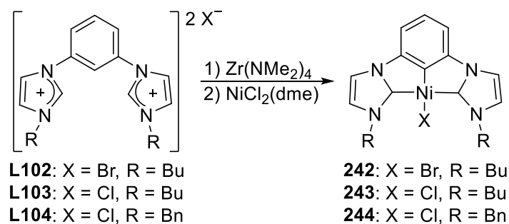
Scheme 62. Pincer Ni(II) complexes. 89
