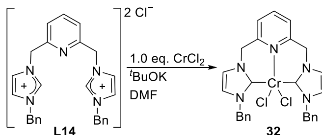
Scheme 12. Cr(II) bis-NHC pincer complex. 17
