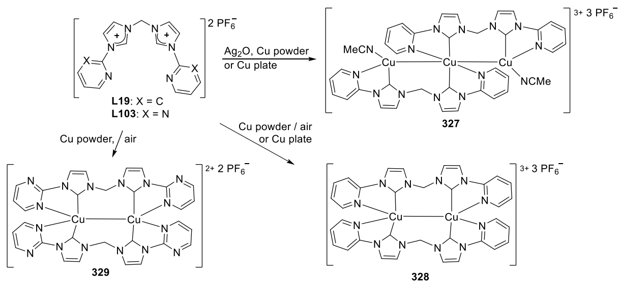
Scheme 104. Di- and tri-NHC Cu(I) complexes. 29,38,68
