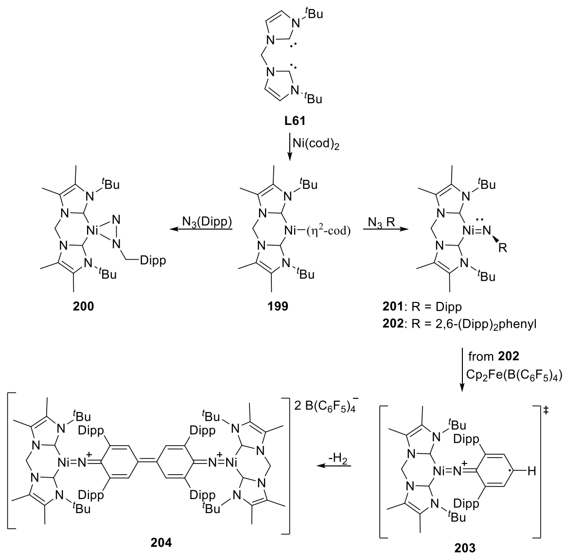
Scheme 48. Synthesis and reactivity of arylimido Ni(II) complexes. 72
