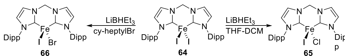
Scheme 23. Fe complexes bearing chelating bis-NHC ligands. 34
