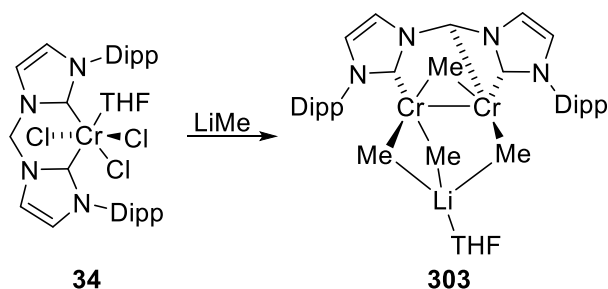
Scheme 87. Trinuclear lithium-chromium bis-NHC complex. 18
