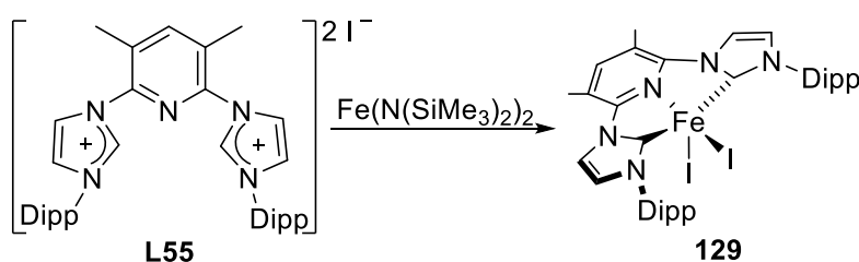
Scheme 38. Fe(II) (bis-NHC)-pyridine complex. 46
