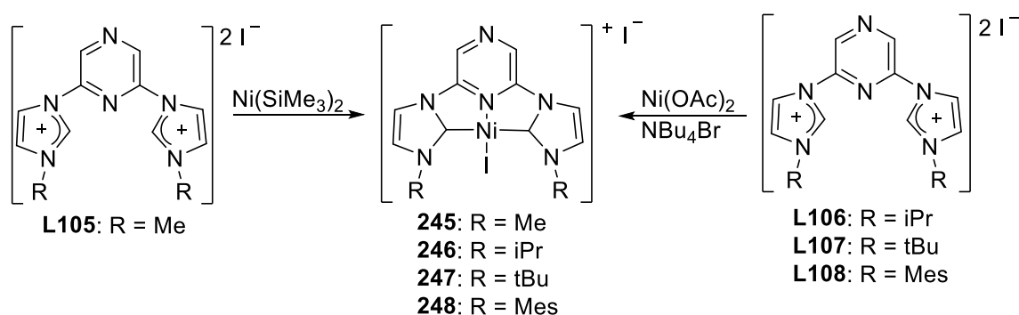
Scheme 63. Pincer bis-NHC Ni(II) complexes. 90
