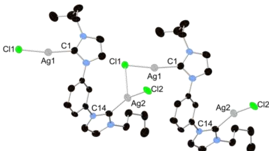
Figure S2. ORTEP of the molecular structure of 336 . Ellipsoids set at 30 % probability level. Hydrogen atoms have been omitted for clarity.
