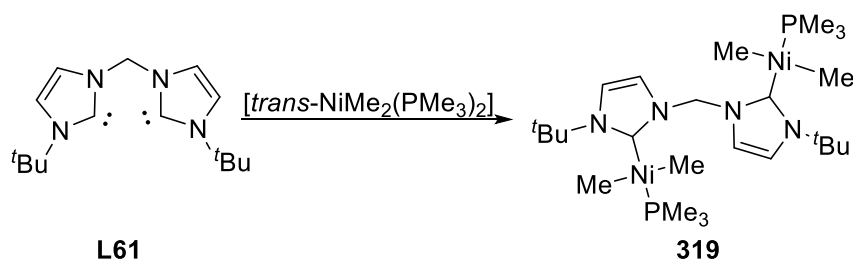
Scheme 97. Bis-NHC methyl Ni(II) complex. 22c
