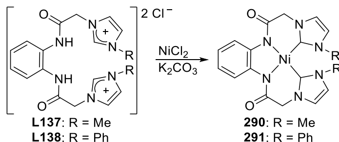
Scheme 81. Bis-NHC amido Ni(II) complex. 104
