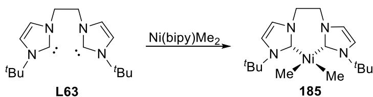
Scheme 42. Methyl Ni(II) complex. 22c
