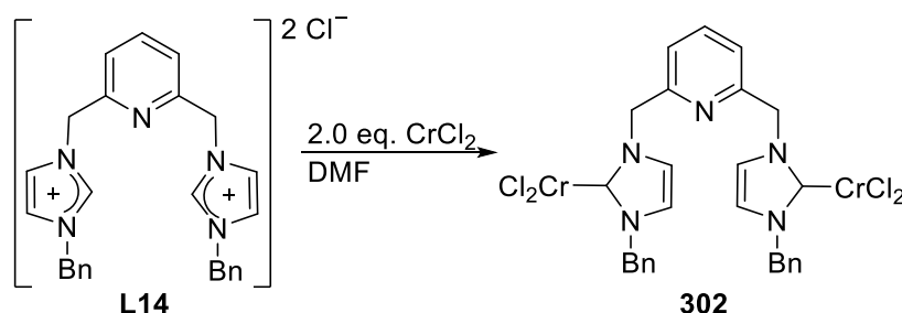
Scheme 86. Bridging bis-NHC Cr(II) complex. 17
