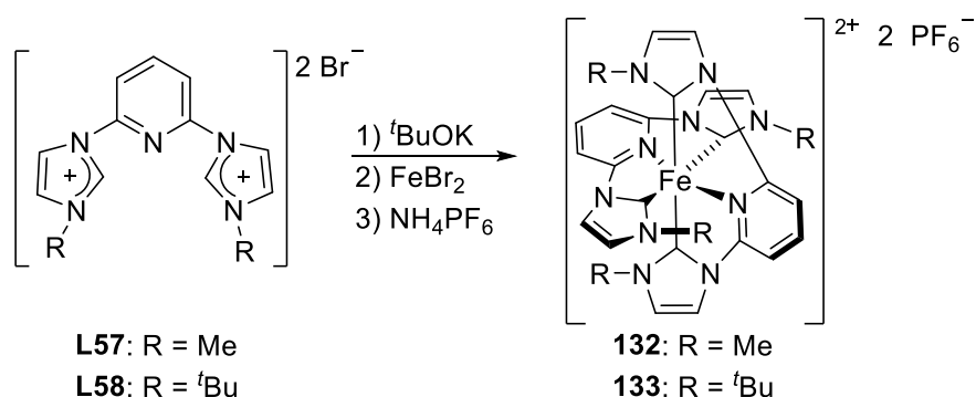
Scheme 40. Fe(II) complexes bearing two (bis-NHC)-pyridine ligand. 53
