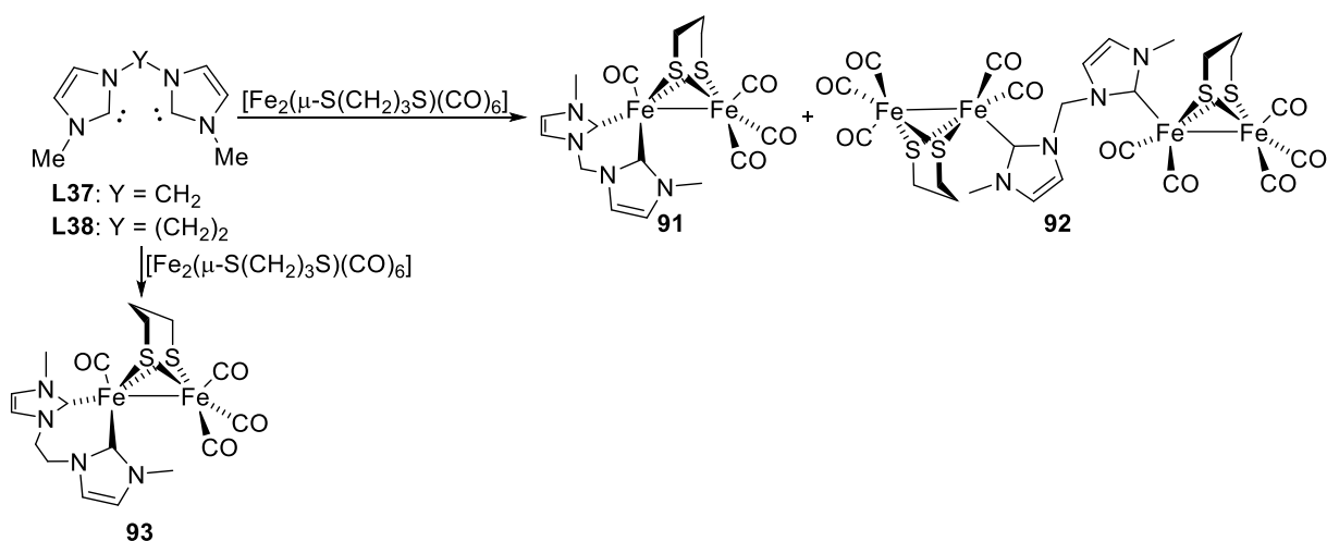
Scheme 26. Fe-S complexes bearing bis-NHC ligands. 39
