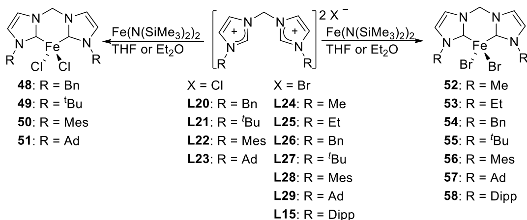
Scheme 18. Fe(II) complexes bearing a methylene bridge bis-NHC ligand. 30-31
