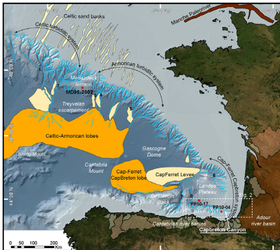
Fig. 1. Shaded bathymetry of the Bay of Biscay that shows the localisation of the margins and associated canyons: 1: Whittard, 2: Shamrock 3: Blackmud, 4: Guilder, 5: Audierne, 6: Capferret, 7: Capbreton, and 8: Santander. The Celtic and Armorican systems meet in adjacent lobes in the north, and the Cap-Ferret and Capbreton systems meet in one lobe with an associated levee in the south. Three cores of the study are shown: PP10-17 and PP10-04 from the SARGASS cruise and the stratigraphic reference MD95-2002. The shaded bathymetry combines data from the new SARGASS cruise (July 2010) and from the following former cruises: ITSAS (Bordeaux 1 University), SEDIFAN, SEAFER and ZEE IPREMER.
