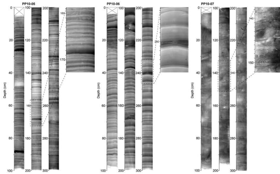
Fig. 5. Details of X-ray imagery for the cores located on the terraces. The zoom-in represents the most typical facies of each core. The cores nearest the thalweg, PP10-05 and PP10-06 are highly laminated, whereas PP10-07 is more bioturbated.
