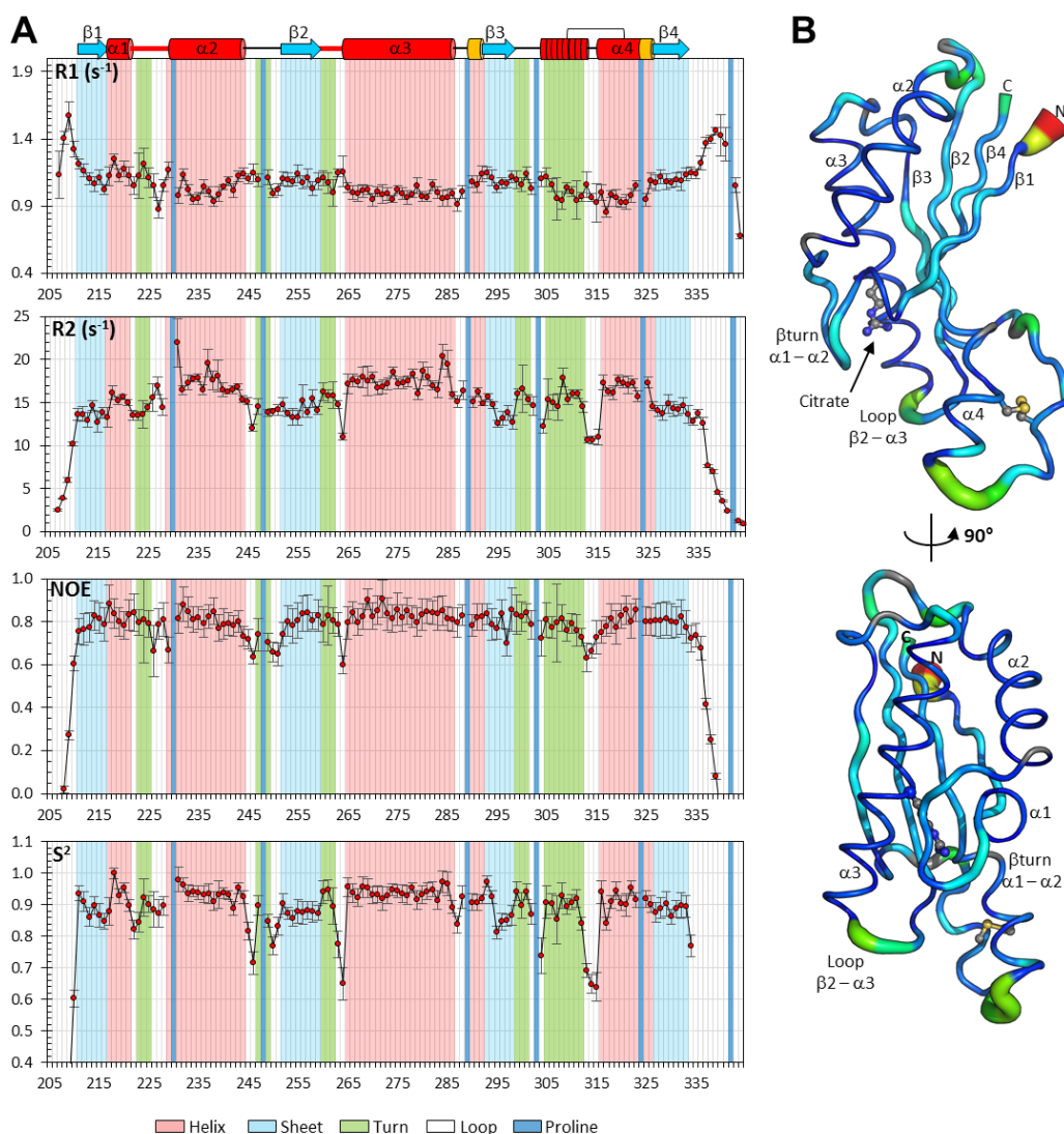
Figure 9. A. Backbone dynamics of C-KpOmpA. ^{15}\text{N} R1, ^{15}\text{N} R2, ^1\text{H} - ^{15}\text{N} steady-state heteronuclear NOEs and S^2 order parameter are plotted as a function of residue number. Secondary structures are shown on the top and by the background color. B. Sausage representation C-KpOmpA structure colored by S^2 order parameter. Radius of cartoon representation is proportional to the inverse of S^2 order parameter. Residues for which no data are available are shown in grey.
