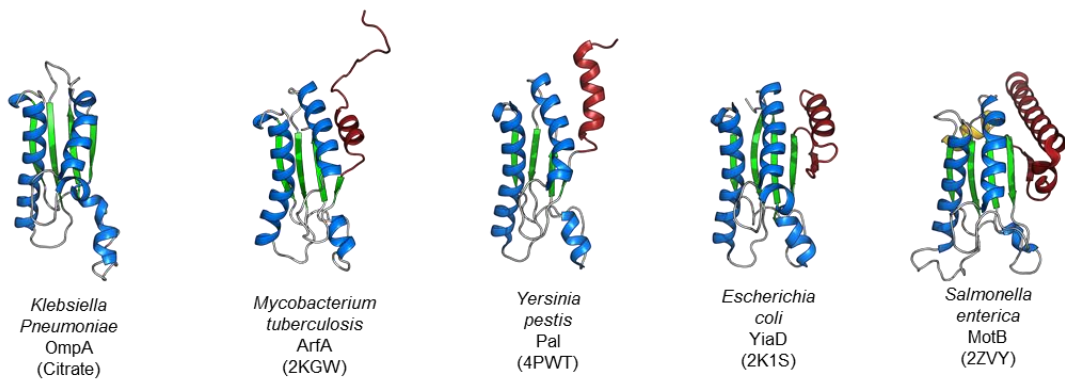
Figure 6. Structures of Klebsiella pneumoniae OmpA, Mycobacterium tuberculosis ArfA (PDB ID: 2KGW), Yersinia pestis Pal (PDB ID: 4PWT), Escherichia coli YiaD (PDB ID: 2K1S) and Salmonella enterica MotB (PDB ID: 2ZVY). Secondary structure elements of the core of OmpA-like domain are colored in blue and green. Supplementary elements in N-terminal or C-terminal are colored in red and yellow, respectively.
