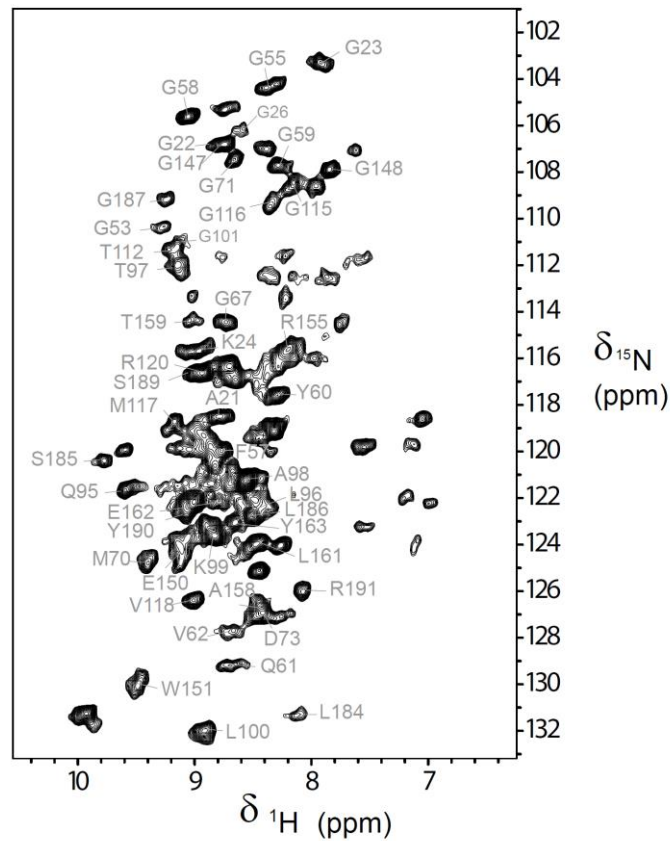
Figure 2. ^{15}\text{N} - ^1\text{H} correlation spectrum of [\text{U-}^{15}\text{N},^2\text{H},^{13}\text{C},^{15}\text{N}] -labelled KpOmpA reconstituted in Escherichia coli polar extract liposomes, recorded at 1 GHz spectrometer under 60 kHz MAS frequency and 25°C. Assigned residues are annotated.
