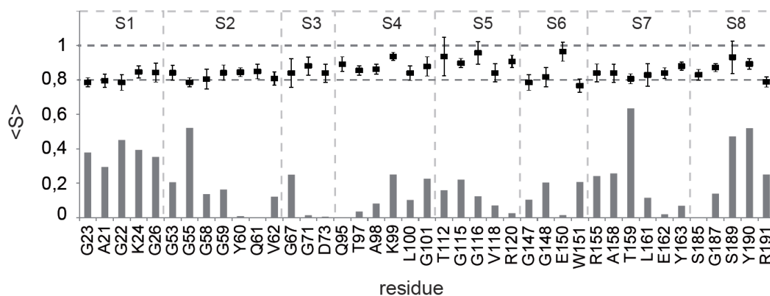
Figure 5. Histogram representation of amide bond order parameter (black box) per assigned residue (data in Supplementary Table S1). Grey bars represent the value of |(3\cos^2\beta-1)/2| , where \beta is the angle the amide bond angle with respect to the long principal axis of the system (i.e. \beta -barrel), which is assumed to be closed to the principal axis of the rotational diffusion motion ( \beta values were computed from the known 3D structure of KpOmpA, pdb 2K0L).
