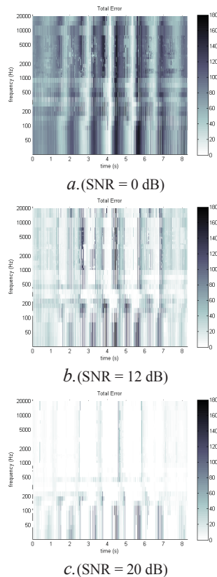
Fig. 7 Localization error of a random noise picked up with a cardioid microphone array in the presence of a disturbing source located at (\theta = 0, \phi = 0) . SNR is a. 0 dB, b. 12 dB and c. 20 dB
