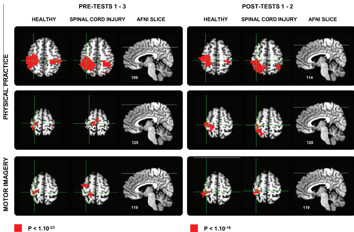
Fig. 4. Neural networks controlling actual and imagined prehension during the three pre- and the two post-tests, in healthy and spinal cord injury participants. The statistical threshold for detection of activations during the post-tests is higher than that in the pre-tests since only two masked activation maps were combined.
