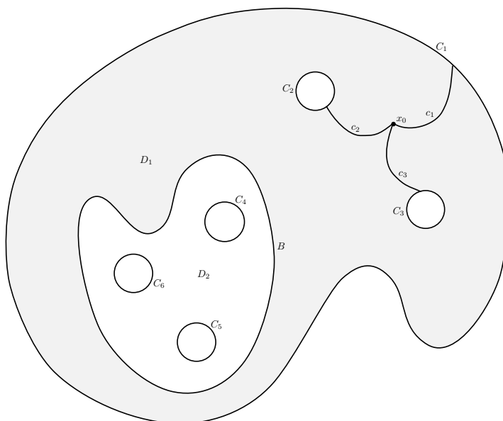
Figure 1.2: The geometry of D' in Lemma 1.2.1.
