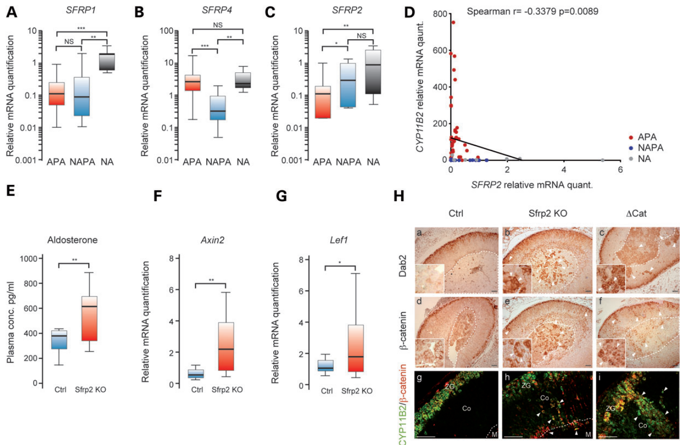
Figure 2. Down-regulation of SFRP2 expression is associated with WNT pathway activation and aldosteronism. (A–C) SFRP2 is down-regulated in APA. The expression of three members of the secreted frizzled related protein (SFRP), SFRP1 , SFRP2 , SFRP4 was analysed by RTqPCR on mRNAs from 35 APA, 17 NAPA and 7 NA. (D) SFRP2 and CYP11B2 expression levels are inversely correlated. RTqPCR data were used to correlate SFRP2 with CYP11B2 expression in a Spearman correlation analysis. (E) Sfrp2 knockout is associated with increased aldosterone production. Plasma aldosterone concentrations were measured in female control (Ctrl, Sfrp2 +/+ and Sfrp2 +/- ) and female homozygous Sfrp2 knockout mice ( Sfrp2 KO, Sfrp2 -/- ) at 13 months. Boxplots represent the quantification of aldosterone production in 11 female control and 13 littermate female knockout mice. (F and G) Wnt signalling is increased in the adrenals of Sfrp2 knockout mice. Axin2 (F) and Lef1 (G) expression levels were analysed by RTqPCR on mRNAs from control and homozygous Sfrp2 knockout mice. Boxplots represent the relative quantification of gene expression in 11 female control and 13 female knockout mice. (H) Genetic ablation of Sfrp2 results in aberrant activation of \beta -catenin and ectopic differentiation of zona-glomerulosa cells. Expression of Dab2 (a–c) \beta -catenin (d–f) and co-expression of \beta -catenin (red) and Cyp11b2 (green, g–i) was analysed by immunohistochemistry in wild-type ( Sfrp2 +/+ ), Sfrp2 knockout ( Sfrp2 -/- ) and \Delta Cat mice (19). Insets were taken from the central adrenal regions, highlighted by dashed white lines. White arrowheads show ectopic Cyp11b2 , Dab2 and \beta -catenin-positive cells. Dashed lines show the boundaries between cortex and medulla. ZG, zona glomerulosa; Co, cortex; M, medulla. Scale bar is 80 \mu m. Statistical analyses in (A)–(C) were performed by non-parametric ANOVA (Kruskal–Wallis) followed by Dunn's post hoc test. Statistical analyses in (E)–(G) were performed by Welch's t -test, to account for different variances between groups. Similar results were obtained by Mann–Whitney analyses * P < 0.05; ** P < 0.005; *** P < 0.0005; NS, not significant.
