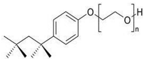
Triton X-100
