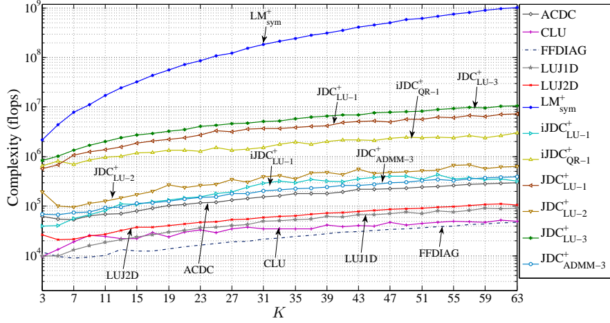
(b) Numerical complexity as a function of number K of matrices
