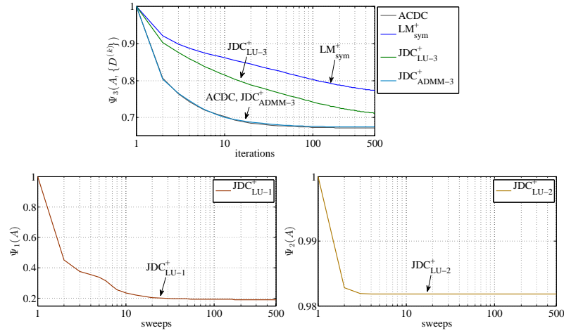
(a) Convergence as a function of sweeps/iterations with SNR = 30 dB
