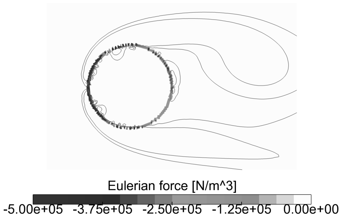
Figure 4.23: Eulerian force \dot{F}_{p,x} applied to the fluid with iso-lines of vorticity.
