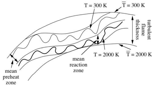
Figure 7.3: Illustration of the thickened-wrinkled flame regime proposed by Borghi and Destriau [164].
