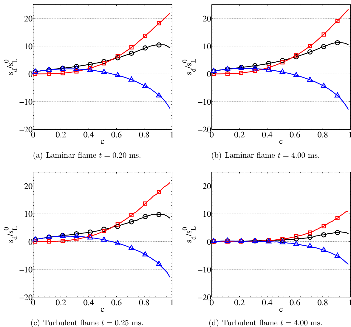
Figure 7.16: Displacement flame speed analysis (Eq. 7.17) for laminar and turbulent flames just after the ignition time and 4 ms after ignition. Local values of flame speeds are averaged on isosurfaces of c . \ominus : s_d ; \square : s_{reac} ; \triangle : s_{diff} .
