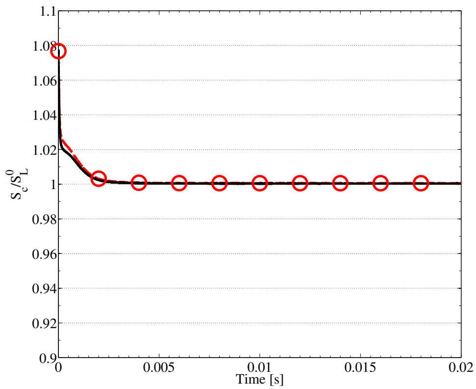
Figure 3.5: Normalized consumption speed versus time for an octane/air flame in a configuration without compression and confinement with s_L^{0,C^8H_{18}} = 0.264 m/s. — s_c (Eq. 3.3) ; -⊕- s_c^{p,expe} (Eq. 3.10).
