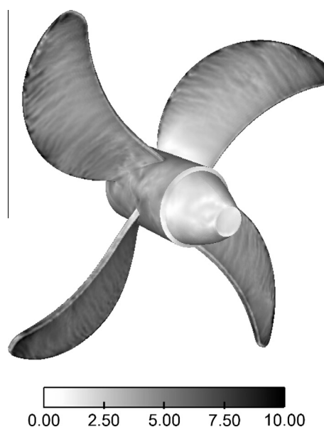
Fig. 6. y^+ field on the fan walls.
