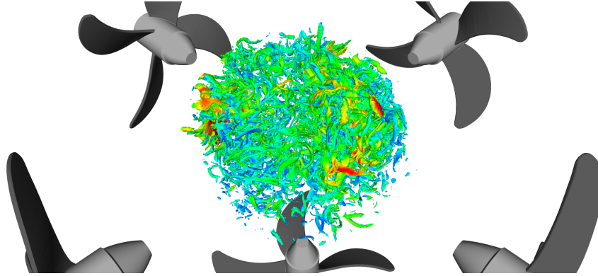
Figure 7.8: Instantaneous isosurfaces of vorticity at the bomb center colored by the velocity magnitude.
