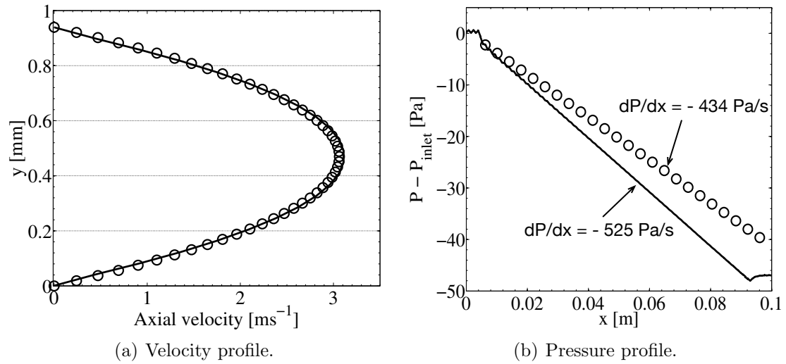
Figure 4.10: Velocity profile. ○ Theoretical profile ; — Immersed Boundaries Method
