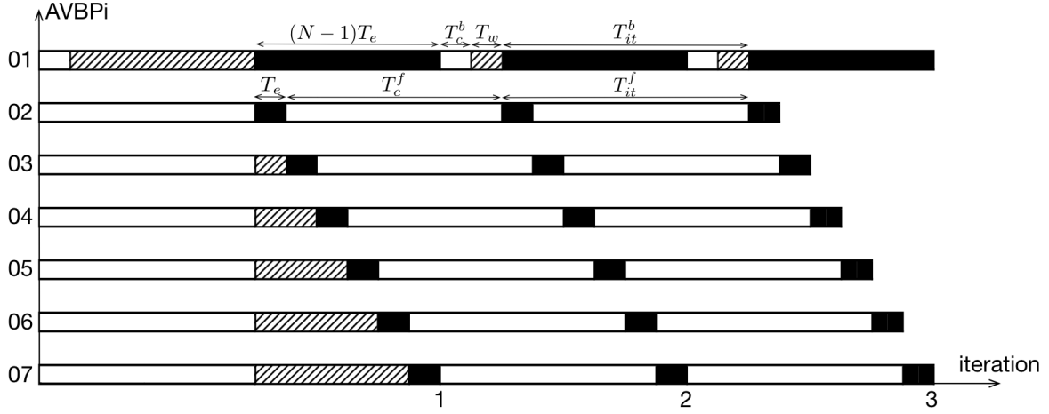
Figure 6.4: Timetable of the operations performed in the MISCOG approach for the FL case (only bomb waits). \square : Computing ; \text{///} : waiting ; \blacksquare : exchanging
