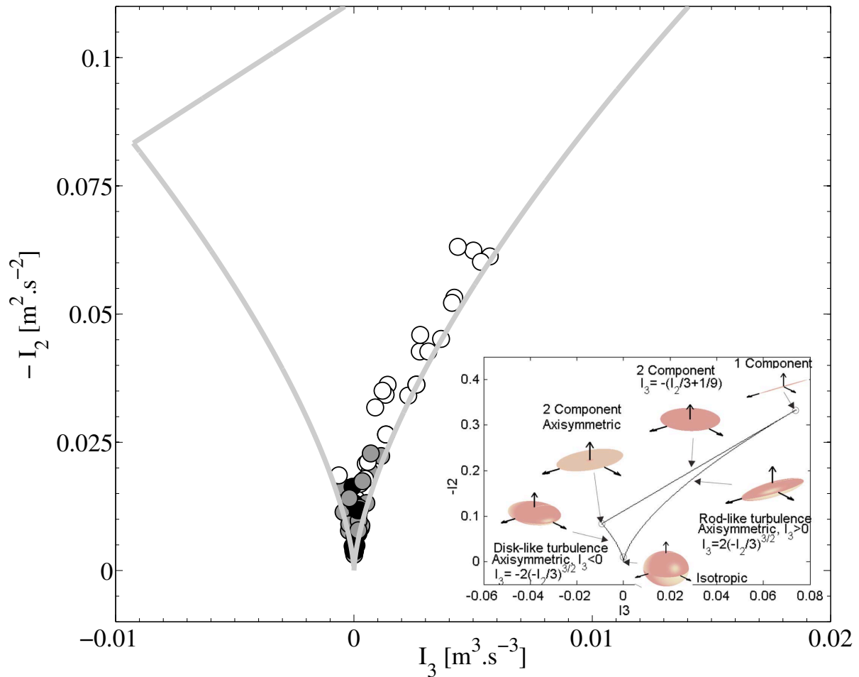
Figure 6.14: Anisotropy invariant map (Lumley triangle). Each point is colored by its distance r to the center of the bomb. ● : r < 15 mm ; ● : r \in [15; 30] mm ; ○ : r > 30 mm. The figure in the bottom-right hand side is taken from [157].
