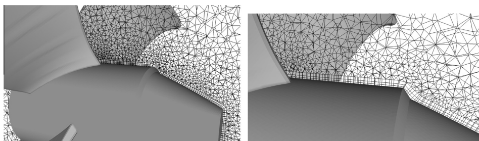
Fig. 5. Mesh of the fan. Four prism layers were added near blade-walls.
