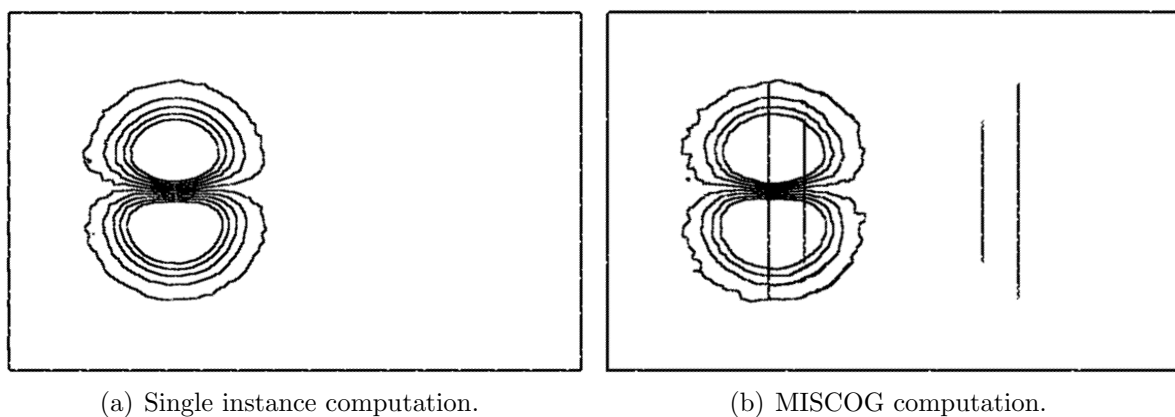
Figure 5.3: Comparison between a 'classic' single mesh AVBP computation and the MISCOG approach. Isolines of velocity after two convection times (the vertical lines in Fig. 5.3(b) indicate the position of the rotating cylinder and of the overlapping zone).
