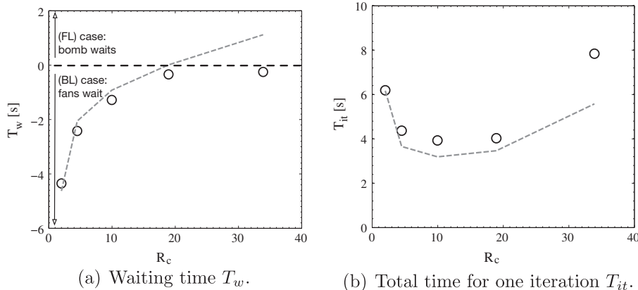
Fig. 9. Performance of MISCOG. ○: Computations; ----: model.
