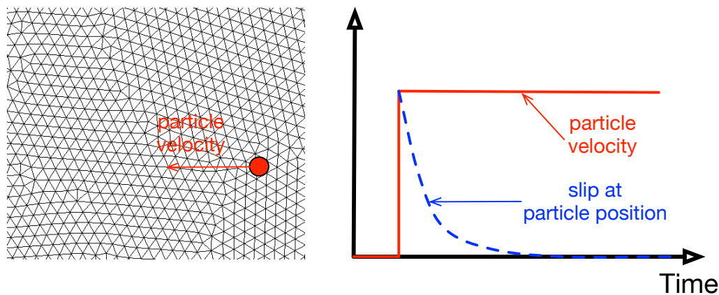
Figure 4.4: Sketch of the numerical configuration used to developed the numerical strategy to perform computations using IB.
