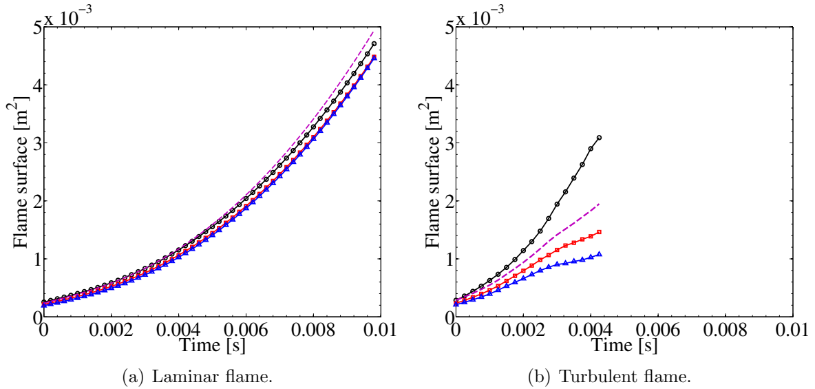
Figure 7.10: Flame surface. \circ —: c^*=0.1 ; \square —: c^*=0.5 ; \triangle —: c^*=0.9 ; -\cdot-\cdot- : \int_V \Xi |\nabla c| dV
