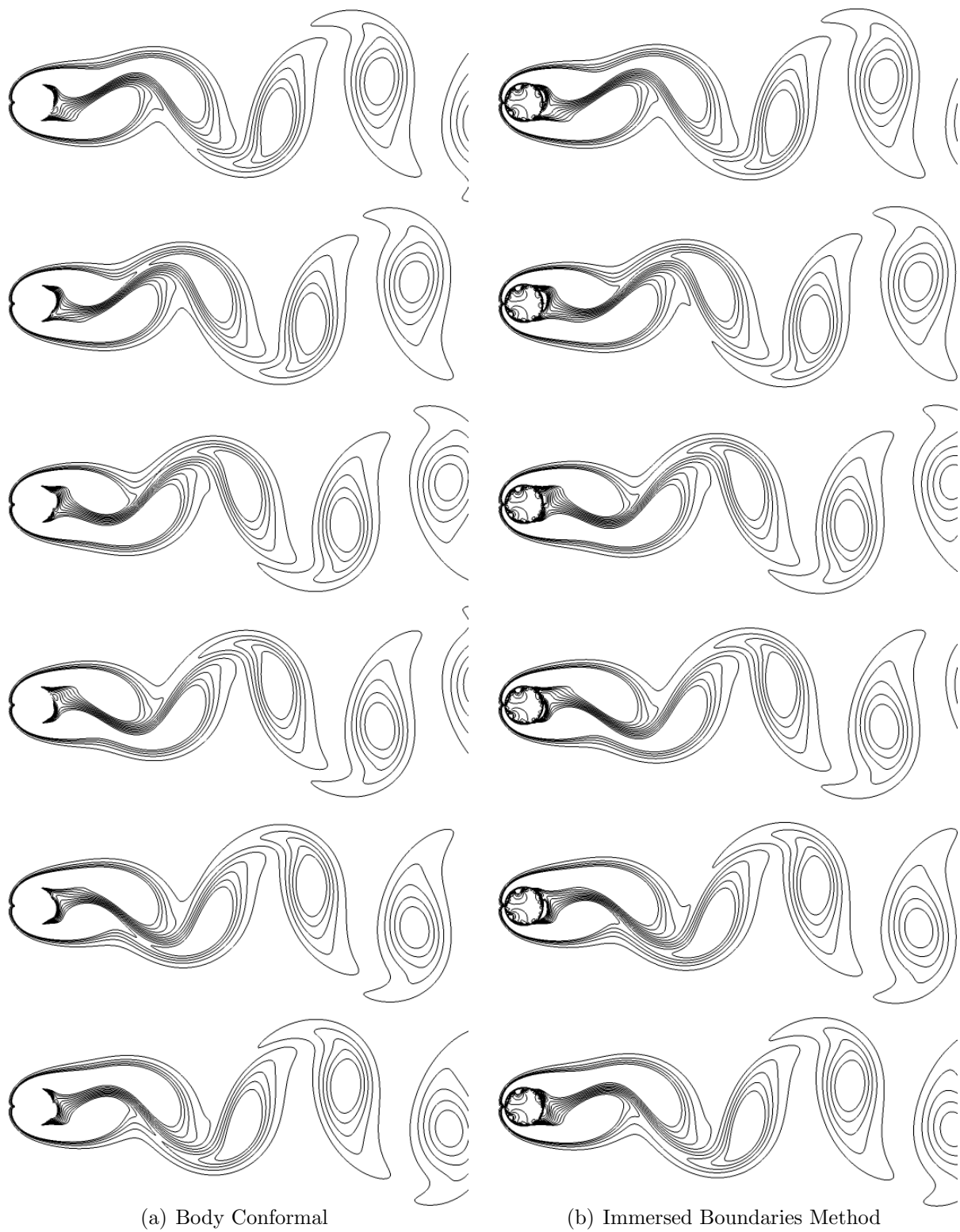
Figure 4.21: Vortex shedding at Re = 100 . Isolines of vorticity. Temporal evolution from top to bottom. Time step between to filed is 2.01 \times 10^{-4} s
