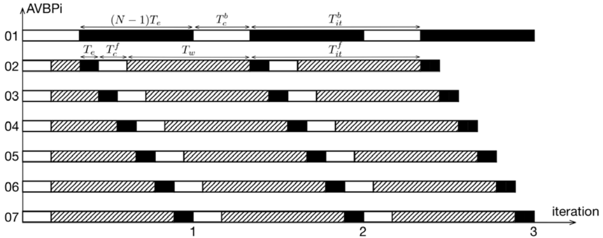
Figure 6.3: Timetable of the operations performed in the MISCOG approach for the BL case (only fans wait). \square : Computing ; \text{///} : waiting ; \blacksquare : exchanging
