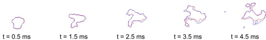
Figure 7.19: Flame propagation illustrated by instantaneous isolines at c^* = 0.9 . — : velocity field unchanged (Fig. 7.18(a)) ; — : velocity field set to zero (Fig. 7.18(b)).
