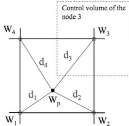
Figure 4.3: Example of projection of a particle two-way coupling contribution into the vertices of a quadrilateral cell
