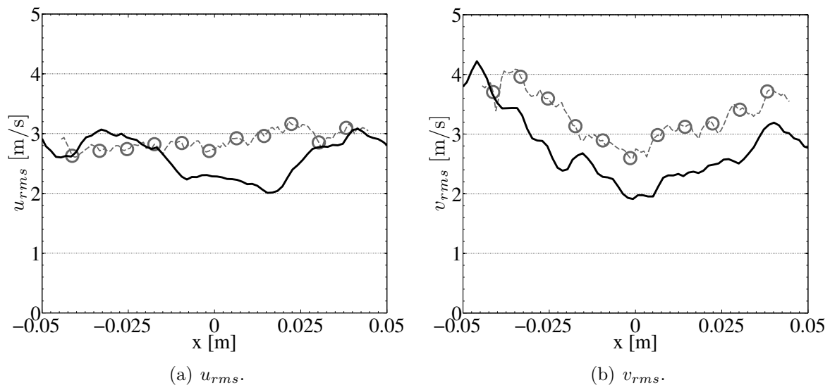
Figure 6.10: Comparison of the fluctuating velocities u_{rms} and v_{rms} along the x-axis. -\circ--\dagger : experimental data (PIV) ; — : LES. (Statistics performed on 60 fan rotations)
