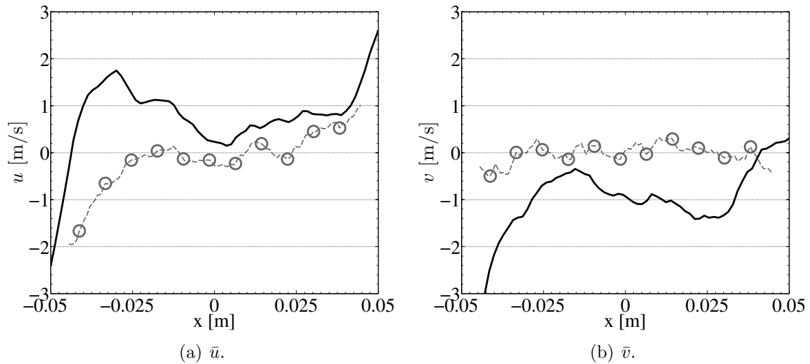
Figure 6.9: Comparison of the average velocities \bar{u} and \bar{v} along the x-axis. -\circ--\dagger : experimental data (PIV) ; — : LES. (Statistics performed on 60 fan rotations)
