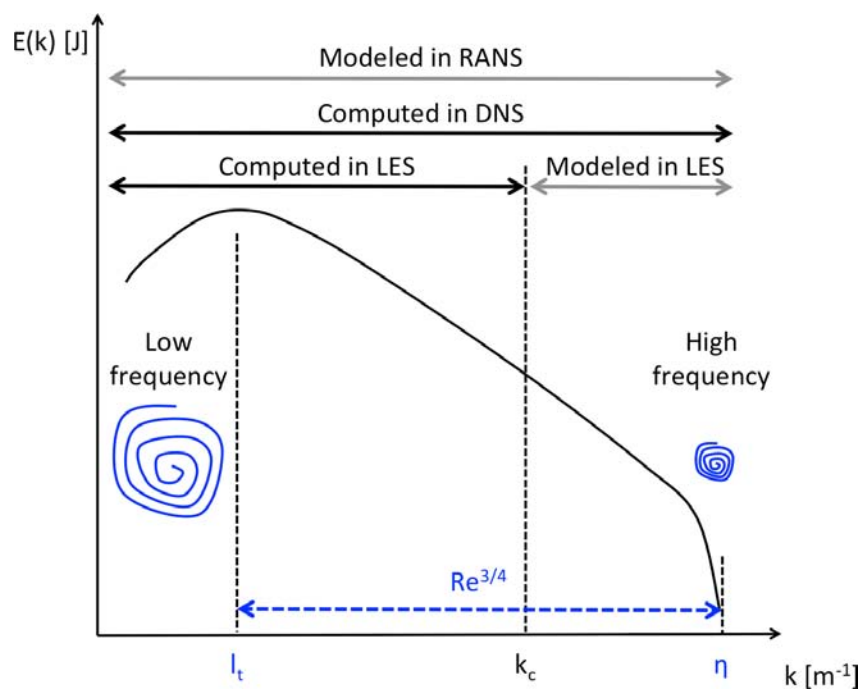
Figure 1.2: Log-log turbulence energy spectrum versus wave number. k_c is the cut-off wave number used in LES.
