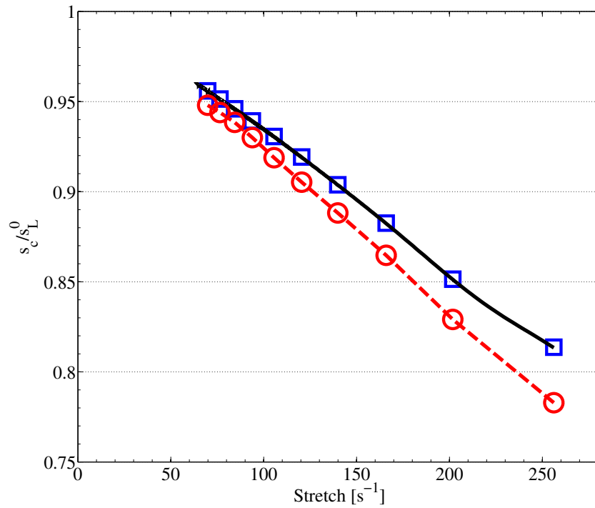
(a) Octane.
