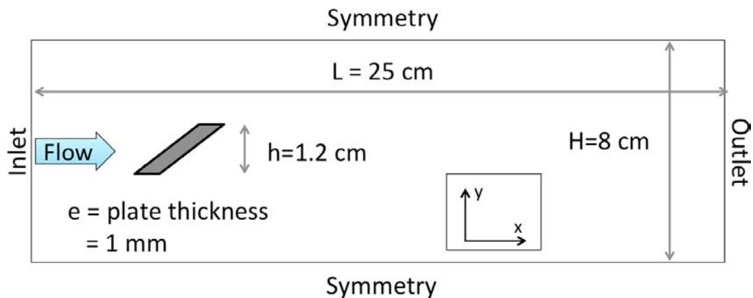
Figure 4.26: Sketch of the configuration: inclined plate.
