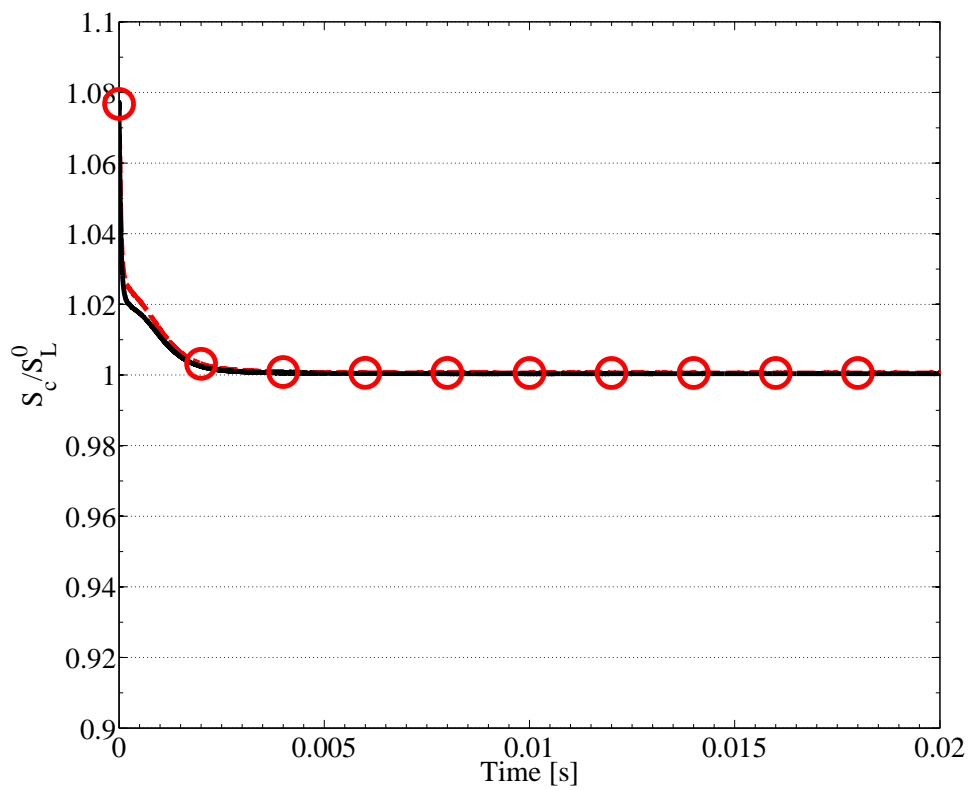
Figure 3.5: Normalized consumption speed versus time for an octane/air flame in a configuration without compression and confinement with s_L^{0 \text{ C}8\text{H}18} = 0.264 m/s. — s_c (Eq. 3.3) ; -⊕- s_c^{p expe} (Eq. 3.10).
