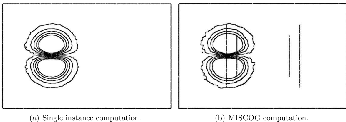
Figure 5.3: Comparison between a classic single mesh AVBP computation and the MISCOG approach. Isolines of velocity after two convection times (the vertical lines in Fig. 5.3(b) indicate the position of the rotating cylinder and of the overlapping zone).
