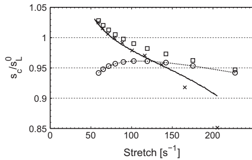
(b) Methane.
