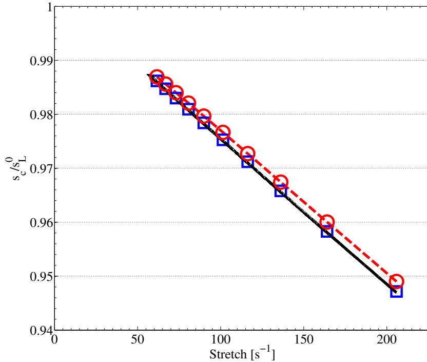
(b) Methane.
