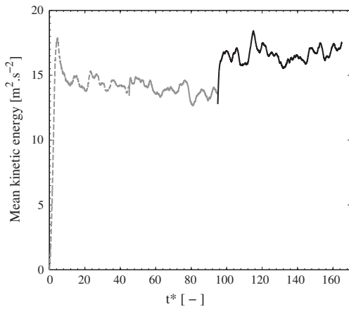
Fig. 10. Mean kinetic energy in the closed vessel versus the number of fan rotations t^* . - - - - : coarse grid LW; ———: coarse grid TTGC; - · - · : fine grid TTGC.
