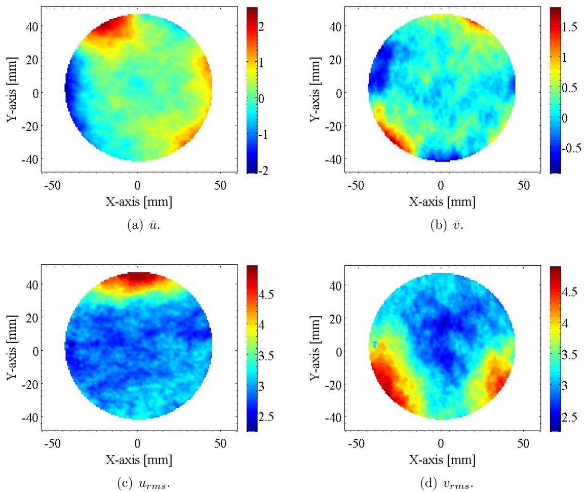
Figure 2.4: Experimental average and fluctuating velocities measured using PIV. Fans rotation speed is N_{fan} = 10\ 000 rpm.
