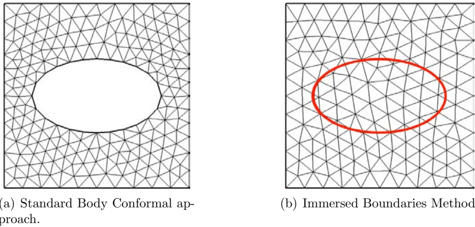
Figure 4.1: Comparison of the Immersed Boundaries Method (IBM) to the classic Body Conformal (BC) approach.
