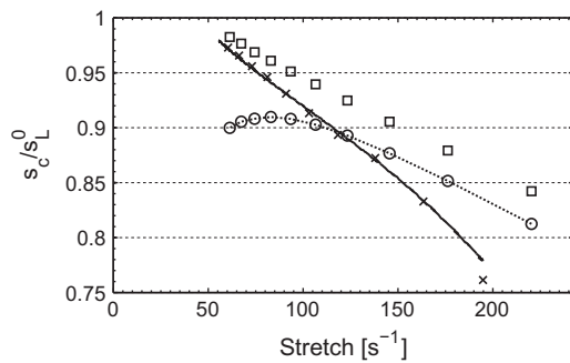
(a) Octane.
