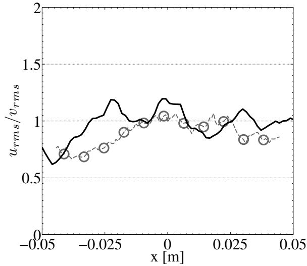
Figure 6.15: Isotropy along the x-axis. -\circ-\circ- experimental data (PIV) ; — : LES.
