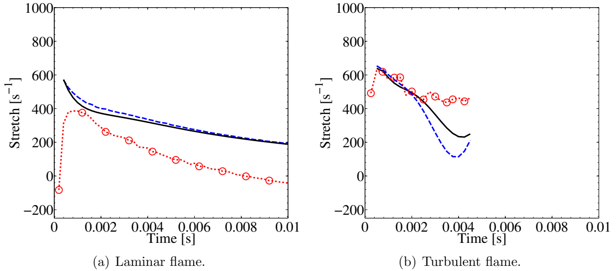
Figure 7.12: Evolution of stretch and curvature during the propagation phase. — : \kappa_\Sigma (Eq. 7.4) ; \cdots\circ\cdots : \langle \kappa \rangle (Eq. 7.7) ; - - - : \kappa (Eq. 7.8)
