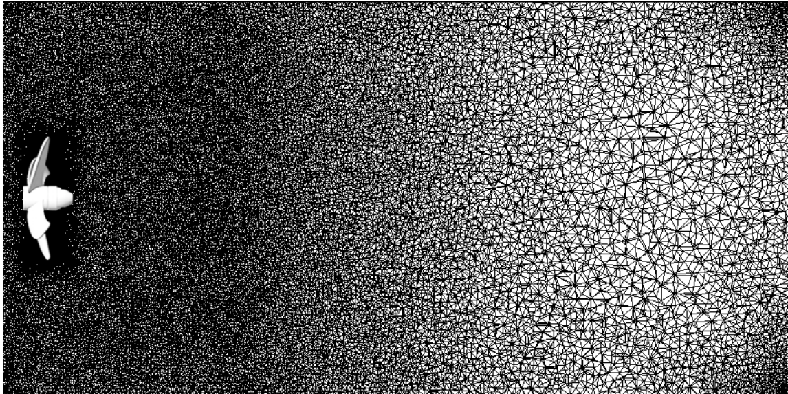
Figure 4.34: One-fan experiment mesh. 13.7 millions of tetrahedra.
