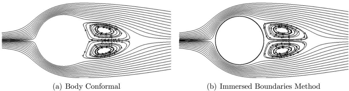
Figure 4.20: Streamline around a cylinder at Re = 20
