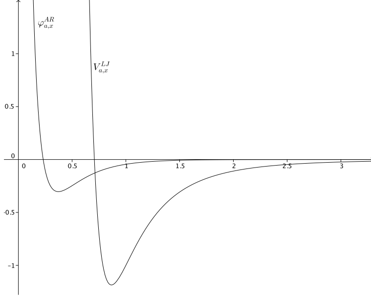
FIGURE 7 – Courbes de \varphi_{a,x}^{AR}(r) = 2\frac{e^{-6r}}{r} - \frac{e^{-3r}}{r} et V_{a,x}^{LJ}(r) = \frac{1}{r^6} - \frac{2}{r^4}
