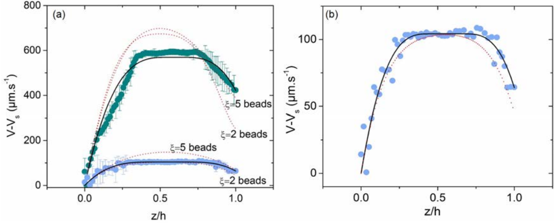
Figure 4.12 – (a) Velocity profiles V corrected from the slip velocity V_s in a channel of 7 \mu\text{m} height. The reduced stress \sigma/\sigma_y = 9.6 (dark cyan), 4.5 (blue). The boundary conditions are 20^\circ\text{-}70^\circ for the top curve and 20^\circ\text{-}20^\circ for the bottom curve. The black solid lines are the best fits to the theoretical expression of the velocity profiles calculated in the asymmetric Herschel-Bulkley flow model. The dashed red lines are the theoretical expression calculated from the cooperative model, where the bulk fluidity and the boundary condition are equal to the asymmetric Herschel-Bulkley model of the profiles. (b) Closer look to the bottom curve of (a).
