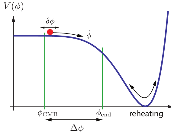
Figure 1.6: An example for the potential of the inflaton. Acceleration occurs when V is more important than the kinetic term. Inflation ends at \phi_{\text{end}} when the slow roll conditions are violated. CMB fluctuations are created by quantum fluctuation \delta\phi about 60 e -folds before the end of inflation. At reheating, the energy density of the inflaton is converted into radiation ( Baumann 2009 ).
