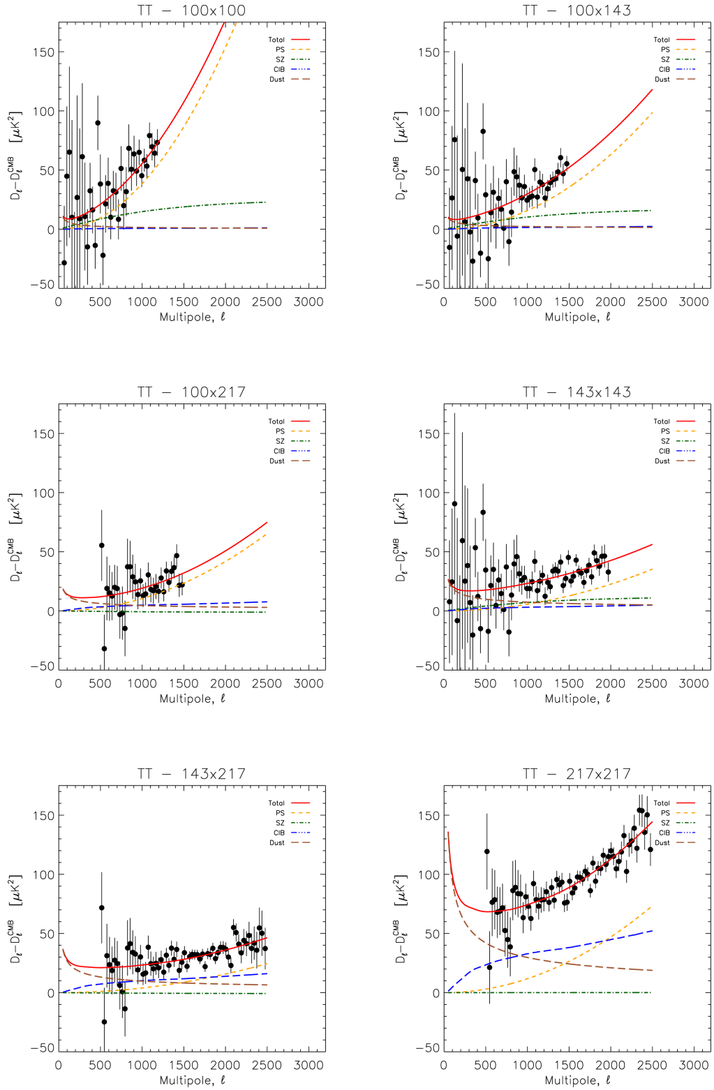
Figure 5.34: Temperature foreground residuals for all the cross-frequency spectra. The best fit level of each residual foreground contribution is also plotted.
