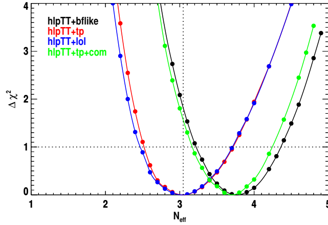
Figure 8.11: Profiles for the N_{\text{eff}} parameter for the HiLLiPOP (TT) likelihood in combination with different choices of the low- \ell information. The black curve is obtained with the LowTEB likelihood. The \tau prior case (standard Gaussian prior 0.07 \pm 0.02 ) is in red. The \tau prior + Commander case is in green. The lollipop likelihood is also considered (in blue). The corresponding mean and errors can be found in Table. 8.3. The vertical dotted line indicates the standard 3.046 value.
