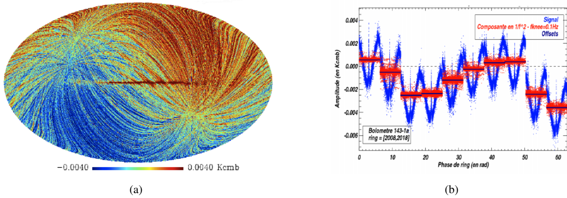
Figure 3.10: (a) The effect of low frequency noise on a map are peculiar strips parallel to the scan direction. We can also recognise the Galactic plane and the solar dipole. (b) Illustration of 1/f noise. The offset are considered constant for each ring, and are fitted and subtracted at mapmaking level (Filliard 2012).
