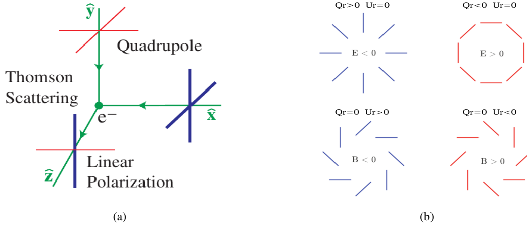
Figure 1.11: (a) Thompson differential cross section (see text) favours the absorption of the components that are parallel to the incoming one. Hence, a quadrupolar anisotropy in the incoming radiation can induce a linear polarisation (Hu & Dodelson 2002). (b) Examples of E-mode and B-mode patterns of polarisation. Adapted from Baumann et al. (2009).
