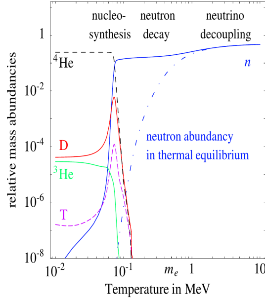
Figure 2.5: Evolution of the main nuclear components of the BBN. The figure is taken from Strumia & Vissani (2006)
