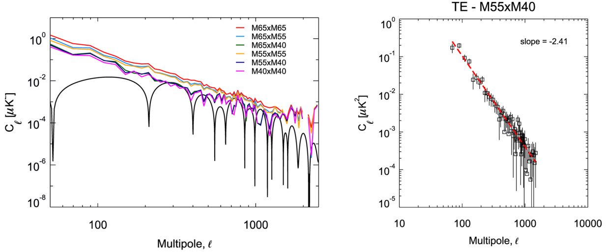
Figure 5.16: Left: 353x353 TE power spectra. The black line is the CMB TE power spectrum. The color lines are the CMB subtracted 353x353 TE power spectra estimated for different set of masks as defined in Table 5.2. Right: fit of the CMB subtracted 353x353 TE power spectrum estimated for M55xM40. The black squares are the data and the red dashed line is the best fit to these data.
