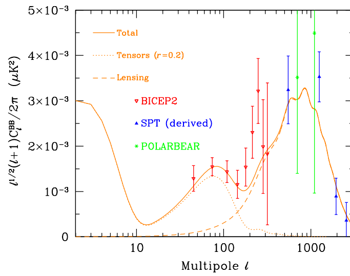
Figure 1.17: Status of BB measurements. In green the POLARBEAR direct measurements of the lensed B-modes ( The Polarbear Collaboration; P. A. R. Ade et al. 2014 ). In blue the SPT points derived from cross correlation with lensing ( Hanson et al. 2013 ). In red the BICEP2 measure at the level of the recombination bump ( Chiang et al. 2010 ). The figure is taken from the Particle Data Group (PDG) ( Olive et al. 2014 )
