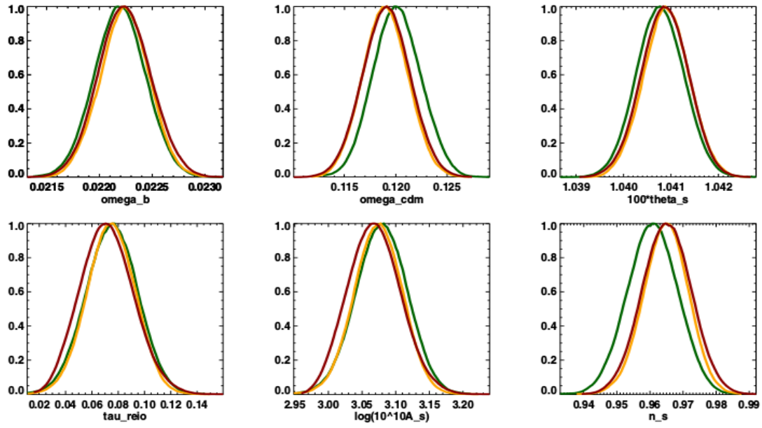
Figure 7.8: Posterior distributions for HiLLiPOP likelihood for the high- \ell part ( \ell_{\text{min}}=50 ) adding for the low- \ell part the standard \tau Gaussian prior 0.007 \pm 0,02 (green), \tau prior + Commander between \ell_{\text{min}}=2 and \ell_{\text{max}}=29 (yellow), and the LowTEB likelihood (red).
