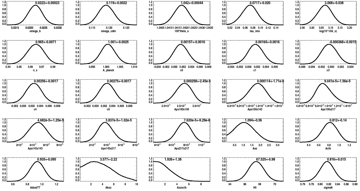
Figure 7.2: Posterior distributions for the temperature only HiLLiPOP likelihood in combination with the LowTEB likelihood. We show the six \Lambda CDM parameters and the nuisances (described in Table 5.7) plus two interesting derived parameters: H_0 and \sigma_8 . The means and the 68% errors can be found in Table 7.2. These results have been obtained using CLASS.
