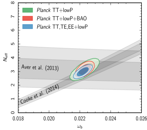
Figure 2.6: Planck constraints in the \Omega_b h^2 - N_{\text{eff}} plane compared to confidence regions derived from ^4\text{He} and deuterium measurements. Y_p is fixed as a function of \Omega_b h^2 and N_{\text{eff}} . Figure is taken from Planck Collaboration, XIII. (2015) .
