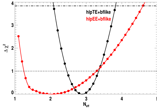
Figure 8.14: Profile likelihood for HiLLiPOP likelihood in combination with the LowTEB at low- \ell . The results are shown in black for TE and in red for EE. The asymmetry of the EE limit comes from the underlying neutrino model assumed. We are, indeed, considering two massless and one massive (0.06 eV) active neutrino, so N_{\text{eff}} , in CLASS, is greater than one by definition.
