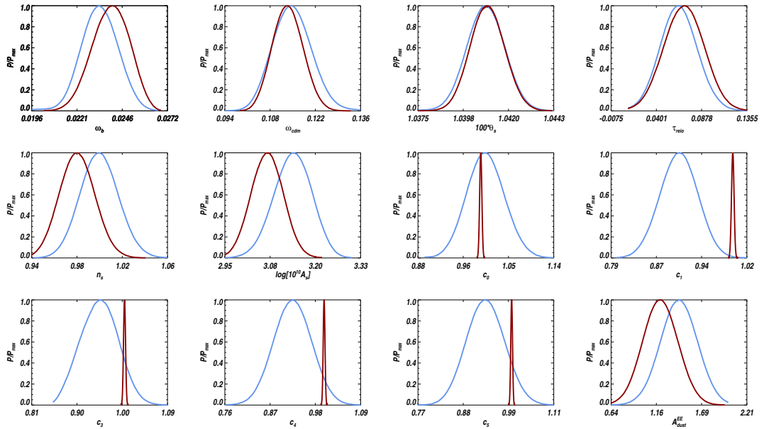
Figure 5.28: Posterior distributions for the EE HiLLiPOP likelihood in case of strong Gaussian priors on calibration parameters (red) or letting the calibration free (blue).
