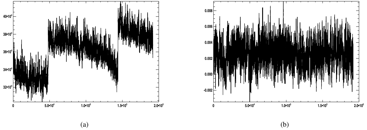
Figure 4.7: (a) Example of bad mixing for a given variable (b) Example of good mixing for another given variable. These example are nuisance parameters taken from different test run of our CMB likelihood.
