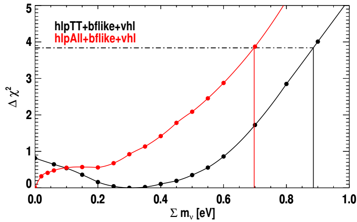
Figure 8.6: The baseline HiLLiPOP (TT) + LowTEB + VHL (in black) is compared to the full HiLLiPOP likelihood +LowTEB + VHL (in red).
