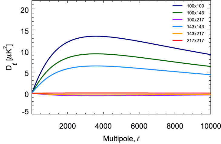
Figure 5.18: The tSZ power spectra templates. A global scaling, A_{\text{tSZ}} , is left free in the analysis
