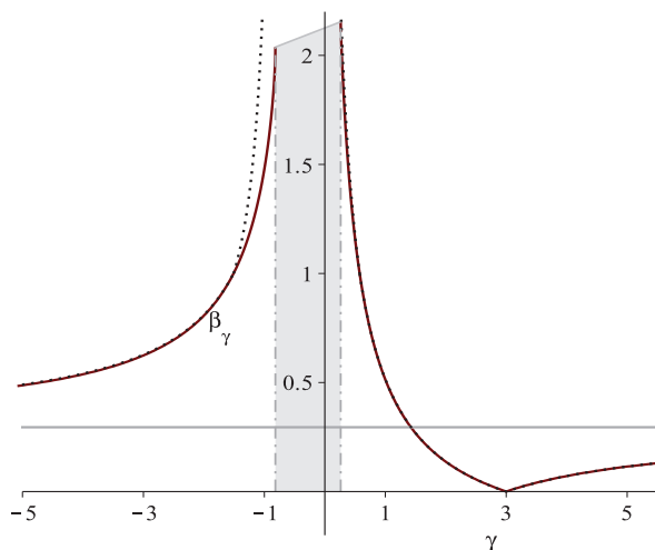
Fig. 9. The plot of \beta_\gamma in the interval \gamma \in (-\infty, -0.817] \cup [0.262, +\infty) (continuous line) and the upper estimate of \beta_\gamma provided by Theorem 2.2 (dotted line).
