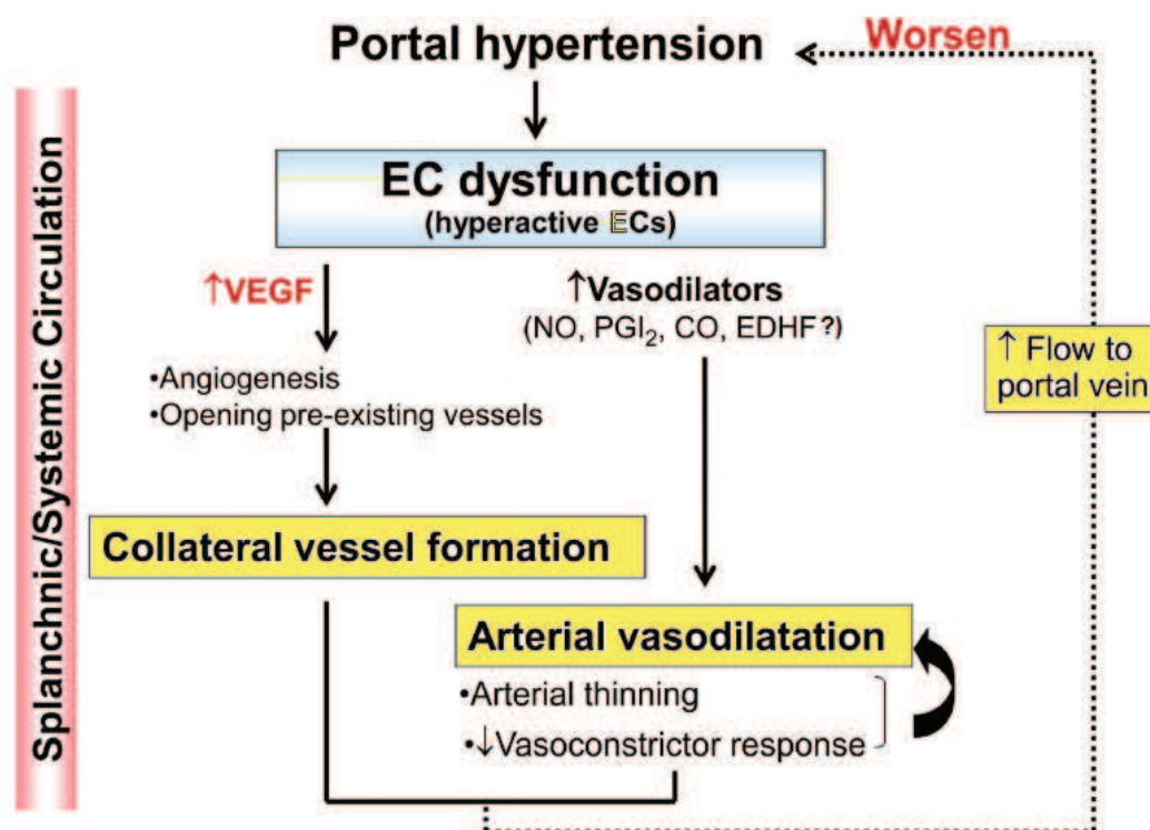
Figure 10. Overview of factors contributing to PH initiation and it is worsening. (Iwakiri 2012).
