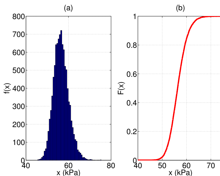
Figure 2.7 – Output histogram of the ULS case for a rectangular wall with one free edge and three clamped edges with normal independent inputs (a), and the cumulative distribution function associated (b).
