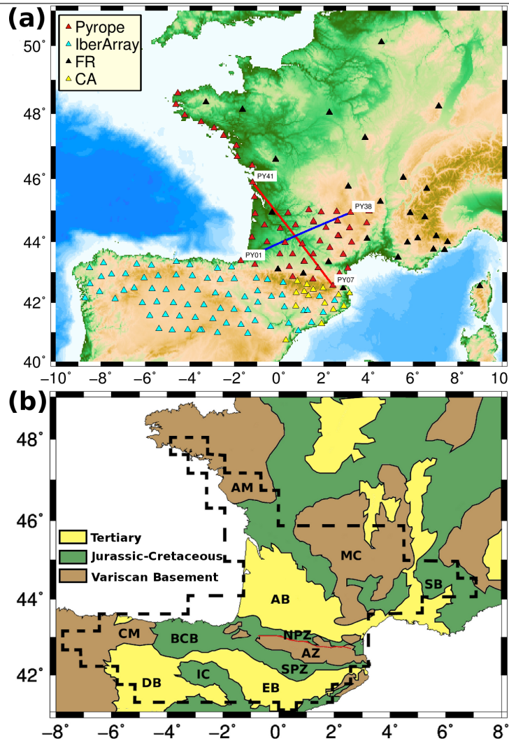
FIGURE 2.6 – (a) Map of the 158 seismic broadband stations used in the present study, corresponding to 12324 station pairs. Red and blue lines, stations pairs used in Figure 2.7. (b) Simplified geological map of the study zone. Red line, the North Pyrenean fault ; dashed black line, limits of the well-resolved zone of the tomography ; AB, Aquitaine basin ; AM, Armorican Massif ; AZ, Axial Zone of the Pyrenees ; BCB, Basque-Cantabrian basin ; CM, Cantabrian mountains ; DB, Duero basin ; EB, Ebro basin ; IC, Iberian chain ; MC, Massif Central ; NPZ, North Pyrenean Zone ; SB, south-eastern basin ; SPZ, south Pyrenean Zone.
