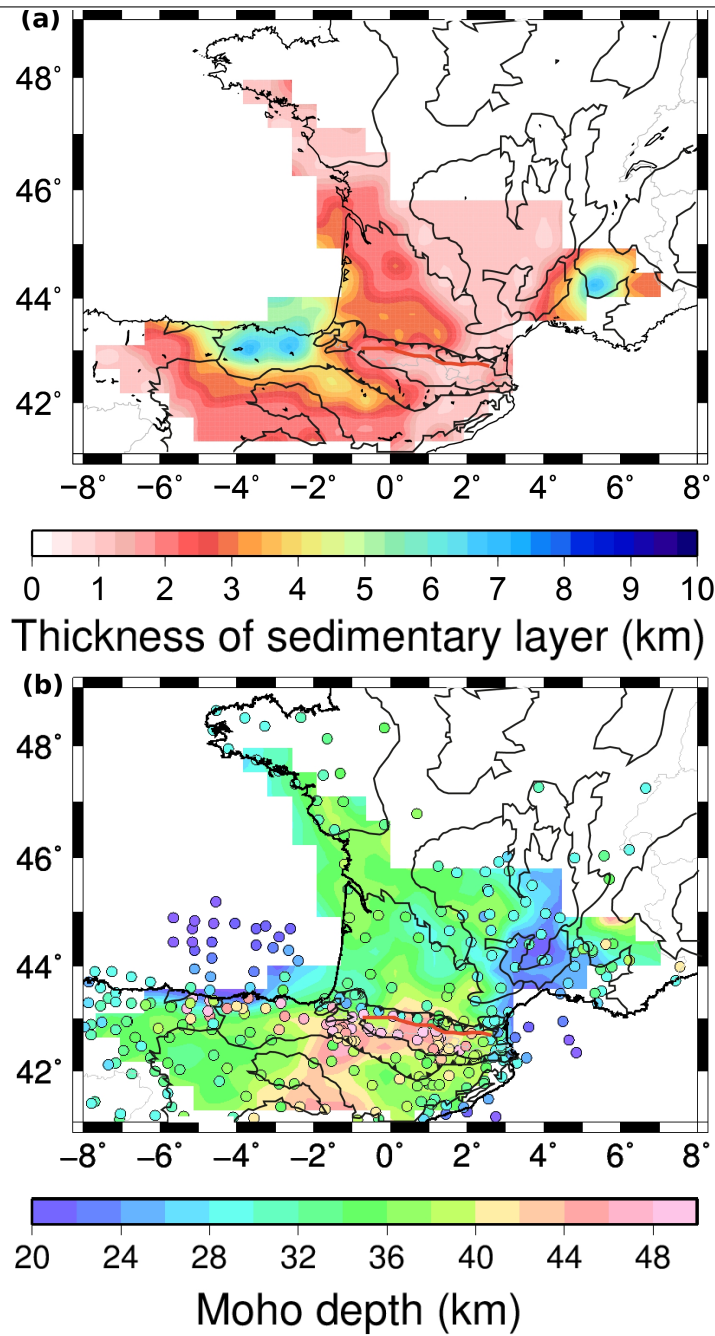
FIGURE 2.12 – Maps of the iso-velocity depths : (a) Iso-velocity V_S = 2.9 \text{ km.s}^{-1} associated with the top of the basement. (b) Iso-velocity V_S = 4 \text{ km.s}^{-1} associated with the crust-mantle boundary. Filled circles, Moho depth values that Chevrot et al. (2014b) estimated from receiver functions or compiled from seismic reflection-refraction studies ; solid black lines, main geological boundaries of Figure 2.6b .
