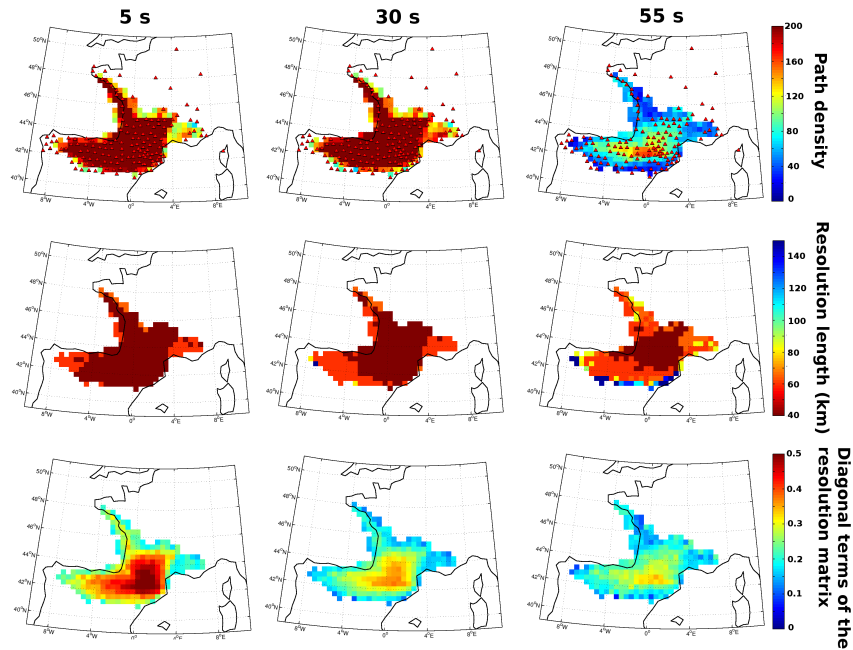
FIGURE 2.17 – Maps of the path density (top), resolution length (middle), and diagonal of the matrix of resolution (bottom) at 5 s, 30 s and 55 s. Red filled triangles (top panels), station locations.
