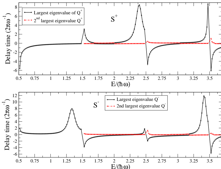
Figure 3.12: Delay time (eigenlifetime) indicating the peaks are of resonant nature. Two largest eigenvalues of +parity time delay matrix Q^+ (top panel) and -parity time delay matrix Q^- (bottom panel).
