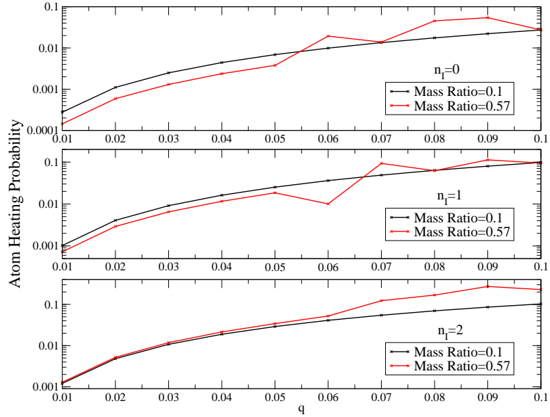
Figure 4.21: Atom heating probabilities for shallow confinement with m_A/m_I = 0.1, 0.57 , a = 0.5 , E_{tot} = 2.7\beta/2 .
