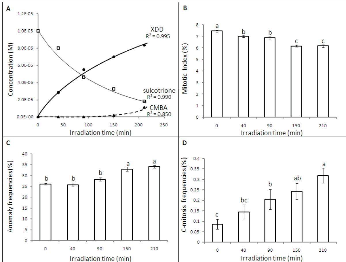
Figure 1. Analysis of sulcotrione photodegradation kinetics. (A) Concentrations of CMBA (▲) and XDD (●) during 210 min of photodegradation of sulcotrione solution ( 1 \times 10^{-5} M) (□) determined by HPLC analyses (detection at 284 and 243 nm). Sulcotrione, XDD and CMBA concentrations follow Quadratic, Michaelis Menten and exponential function respectively, R^2 are indicated for each regression curve. Mitotic index (B) , anomaly frequencies (C) and C-mitosis frequencies (D) were evaluated in root tips cells after 48 h treatment with sulcotrione solution after different time (0, 40, 90, 150, 210 min) of UV degradation (290–420 nm). Data represent an average ( \pm SE) of 3 bulbs. The results of Tukey HSD all-pairwise comparisons test are indicated by different letters where values differ significantly at p < 0.05 .
