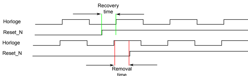
FIGURE 3.20 – Exemple de recovery time et removal time.
