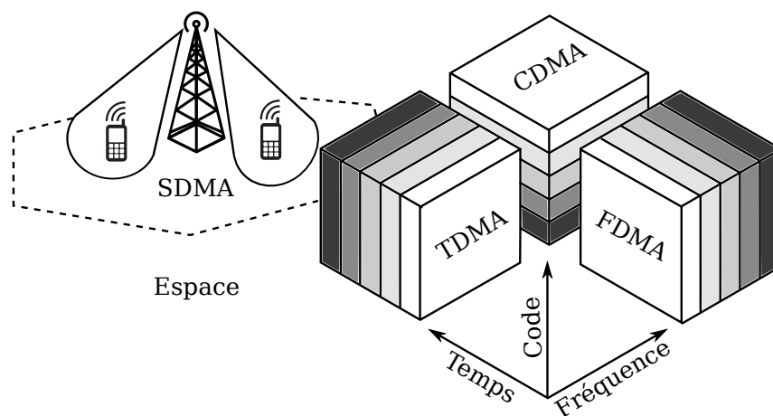
FIGURE 1.5 – Techniques de multiplexage.
