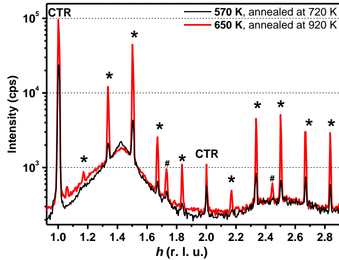
Figure IV.4 – Radial-scans along the Si[ \bar{1}21 ] azimuth highlighting the liquid structure factor and the (6 \times 6) signature (stars) for a 30 ML deposit of gold annealed at different temperature (720 K and 920 K).
