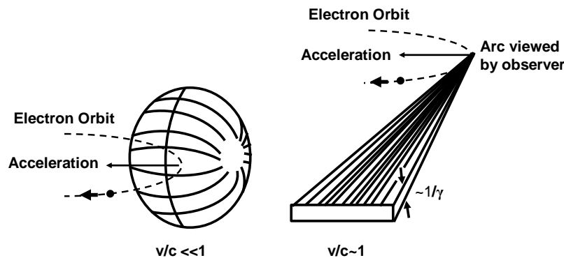
Figure II.13 – Illustration of the radiation emission of electrons in circular motion. Left : non-relativistic case, right : relativistic case. From [Als-Nielsen et al. , ].
