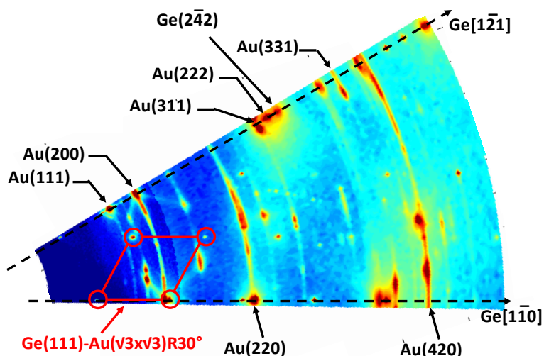
Figure VI.6 – Reciprocal space map of the Au-Ge system in the solid state (at RT) after melting and solidification. The red, and blue colors refer to high and low intensity, respectively. The yellow colors represents intermediate intensities
