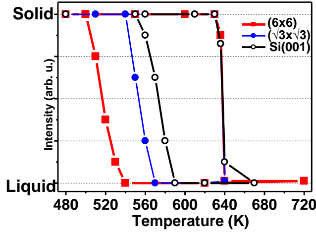
Figure V.6 – Schematic evolution of the Bragg intensity highlighting the solid-liquid-solid phase transition cycles for Si(001), Si(111)- (\sqrt{3}\times\sqrt{3})R30^\circ Au and Au on Si(111)- (6\times 6) Au substrates.
