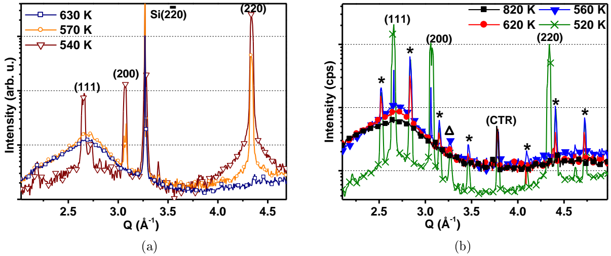
Figure V.18 – Radial-scans for a 30 ML deposit (a) along the [\bar{1}\bar{1}0] azimuth at 630 K, 570 K and 540 K and (b) along the [\bar{1}\bar{2}1] azimuth at 820 K, 620 K, 560 K and 520 K, in this case the sample was previously annealed at 940 K
