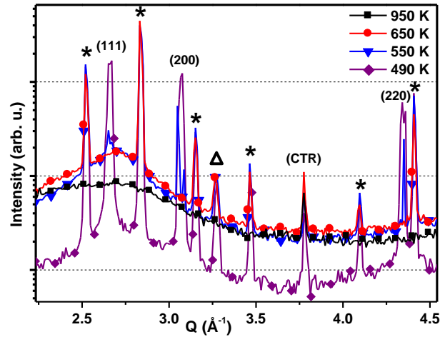
Figure V.19 – Radial-scans along the [1\bar{2}1] azimuth at 950 K, 750 K, 650 K and 490 K, for the 2+8 ML sample.
