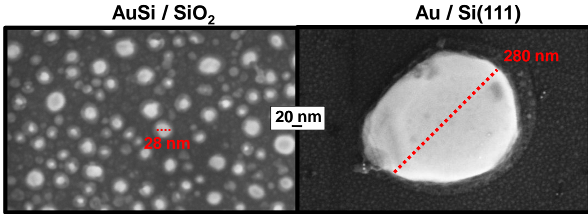
Figure VII.8 – Left : SEM picture of the resulting islands that formed during the experiment presented in section VI.3.1 concerning the 6 ML AuSi deposit on \text{SiO}_2 substrates annealed at 690 K. Right : SEM picture of the resulting islands that formed during a typical experiment with a deposit of 6 ML of Au on a Si(111) surface annealed at 720 K. The scale bar is the same for the two images to highlight the size difference between the two experiments.
