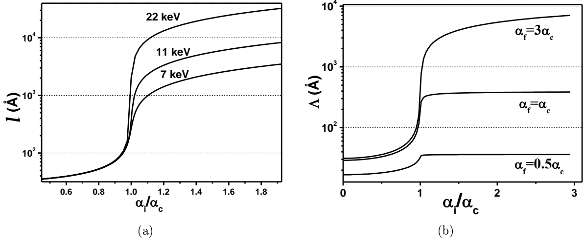
Figure II.2 – Variations of the scattering depth (a) as a function of the incident angle for three different energies, (b) as a function of the incident angle for exit angles equal to half, one and three times the critical angle for a Si surface and an incident wavelength of 1.1 \text{ \AA} ( i. e. 11 keV, \delta = 4.03 \cdot 10^{-6} and \beta = 5.04 \cdot 10^{-8} ).
