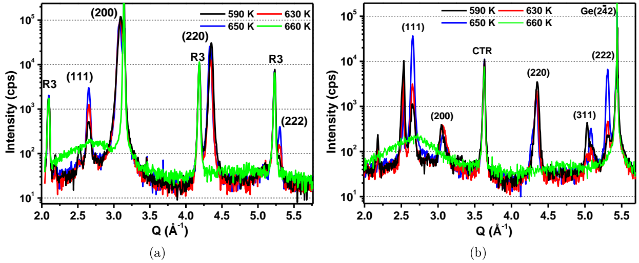
Figure VI.3 – Radial-scans performed upon annealing at 590 K, 630 K, 650 K, 660 K along (a) the Ge[110] azimuth and (b) along the Ge[121] azimuth.
