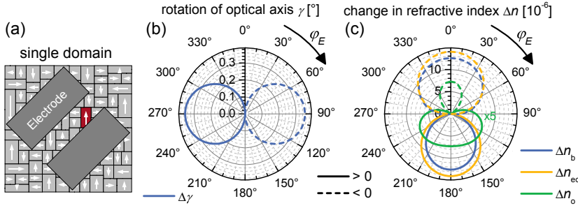
Fig. 3.4 (a) Simulated response for a single ferroelectric domain: (b) Rotation of the optical axis and (c) variation of the birefringence \Delta n_b and the ordinary and extraordinary refractive index \Delta n_o (scaled by \times 5 ) and \Delta n_{eo} , respectively, as a function of the direction of the applied field. Solid and dashed lines correspond to positive and negative values, respectively.
