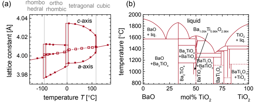
Fig. 2.2 (a) Lattice parameters and crystalline symmetry measured for bulk- \text{BaTiO}_3 at different temperatures. Transitions between the different crystalline phases are indicated by gray lines. Open symbols and the dashed line correspond to calculated values assuming a cubic structure with constant cell volume. All data replotted from ref. [50]. (b) Phase diagram for different compositions of \text{BaO} and \text{TiO}_2 (replotted from ref. [72]). Only the major phases are labeled. The full diagram can be found in ref. [72].
