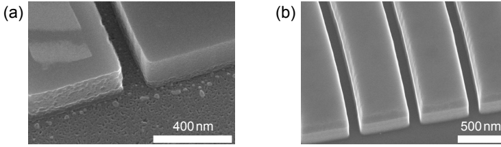
Fig. 4.23 SEM images of grating couplers after etching the top-silicon with HBr. (a) Rough and smooth sidewalls adjacent to each other on the same device due to locally varying plasma conditions with an ICP power of 400 W. Residuals of HSQ are visible on top of the left structure. (b) Smooth side walls when etching with a stable plasma at an ICP power of 800 W. The HSQ layer has not been removed for that sample.
