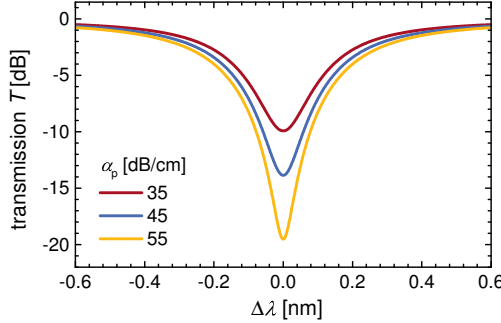
Fig. 4.39 Simulated transmission spectrum for a ring resonator with the same cavity length as the race track resonators shown in fig. 4.37 . The simulations were performed at \lambda \approx 1550 nm for different propagation losses \alpha_p based on the method described in section 4.3.4 . The coupling between the ring and the straight waveguide was set to obtain an extinction ratio of r_e \approx 20 dB.
