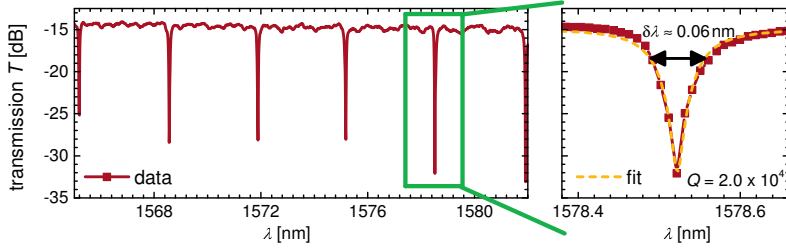
Fig. 4.32 TM-transmission spectrum of a \text{Si}_3\text{N}_4 -slot waveguide ring resonator with r = 30\ \mu\text{m} . Resonances with quality factors of Q = 2.0 \times 10^4 are measured. The width of the resonance \delta\lambda at half transmission ( -3\text{dB} ) is indicated in the right plot.
