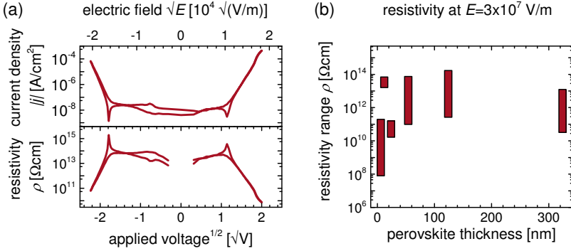
Fig. 2.31 (a) Exemplary j(\sqrt{V}) and resistivity curve of a 8 nm-BaTiO 3 /4 nm-SrTiO 3 /Si sample. The current is normalized to the size of the electrical pad (diameter of 225 μm). (b) Resistivity ranges at the same electric field E = 3 \times 10^7 V/m measured for various MBE-grown samples with different thicknesses d . Samples with d > 100 nm are grown with the hybrid growth approach (section 2.4).
