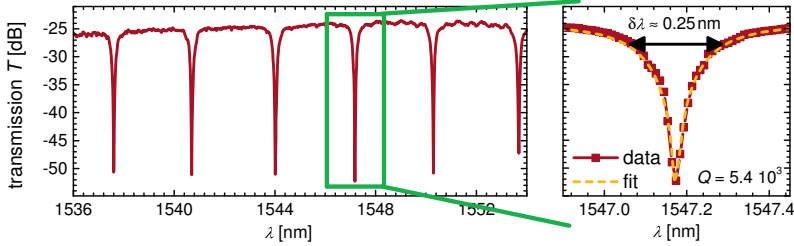
Fig. 4.33 TM-transmission spectrum of a critically coupled BaTiO 3 -slot waveguide ring resonator. The quality factor of the magnified resonance is Q = 5.4 \times 10^3 . The width of the resonance \delta\lambda at half transmission ( -3 dB) is indicated in the right plot.
