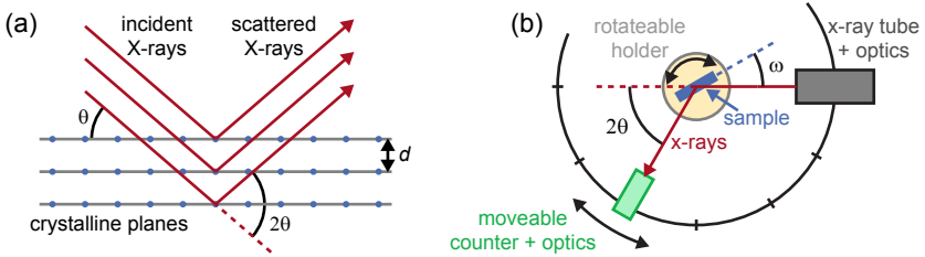
Fig. 2.5 (a) Scattering of x-rays at atoms of different crystalline planes. Since the wavelength of the x-rays is in the same order of magnitude as the distance of the atomic planes d , a diffraction pattern is visible. (b) Illustration of a XRD system (top view).
