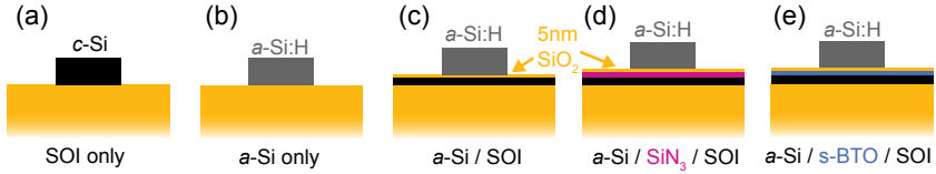
Fig. 4.25 Reference samples fabricated to determine losses (a) in standard SOI waveguides, (b) in FE a -Si:H waveguides, and (c) in PE a -Si:H waveguides. (d) The BaTiO 3 layer is replaced by a 50 nm-thick Si 3 N 4 layer to verify the existence of a TM mode, and to analyze the propagation losses. (e) PE-waveguides samples with sputtered, polycrystalline BaTiO 3 .
