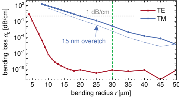
Fig. 4.10 Simulated bending losses for waveguides with HE cross section profile. \alpha_b = 1 dB/cm serves as upper limit when analyzing the bending losses, and is indicated with a dashed gray line. The dashed blue line shows a reduction of the losses by over-etching 15 nm into the BaTiO 3 layer. The dashed green line indicates the design point for active devices ( r = 30 \mu\text{m} ).
