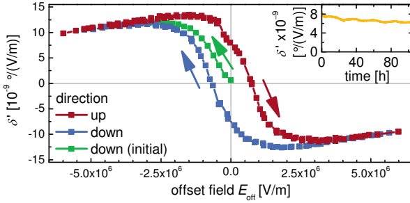
Fig. 3.10 Optical response as a function of the offset field E_{\text{off}} . The data set is collected in three successive loops measured at 25 °C after heating the film above its bulk Curie temperature (green) and sweeping E_{\text{off}} up (red) and down (blue) again. The inset shows the relaxation of the remanent \delta' value at room temperature.
