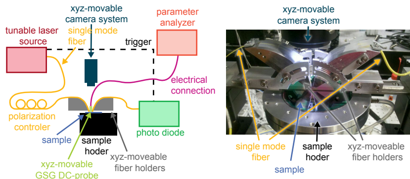
Fig. 4.26 (a) Schematics of the experimental setup for optically characterizing integrated devices. (b) Photograph of the system.
