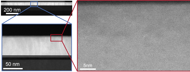
Fig. 2.22 Dark-field TEM images at various magnification levels of a 50 nm thick \text{BaTiO}_3 film grown via shuttered co-deposition. The film is very homogeneous and does not show any pores or islands.
