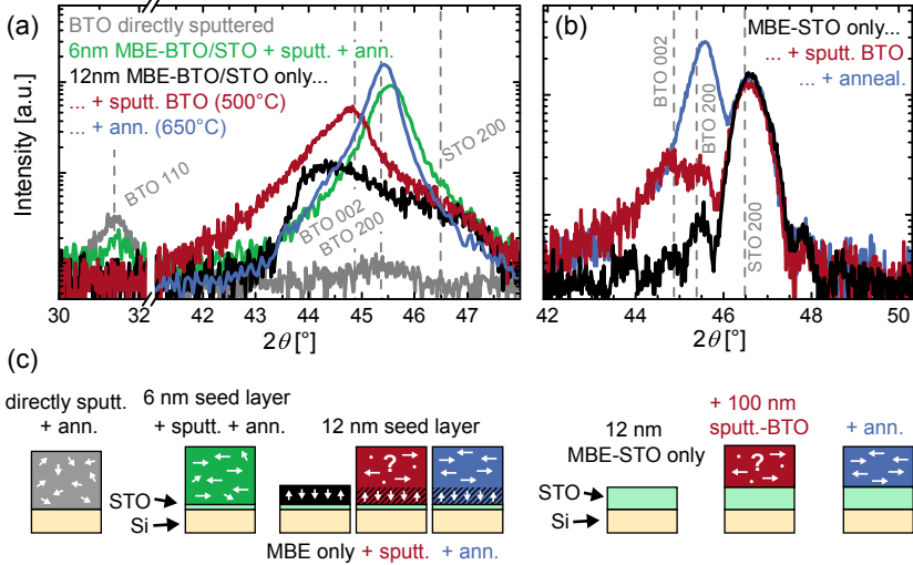
Fig. 2.26 (a) \theta - 2\theta scans of 100 nm BaTiO 3 (i) sputtered-and-annealed on a bare Si substrate (grey), (ii) sputtered-and-annealed on a 2 nm BaTiO 3 /4 nm SrTiO 3 seed layer (green), (iii) sputtered on a 8 nm BaTiO 3 /4 nm SrTiO 3 MBE seed layer at 500 °C (red) and subsequently annealed at 650 °C (blue). The black curve is a 8 nm BaTiO 3 /4 nm SrTiO 3 MBE seed layer only. (b) \theta - 2\theta scans of 100 nm BaTiO 3 sputtered onto a 12 nm MBE-SrTiO 3 seed layer at 500 °C (red) and annealed at 650 °C (blue) (visualized in the schematics). The black curve is the SrTiO 3 seed only. (c) Schematics of the crystalline structure of the samples. The white arrows indicate the orientation of the BaTiO 3 c -axis.
