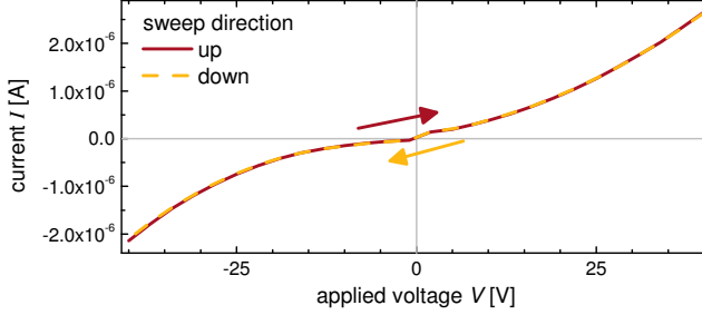
Fig. 3.7 Current-voltage characteristics: Only small currents in the \mu\text{A} range between two electrodes (size \sim 150\text{ }\mu\text{m} \times 350\text{ }\mu\text{m} ) separated by a gap of 7\text{ }\mu\text{m} are measured. In particular, no electric break down is observed.
