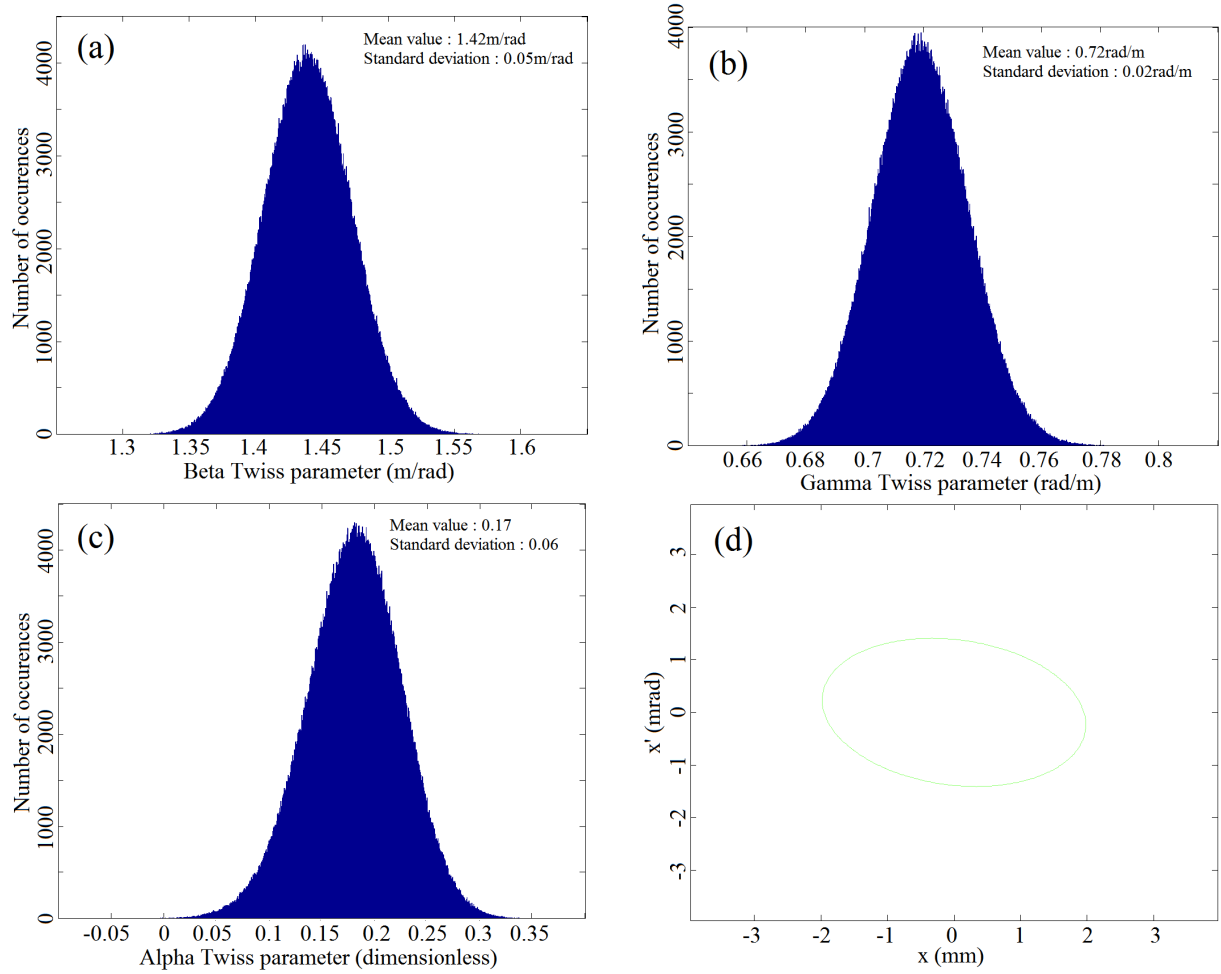
FIGURE 2.10 – Histograms obtained for \beta_y (a), \gamma_y (b) and \alpha_y (c) with the classical 3-screen method in the selected example. Vertical Twiss ellipse obtained (d). Experimental conditions : see Fig. 2.9.
