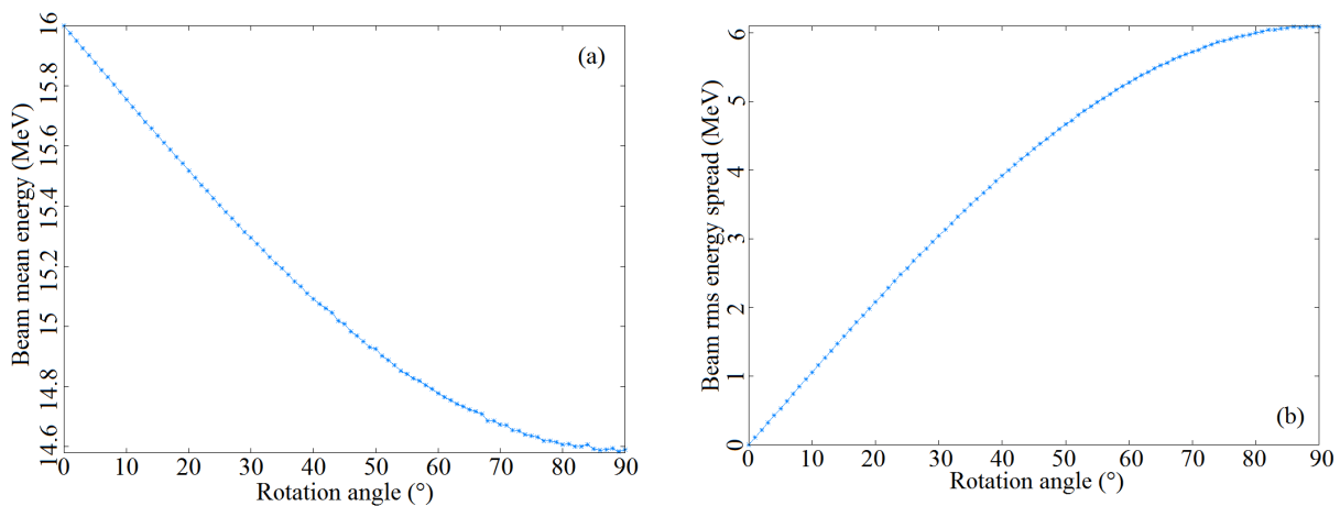
FIGURE 3.46 – Electron beam mean energy (a) and rms energy spread (b), as a function of the angle of rotation in the time/energy phase space, for an initial monokinetic 16 MeV energy distribution with the time profile shown in Fig. 3.45
