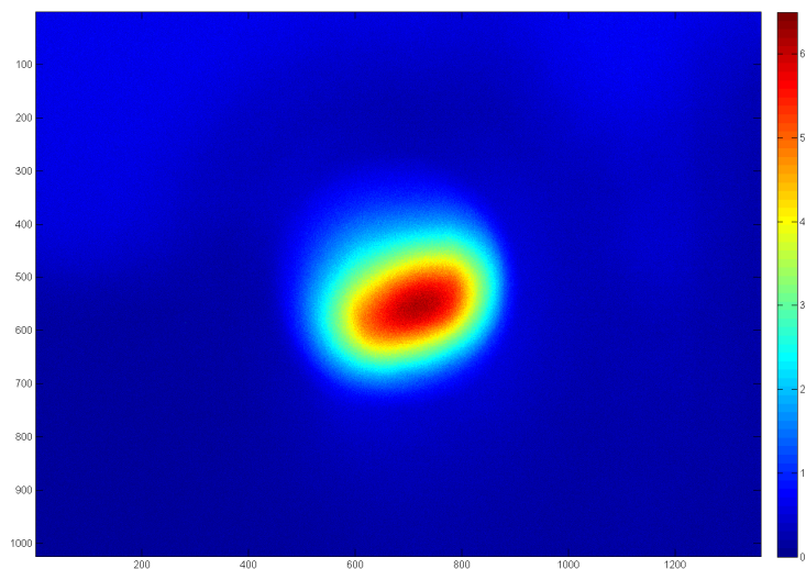
FIGURE 2.50 – Cerenkov radiation measured at the entrance of the streak camera with the Thorlabs mirrors; Conditions : 63 MV/m Gun peak accelerating field; -40^\circ Gun RF-phase ( 0^\circ = maximum of bunch charge); 3.6 MeV bunch energy; 420 pC bunch charge; IB3 = 138 A; IB5 = 44 A; 6.3 \times 4.8 mm 2 CCD pad; Gain 0 of the CCD camera.
