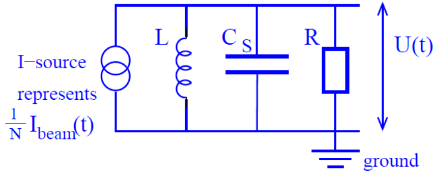
FIGURE 1.12 – Simplified equivalent circuit for the secondary transformer side [43].
