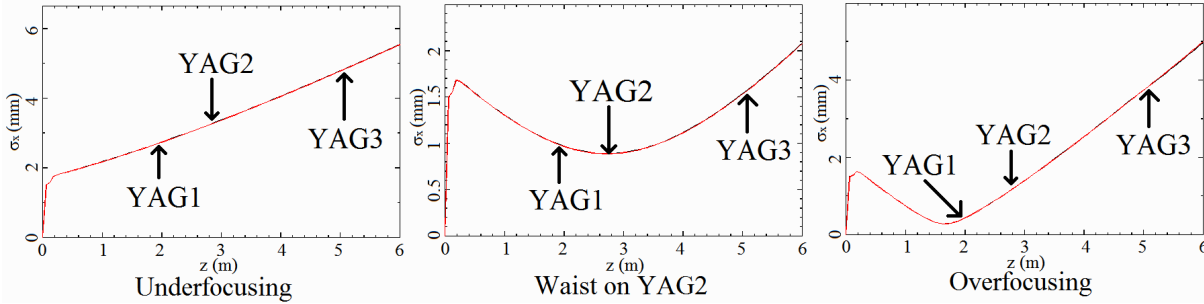
FIGURE 2.8 – The 3 focusing cases studied in ASTRA
