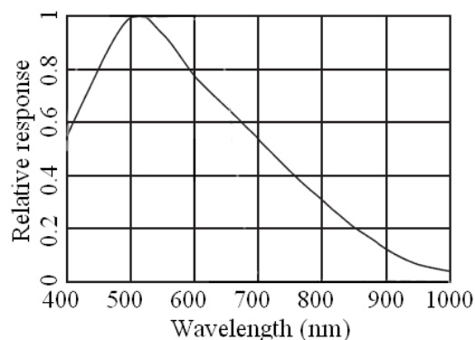
FIGURE 2.45 – Spectral sensitivity of the MatrixVision BlueCougar S-123 CCD camera [80]
