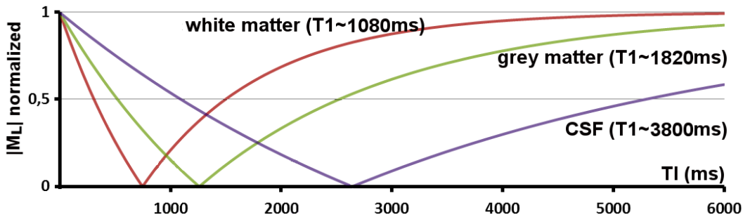
Figure 2.1: Recovery of normalized longitudinal magnetization for tissues with different T1 values in a 3 Tesla magnetic field. The graph shows absolute values of the normalized longitudinal magnetization, as it is measured from the acquired T1 relaxation signal. T1 values for different tissues at 3T were taken from [140].
