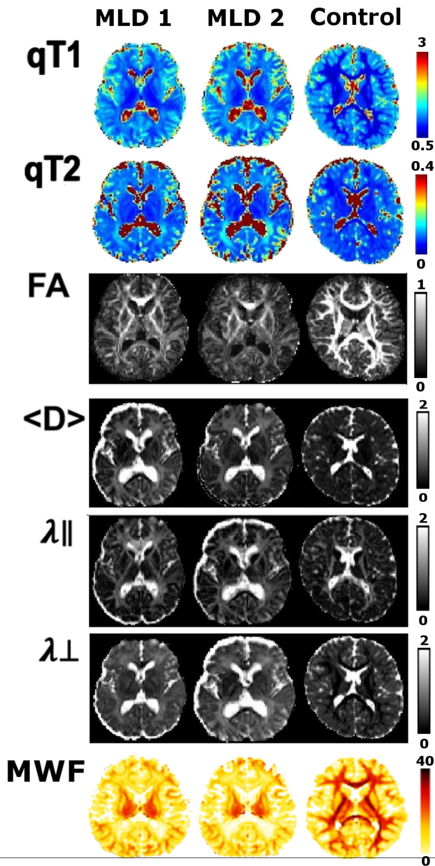
Figure 8.4: Quantitative MRI maps for a typical MLD child (MLD1, 29 months), same child 5 months later (MLD2) and an age-matched control child. qT1 and qT2 values are expressed in seconds, diffusivities ( \langle D \rangle , \lambda_{\parallel} and \lambda_{\perp} ) are given in 10^{-3}\text{mm}^2/\text{s} .
