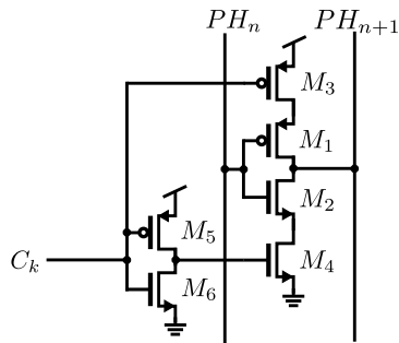
Figure 3.14: Schematic diagram of the fine tuning cells
