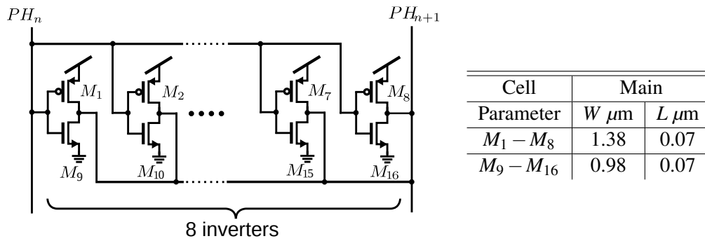
Figure 3.11: Schematic of the main inverter of oscillator: 8 inverters connected in parallel.
