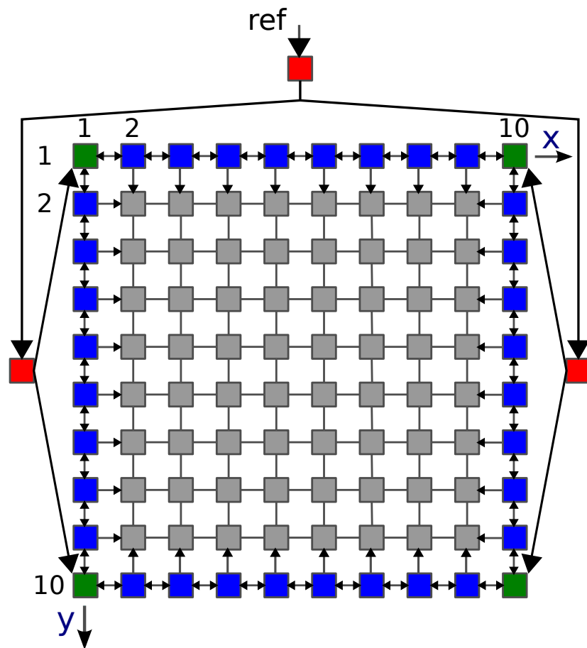
Figure 7.3: Proposed network topology ( \rightarrow : unidirectional; \leftrightarrow , - : bidirectional)
