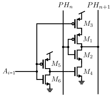
Figure 3.13: Schematic diagram of the additional coarse tuning cells
