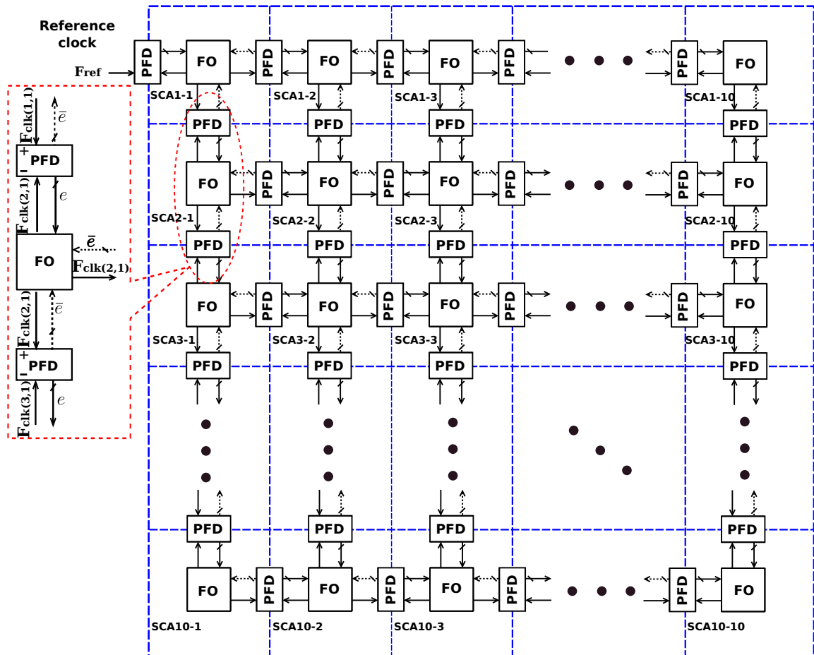
Figure 2.1: Clocking network architecture
