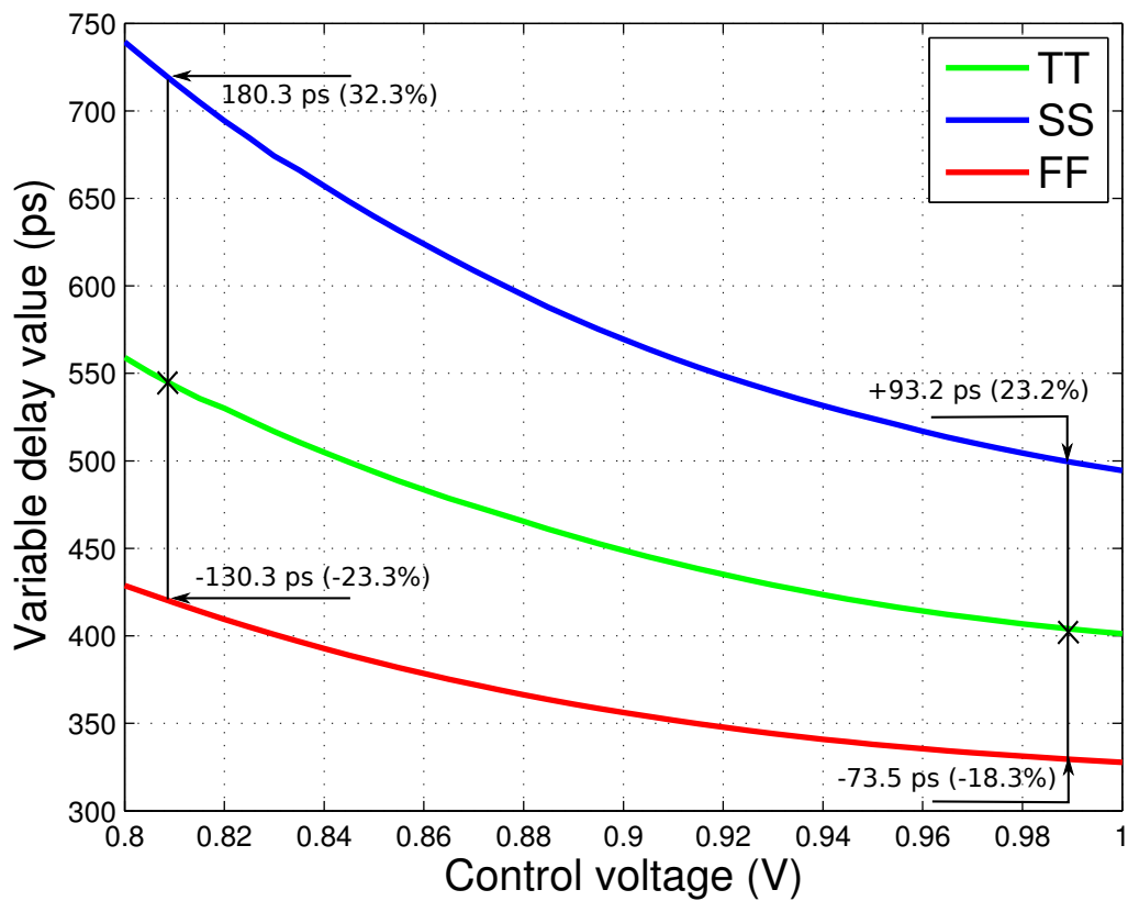
Figure 4.31: Simulated variable delay value versus control voltage in different process corners: process variations: TT, FF and SS
