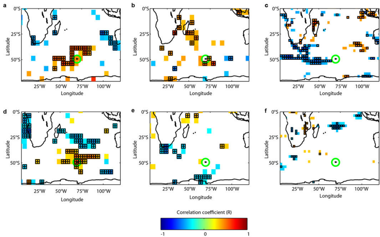
Figure 3. Teleconnections between climate at PAF and conditions in the surrounding oceans. Correlation coefficient (R) is computed between December to March (DJFM) HadSST2 mean Sea Surface Temperature and mean DJFM local atmospheric temperature (a&d) and precipitation (b&e) observed at Kerguelen. c&f) same as previous panels but for correlation between ERA40 precipitation from the pixel including Kerguelen Islands and ERA40 surface latent heat flux during DJFM. Surface latent heat flux is negative when evaporation occurs. Correlation maps are made before 1975 (a, b&c) and after 1975 (d, e&f). All time-series are detrended. Pixels where correlation is significant at 95% are in squared areas, at 90% are in colored areas. Pixels where correlation significance is lower than 90% are not shown. Kerguelen Islands are located inside the green circle.
