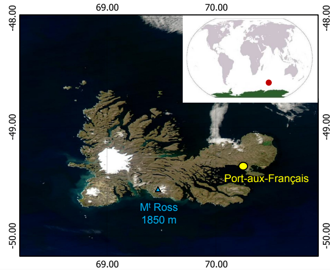
Figure1. MODIS© image of Kerguelen archipelago showing the location of Port-aux-Français station. Location of Kerguelen is shown as a red dot on the global map in the top right corner.
