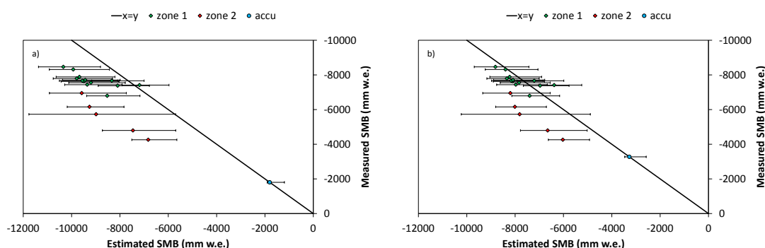
Figure 7. Comparison between field annual SMB measured at stake locations (see Fig. 1 b 1 for locations) and annual SMB estimates. Two cases were used for the computation of SMB : (a) turbulent heat fluxes of 50 \text{ W m}^{-2} and doubled precipitation compared to estimates, and (b) turbulent heat fluxes of 30 \text{ W m}^{-2} and estimated precipitation. Values are separated into zone 1 and zone 2 (see Section 2.1 1 for explanations). The point named "accu" corresponds to the x = y SMB value calculated with the albedo of a pixel situated in the accumulation zone of the glacier (990 m a.s.l.). Error bars were estimated by calculating the error introduced when selecting different pixels adjacent to the one in which the stake is located, plus the systematic bias introduced by using clear-sky images.
