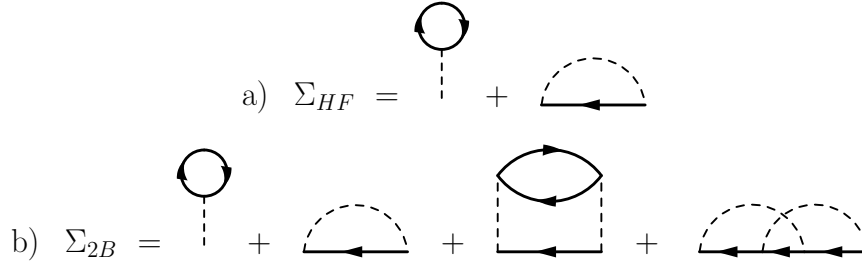
Figure 3.5: Feynman diagram representation of the a) Hartree-Fock and b) second Born self-energies. The bold straight lines represent the interacting 1-GF, the dashed lines the Coulomb potential v_c .
