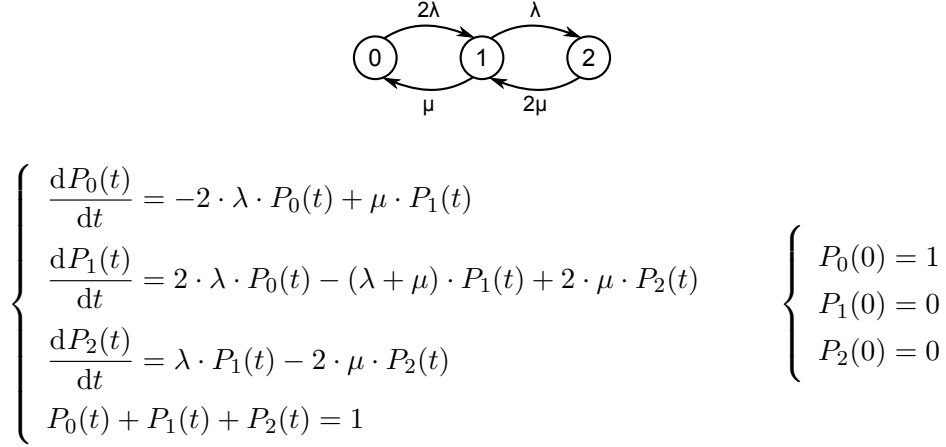
Figure 2.4.: A Markov chain with 3 states, its set of ordinary differential equations, and its initial distribution.
