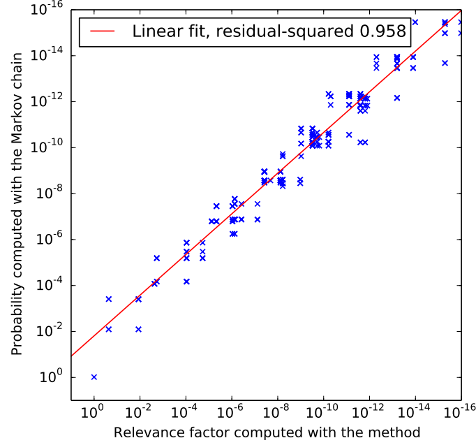
Figure 3.3.: Correlation between the relevance factor computed during the generation of the chain and the probability calculated with the Markov chain for each state of the complete chain for the fault tolerant database, with mission time T = 100 hours.
