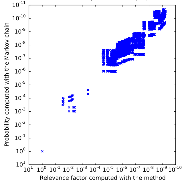
Correlation between the relevance factor computed with the partial generation method and the probability of the state in the Markov chain at mission time, for each state of the partial chain (85,353 states)
