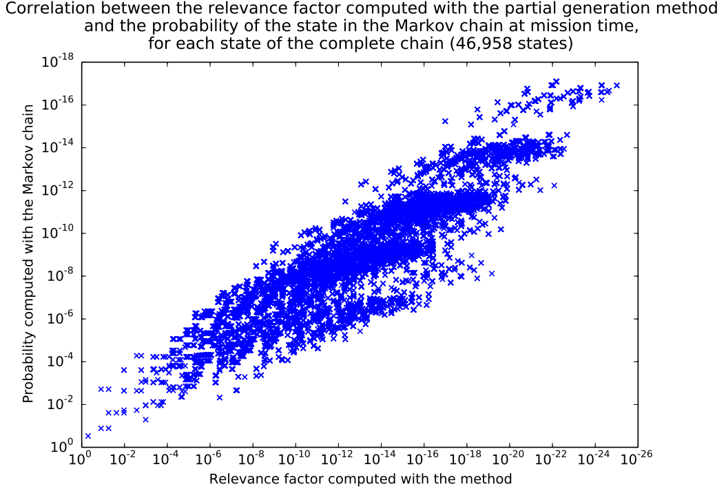
Figure 3.15.: Correlation between the relevance factor computed during the generation of the chain and the probability calculated with the Markov chain for each state of the full chain for the oil production system at mission time T = 130,000 hours.
