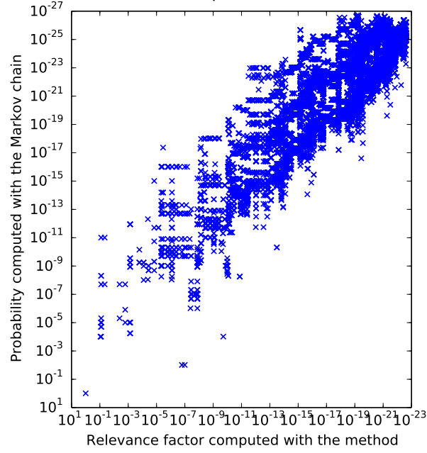
Correlation between the relevance factor computed with the partial generation method and the probability of the state in the Markov chain at mission time, for each state of the partial chain (41,207 states)
