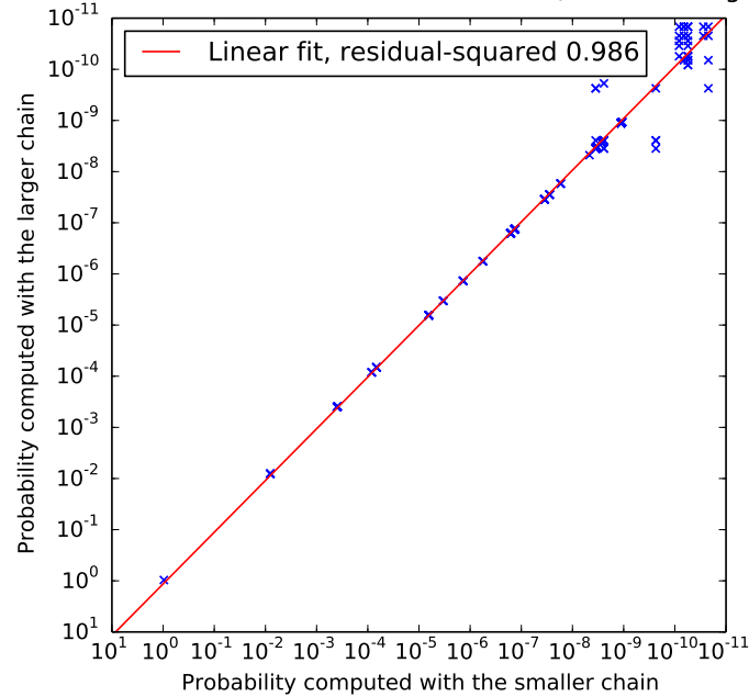
Figure 3.4.: Correlation between the probability of each state of the partial model (threshold \xi = 1,000 transitions) whether they are in the partial chain or in the full chain, for the fault tolerant database, with mission time T = 100 hours.
