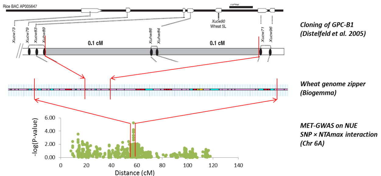
Figure 5: GNY5 and Gpc-B1 are homeologous. The MET-GWAS model was a mixed model K including quality and precocity as covariates, a SNP main effect and an SNP \times NTA max interaction.
