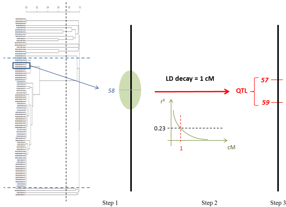
Figure 2: Method that should be tested to define QTL from GWAS result. Step 1: QTN clustering in function of LD ( r^2 ) (method average, cut-off = 1- critical LD). Step 2: Estimation of LD decay around the most significant QTN. Step 3: Creation of QTL boundaries.
