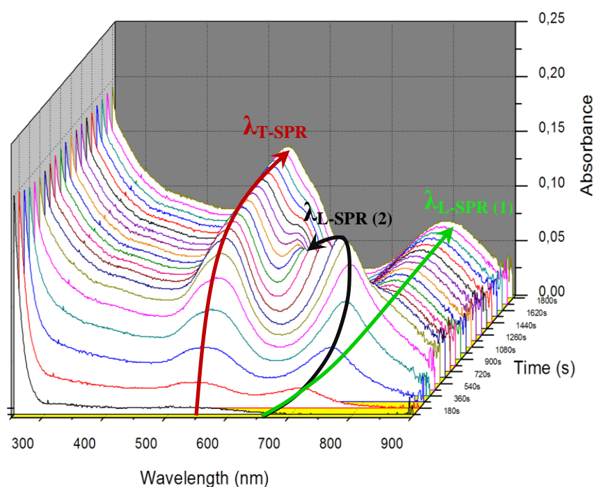
Figure III. 4 Time resolved UV-Vis Spectra of gold NP growth obtained via simultaneous addition of two different types of seeds in growth solution composed of 0.1 M CTAB, 0.5 mM \text{HAuCl}_4 , 0.045 mM \text{AgNO}_3 and 0.75 mM L-Ascorbic Acid
