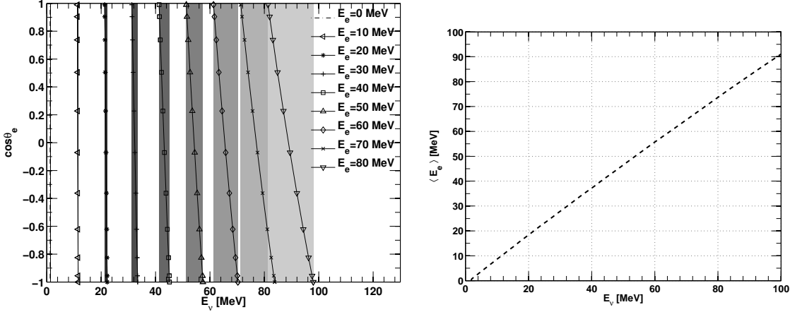
Figure 4.4: Left: Relationship between E_\nu and E_e as a function of the positron emission angle, \cos \theta_e . The gray bands correspond to the range of possible reconstructed neutrino energies for a given positron energy [158]. Right: Average positron energy as a function of the neutrino energy.
