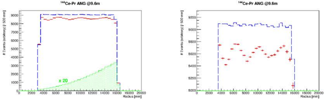
Figure 7.19: Left: Normalized radial distribution of the signal and background in case of non-oscillation (blue) and oscillation (red) and the background (green, enhanced by a factor 20). Each bin content at equidistance to the source is divided by the total scintillator volume at the corresponding distance. Right: Close-up view of the left panel.
