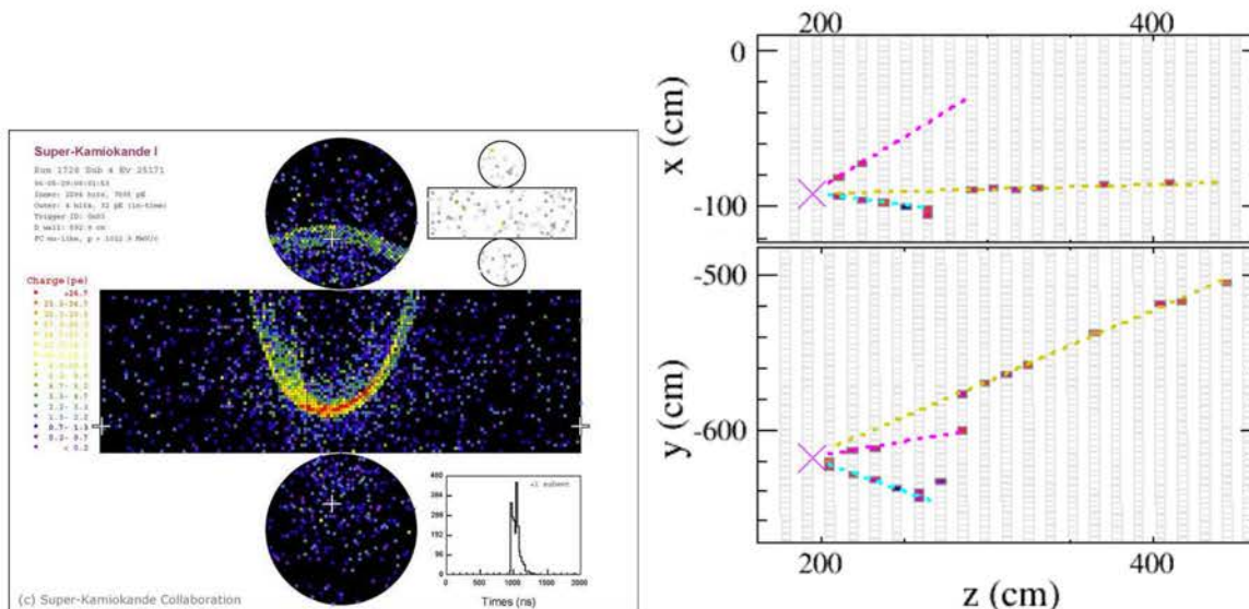
Figure 5.1: Left: Čerenkov ring created by a neutrino-induced muon in Super-Kamiokande [174]. Right: Event display of the first neutrino candidate event selected in the segmented NOνA’s far detector [175].
