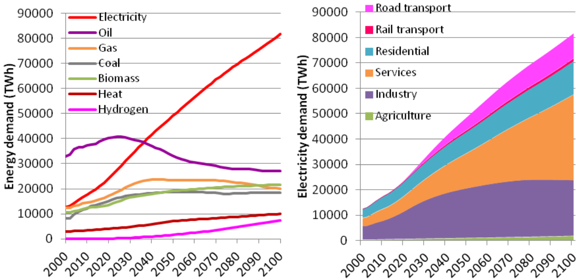
Figure 47: Global energy needs in the baseline scenario; decomposition by end-use fuel (left) and decomposition of electricity needs by sector (right) (POLES+EUCAD).
