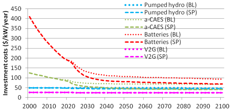
Figure K-4: Investment costs of the four storage technologies, in the Baseline (BL) and the Storage Performance (SP) scenarios (exogenous assumptions).
