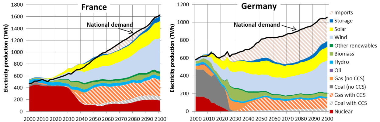
Figure 85: Electricity production in France (left) and in Germany (right). Climate policy scenario (POLES+EUCAD).
