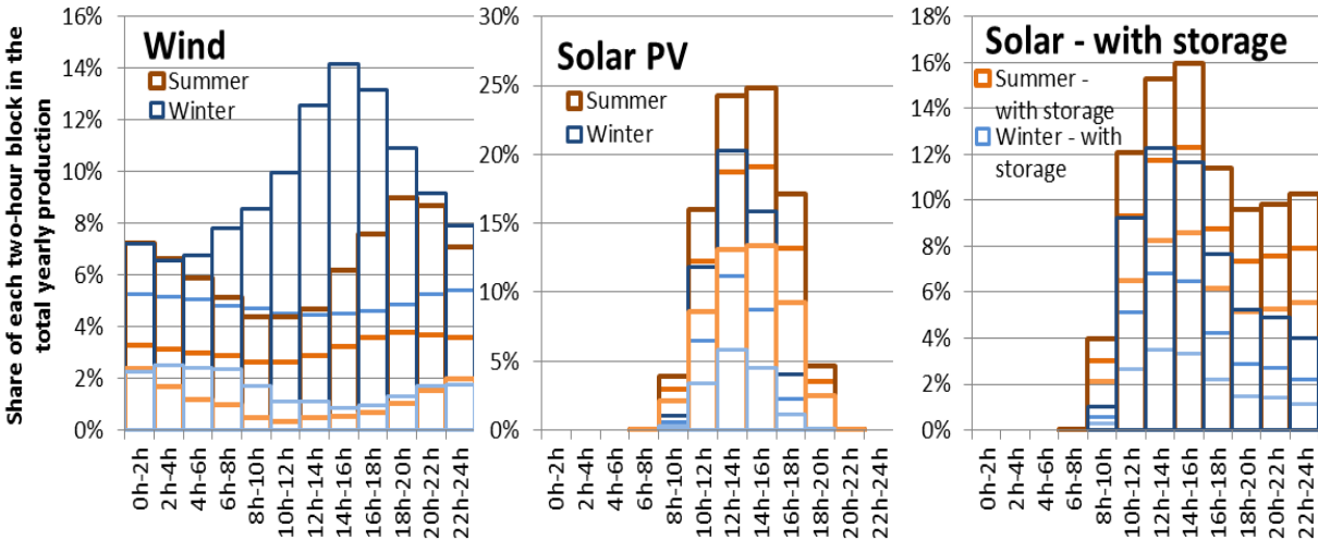
Figure 13: High, medium and low production profiles of wind and solar (photovoltaic or thermodynamic with heat storage); second improvement of POLES’ inputs.
