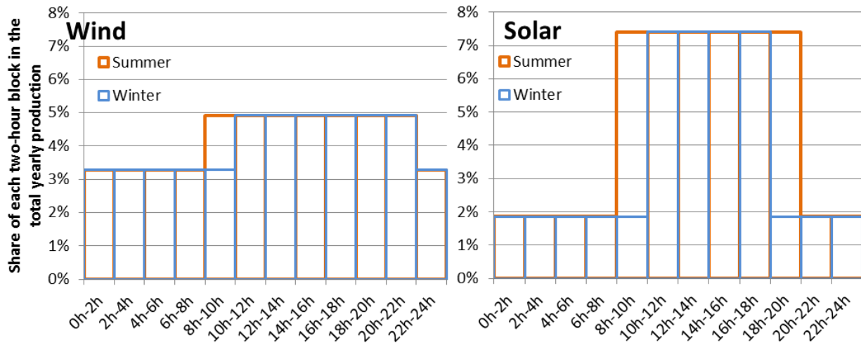
Figure 9: Distribution of wind and solar (centralised) productions across the 24 two-hour blocks (former modelling).
