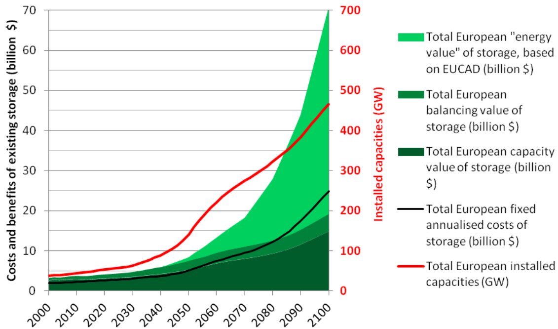
Figure 69: Comparison of the total cost of storage technologies (black line) and the three values identified for storage (green areas). In red is indicated the development of installed storage capacities. European total, baseline scenario (POLES+EUCAD).
