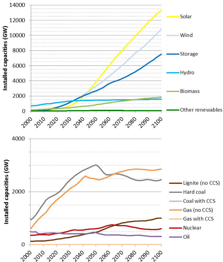
Figure 49: Global installed capacities of the different technologies in the baseline scenario. Renewable and storage technologies on top; fossil fuel and nuclear technologies on bottom (POLES+EUCAD).
