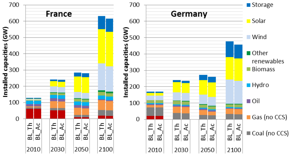
Figure H-10: Installed capacities in France and Germany with 6 typical days based on two calibration methods (with theoretical potential BL_Th and with actual production data BL_Ac); baseline scenario (POLES+EUCAD).
