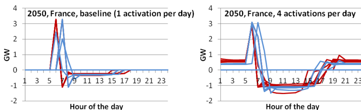
Figure 66: Demand response activation (installed capacity of 3.3 GW), for 1 activation per day (left) and 4 activations per day (right); a positive value indicates a net production. France, 2050, baseline scenario (POLES+EUCAD).
