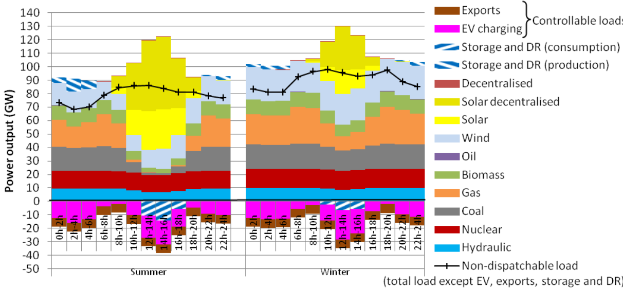
Figure 19: Operation of the power system in the improved POLES. France, 2050, baseline scenario (POLES only).
