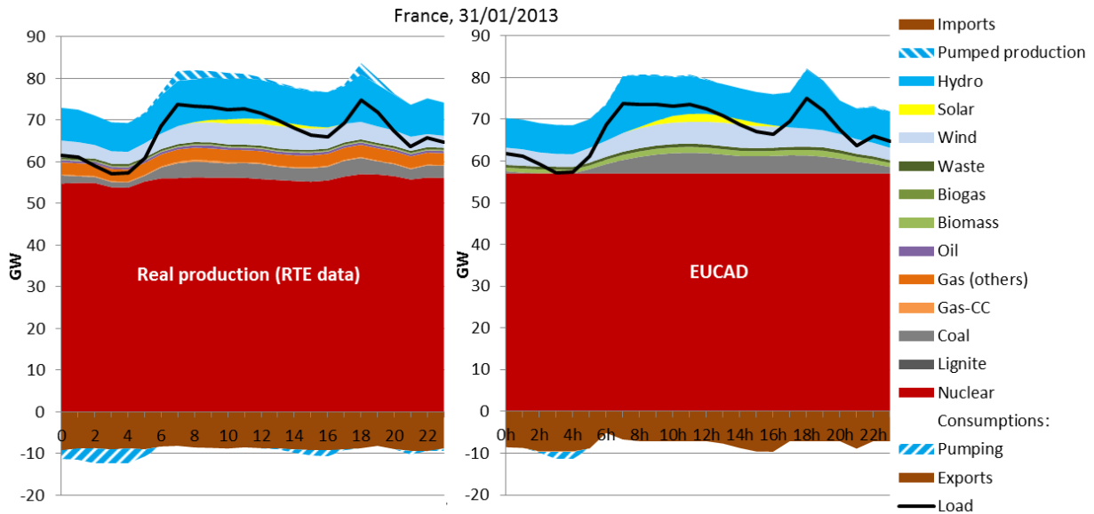
Figure 31: Comparison of the real production data (RTE data; on left) with EUCAD European computation (right). France, 31/01/2013.
