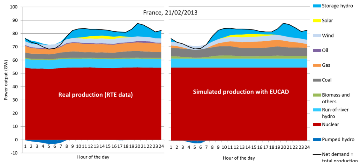
Figure 29: Comparison of the real power plant dispatch (RTE data, left) and EUCAD national computation (right). France, 21/02/2013.
