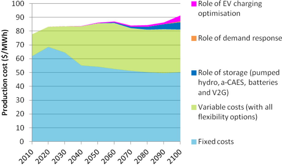
Figure 68: Impact of removing storage, DR and EV charging optimisation on the total European electricity production cost (based on the baseline scenario; POLES+EUCAD).
