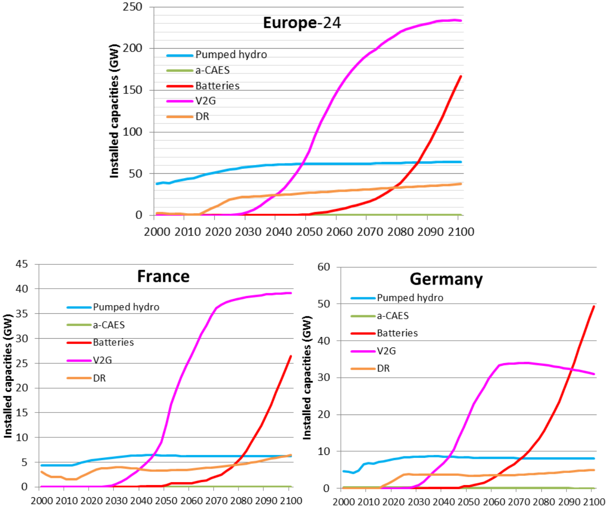
Figure 54: Installed storage and DR capacities for Europe (top), France (bottom-left) and Germany (bottom-right). Baseline scenario (POLES+EUCAD).
