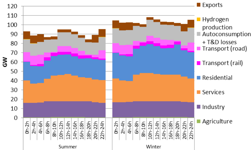
Figure 7: National demand breakdown in consumption sectors. France 2050, baseline scenario (former modelling).
