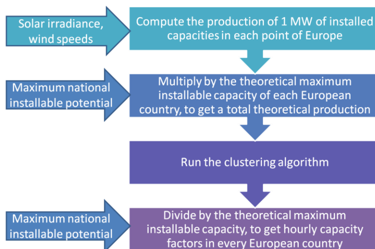
Figure H-3: Diagram of the computation process of the cluster algorithm based on the maximum production potential (based on the 2006 meteorological year).
