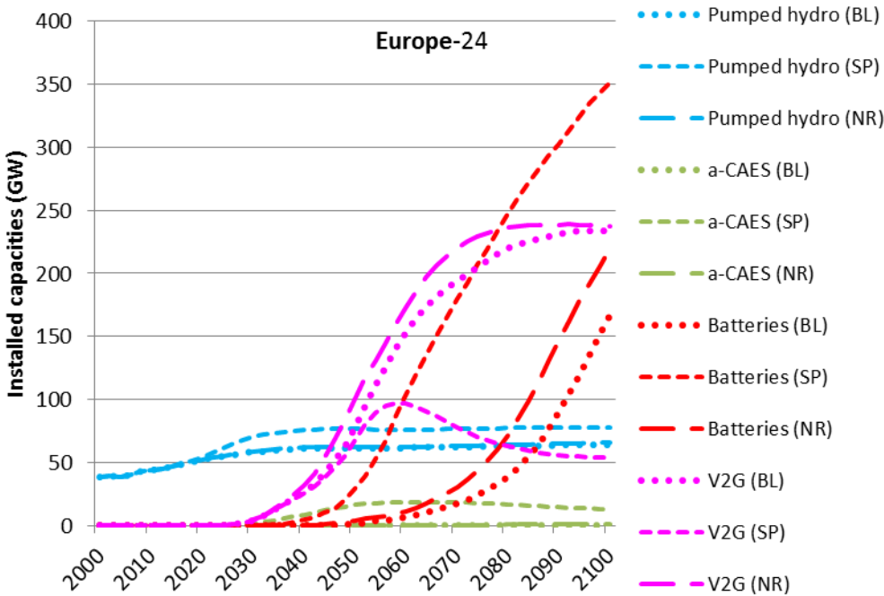
Figure 77: Installed capacities of all storage technologies in Europe for the scenarios Baseline (BL), Storage Performance (SP) and New Renewable (NR) (POLES+EUCAD).
