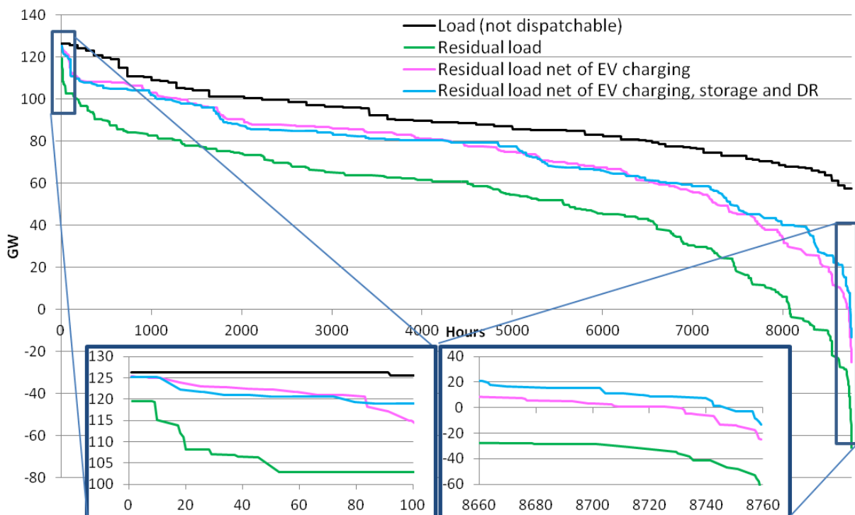
Figure 17: Effect of VRES, EV charging, storage and DR on the load duration curve, zooming on the 100 hours of highest (lower left) and lowest consumption (lower right).
