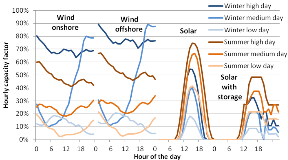
Figure H-2: Wind onshore, wind offshore, solar and solar with storage production profiles, based on assumptions of high, medium and low days of production.
