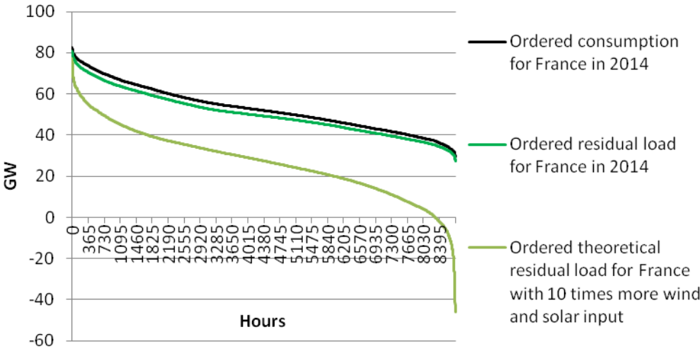
Figure 2: Load duration curve and residual load duration curves for two levels of wind and solar penetration in the French system (2.4% and 24.6%). Source: RTE data for 2014 [17].
