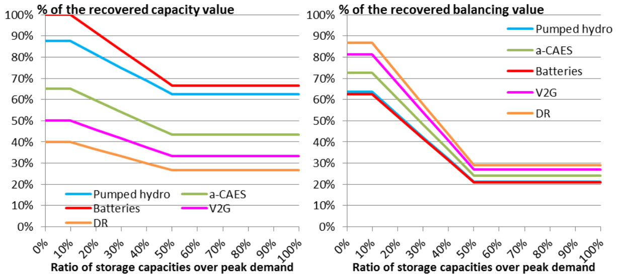
Figure 23: Proportion of capacity (left) and balancing values (right) that storage and DR could recover (modelling assumptions).
