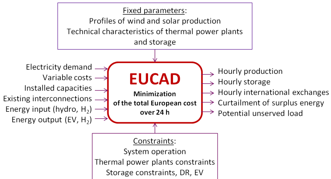
Figure 28: EUCAD diagram (EUCAD stand-alone version).
