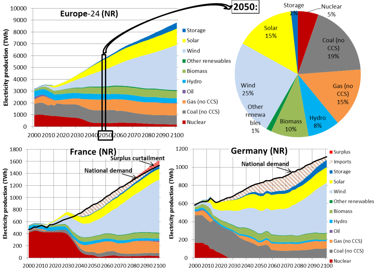
Figure 72: Electricity supply for Europe (top), France (bottom-left) and Germany (bottom-right). New Renewable scenario (POLES+EUCAD).
