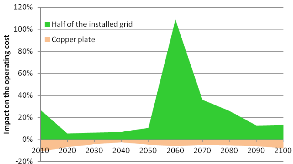
Figure J-4: Impact of the cases with half of the grid capacities and with a perfectly interconnected Europe (copper plate) on the operating cost (based on the baseline scenario)
