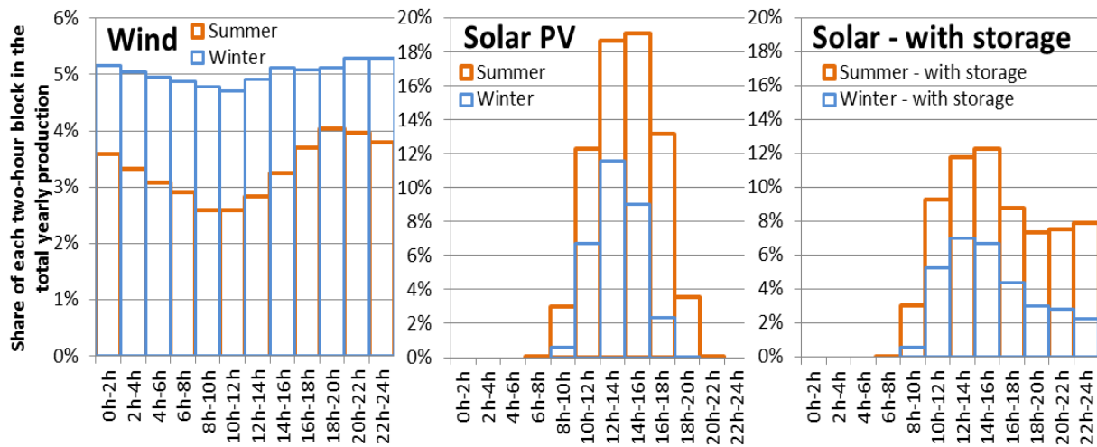
Figure 12: Distribution of wind and solar production (photovoltaic or thermodynamic with heat storage); first improvement of POLES' inputs.
