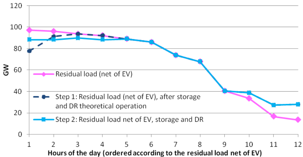
Figure 16: Storage and DR dispatching method, illustrated on a summer day of medium demand, low wind and high solar. France, 2050, baseline scenario (POLES only).
