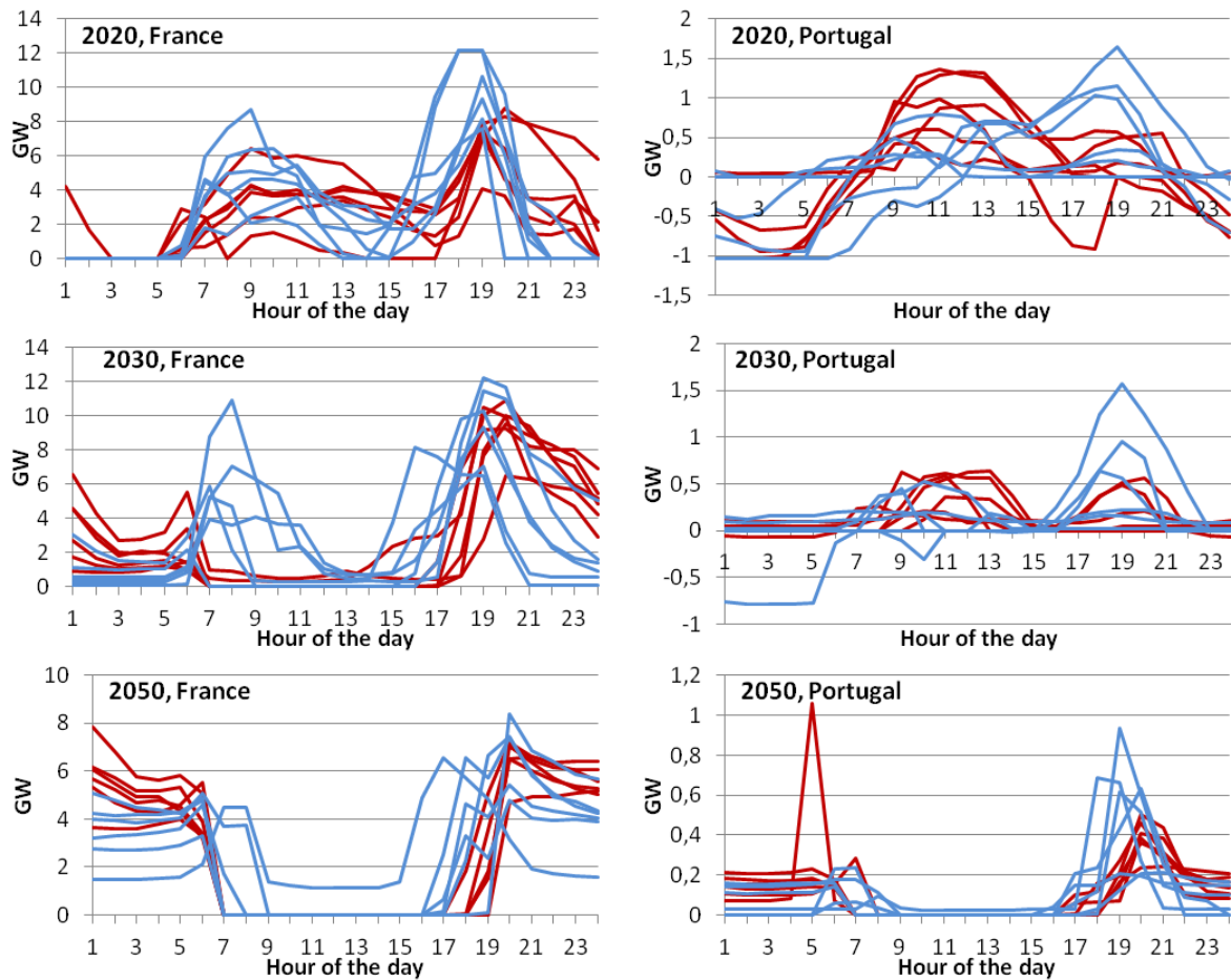
Figure 64: Operation of lakes and pumped hydro for France (left) and Portugal (right), for the 12 typical days (red: summer; blue: winter) of the years 2020, 2030 and 2050. A positive value indicates a production. Baseline scenario (POLES+EUCAD).
