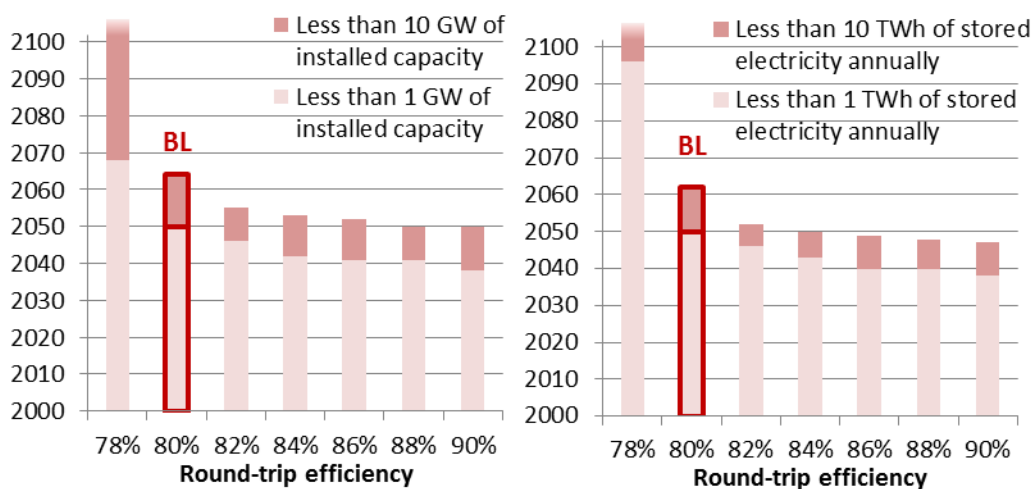
Figure 81: Sensitivity of battery development to the efficiency, in terms of installed capacity (left) and stored electricity (right) in Europe. Based on the baseline scenario (POLES+EUCAD).
