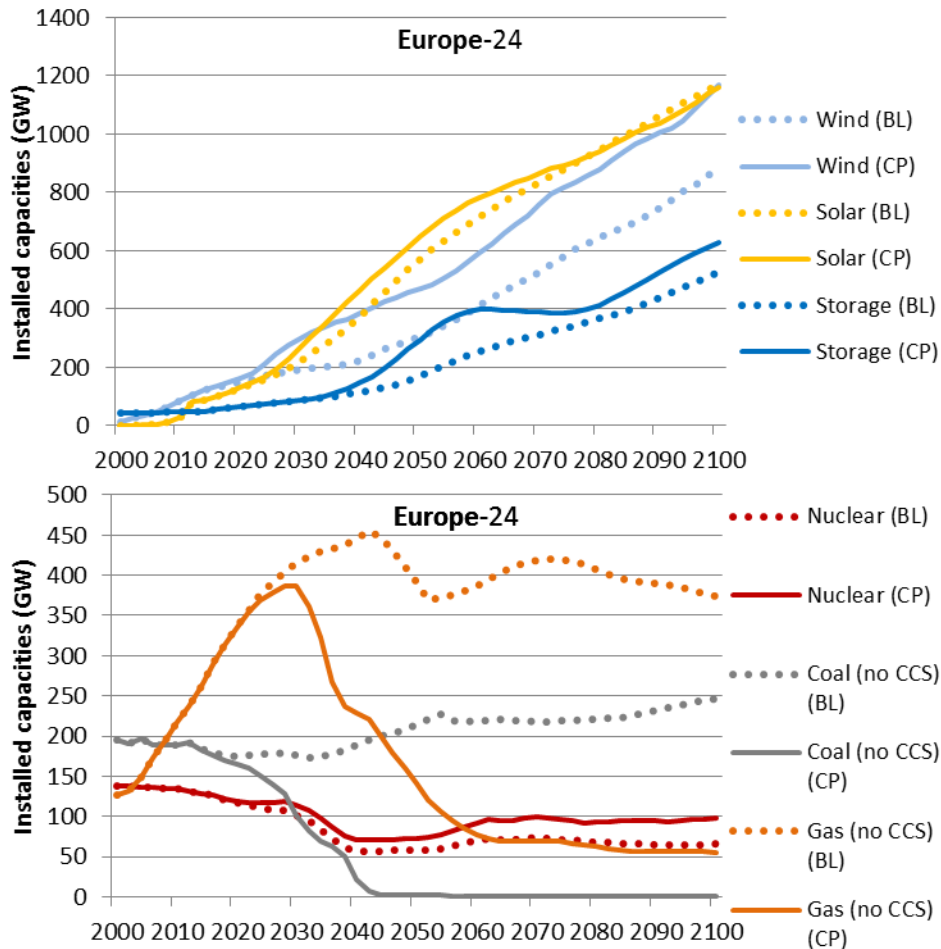
Figure 84: Electricity production capacities in Europe-24, compared between Climate Policy (CP) and Baseline (BL) scenarios (POLES+EUCAD).
