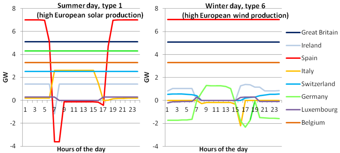
Figure 61: Net imports of France from neighbouring countries. Daily exchanges for 2050, for the type 1-summer day (left) and the type 6-winter day (right); positive values indicate imports, negative values are exports. Baseline scenario (POLES+EUCAD).
