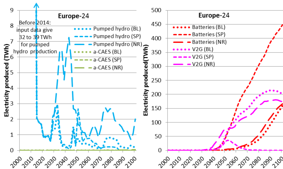
Figure 78: Electricity production of all storage technologies (pumped hydro and a-CAES left, V2G and batteries right) in Europe for the scenarios Baseline (BL), Storage Performance (SP) and New Renewable (NR) (POLES+EUCAD).
