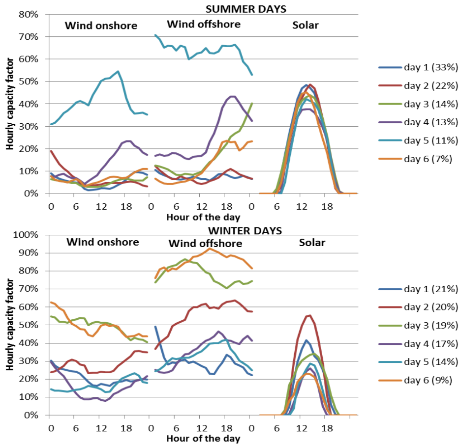
Figure 35: The 12 typical wind and solar production days for France, obtained with the cluster algorithm (summer on top, winter on bottom); the probability of occurrence is indicated in parentheses.
