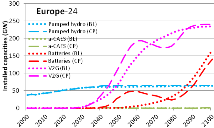
Figure 88: Installed storage technologies in Europe, compared between the Baseline (BL) and the Climate Policy (CP) scenarios (POLES+EUCAD).
