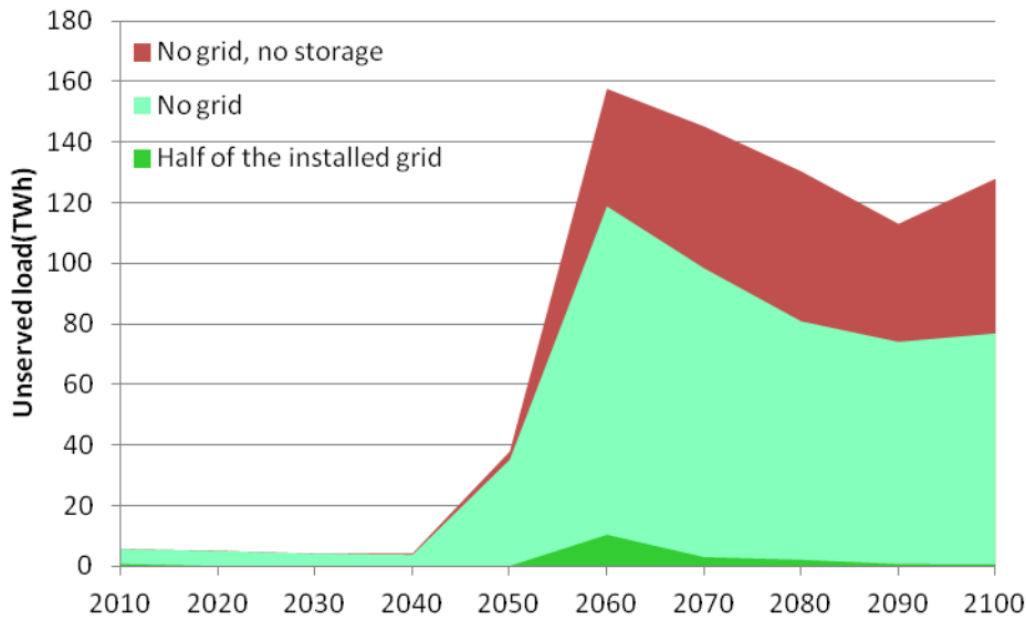
Figure J-2: Unserviced load in Europe in three hypothetical cases, with no grid, with no grid and no storage, and with only half of the installed grid (based on the baseline scenario).
