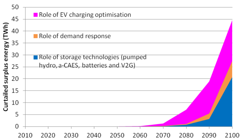
Figure 67: Role of storage, DR and EV charging optimisation in avoiding curtailed surplus energy. Total for Europe, baseline scenario (POLES+EUCAD).
