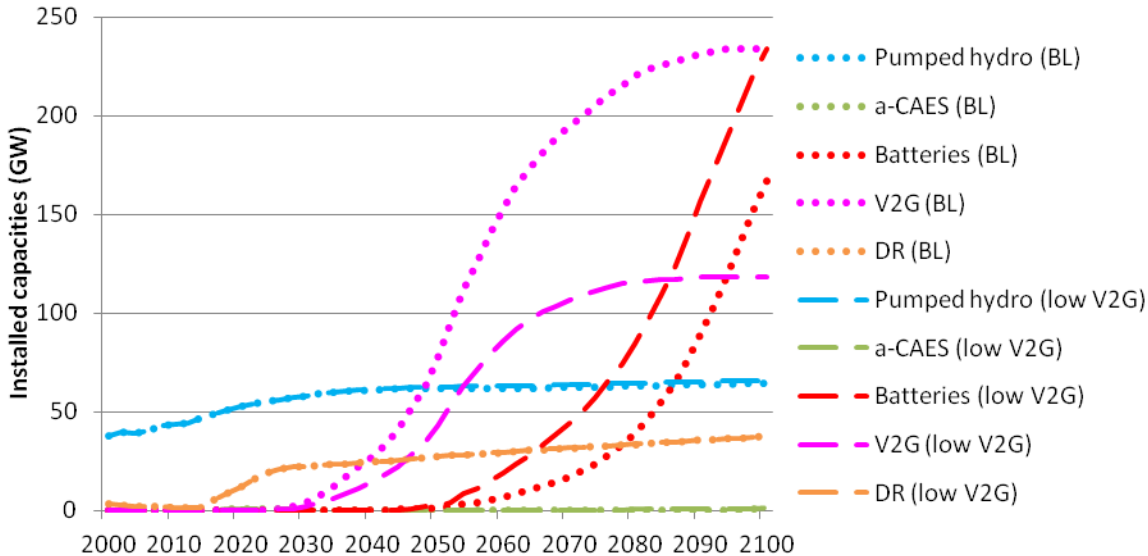
Figure B-1: Comparison of the development of storage and DR in Europe in the baseline scenario (BL) and in a scenario with a maximum installable potential in V2G at half of the baseline potential (low V2G) (POLES+EUCAD).
