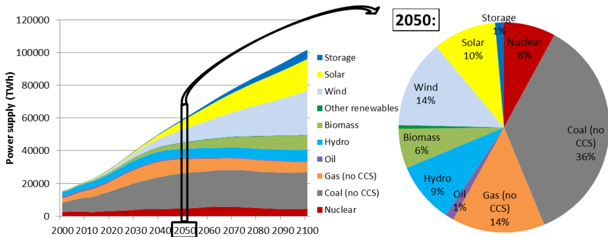
Figure 51: Global electricity supply by energy source in the baseline scenario; time evolution (left) and decomposition for the year 2050 (right) (POLES+EUCAD).
