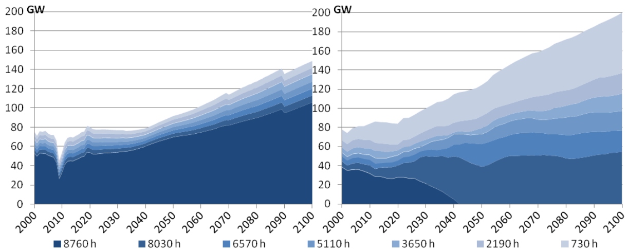
Figure 21: Duration blocks' evolution as expected by the former modelling (left) and the new modelling (right). France, baseline scenario (POLES only).
