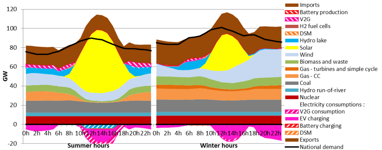
Figure 38: Aggregated dispatch from EUCAD based on high, medium and low production days for wind and solar (9 days per season). France, 2050, baseline scenario (POLES+EUCAD).
