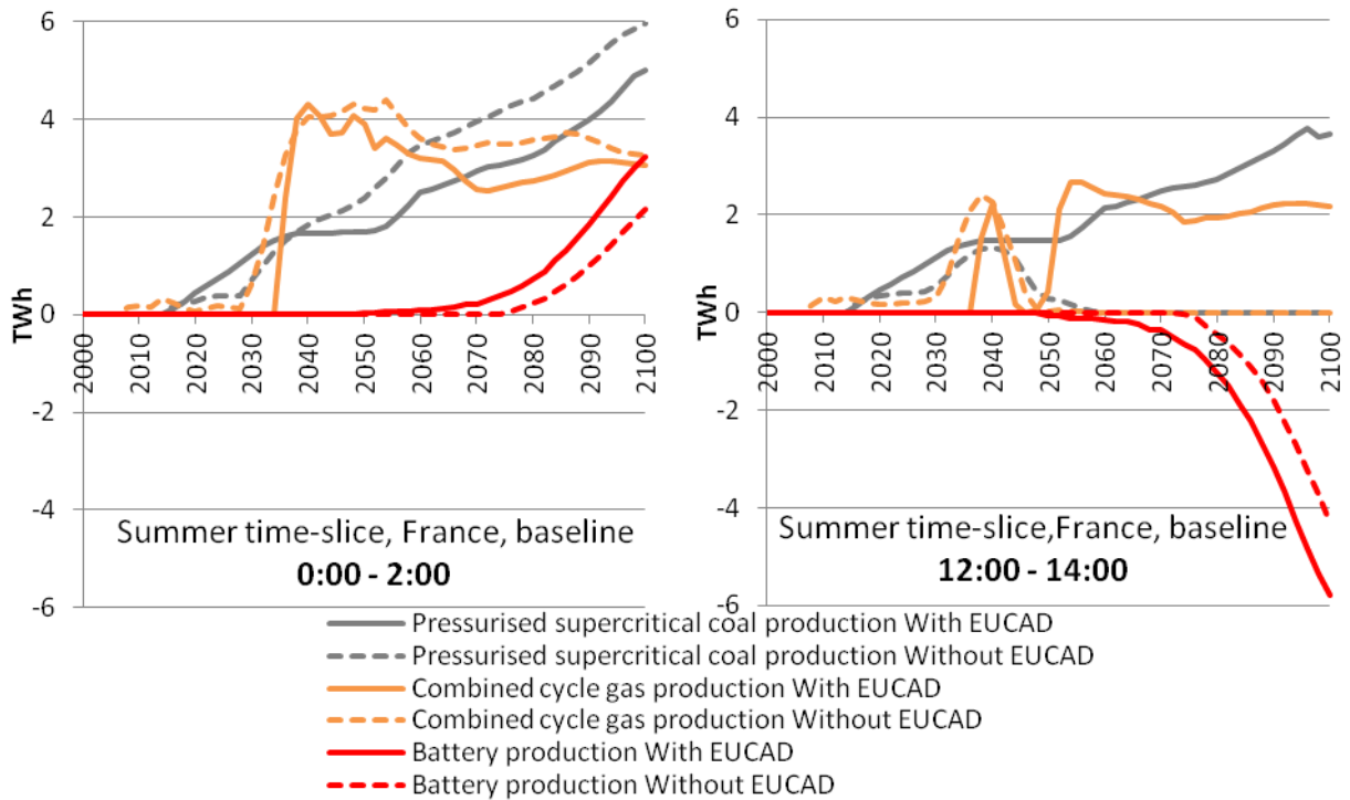
Figure 41: Comparison of coal, gas and storage production (or storage) in POLES only and in POLES+EUCAD. France, baseline scenario (POLES only vs. POLES+EUCAD).
