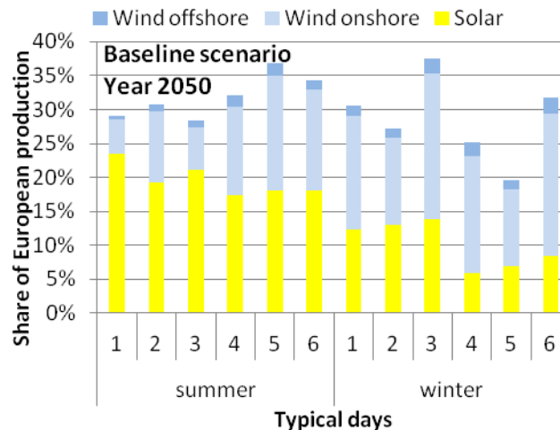
Figure 36: VRES share in Europe electricity production for the 12 typical days obtained with the cluster algorithm. 2050, baseline scenario (POLES+EUCAD).
