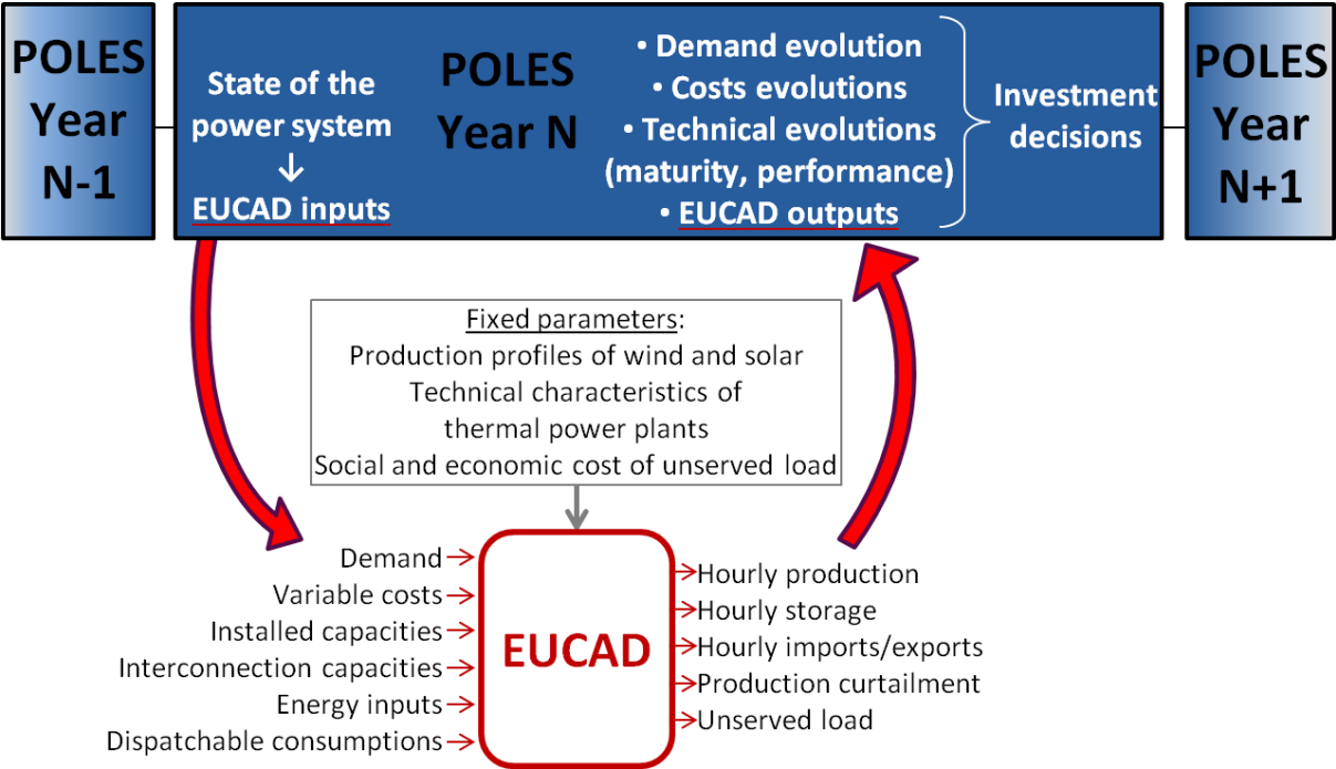
Figure 40: Diagram of the coupling between POLES and EUCAD. This concerns only the power system so the rest of POLES is not represented (see figure 6 for a more general overview of POLES).
