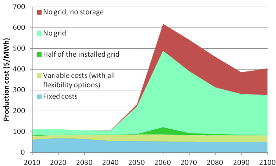
Figure J-3: Electricity production cost in different hypothetical cases (No grid and no storage technologies, no grid, only half of the installed grid capacities, normal use of the grid capacities), based on the baseline scenario.
