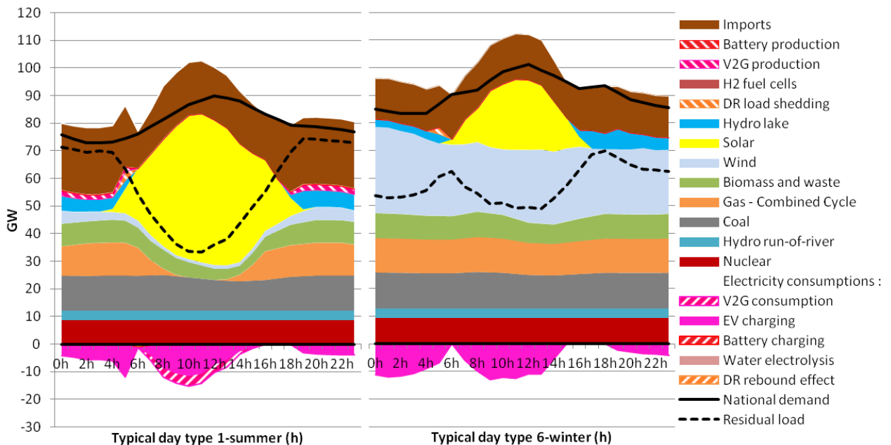
Figure 62: Power system dispatch for France, 2050, baseline scenario (left: type 1-summer; right: type 6-winter) (POLES+EUCAD).
