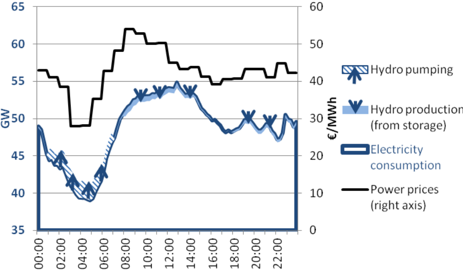
Figure D-1: Hydro pumping operation according to power prices. 15/04/2015, France, RTE data.
