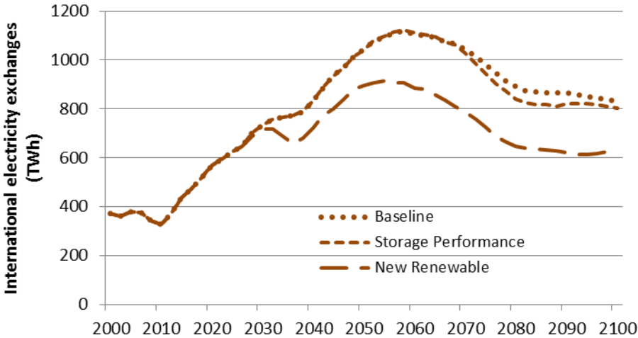
Figure 73: International electricity exchanges in Europe for the scenarios Baseline, Storage Performance and New Renewable (POLES+EUCAD).
