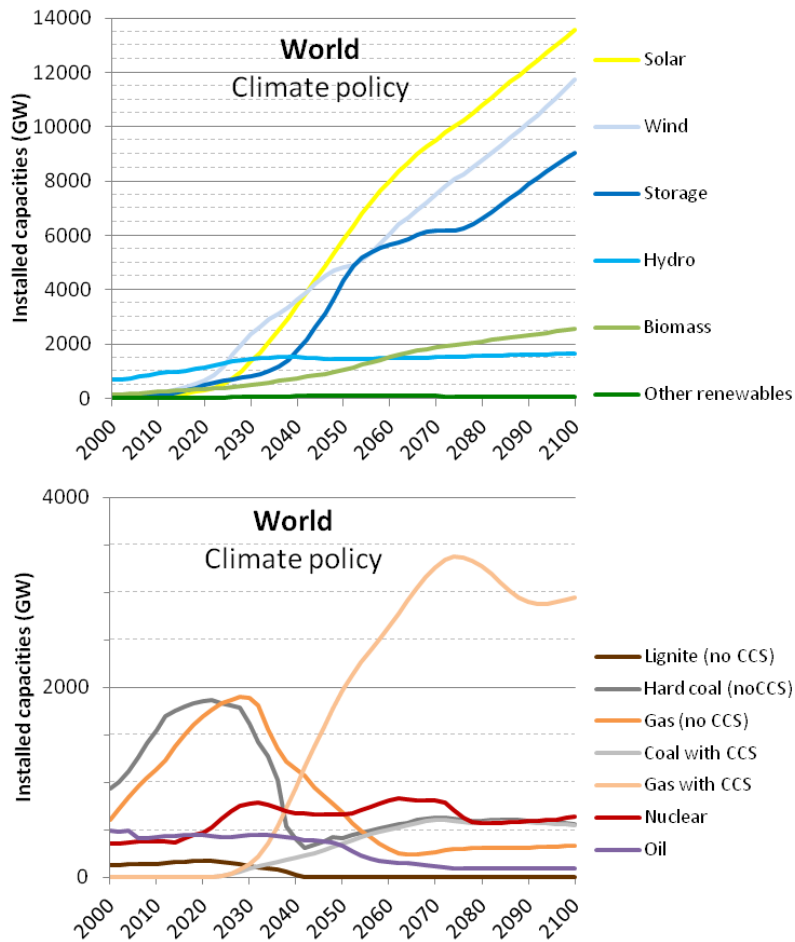
Figure L-3: Global installed capacities of the different technologies in the climate policy scenario. Renewable and storage technologies on top; fossil fuel and nuclear technologies on bottom (POLES+EUCAD).
