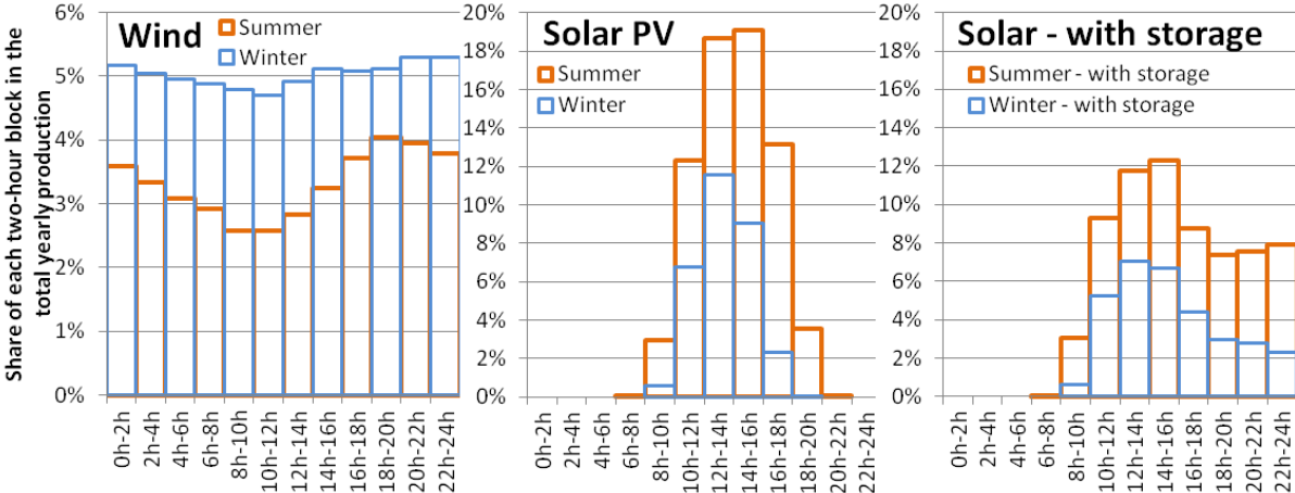
Figure H-1: Wind, solar and solar with storage production profiles, averaged for each two-hour block of POLES (pre-existing POLES modelling).
