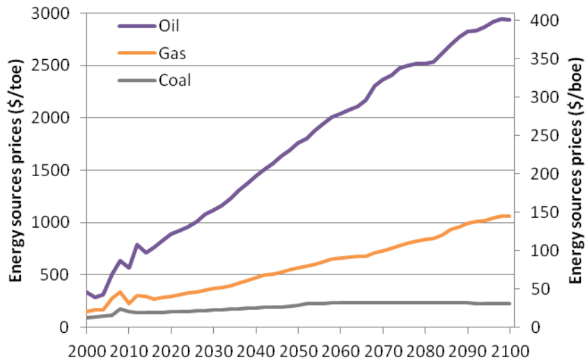
Figure 48: Global oil, gas and coal prices in $2005 per ton of oil equivalent ($/toe, left axis) and in $2005 per barrel of oil equivalent ($/boe, right axis). Baseline scenario (POLES+EUCAD).
