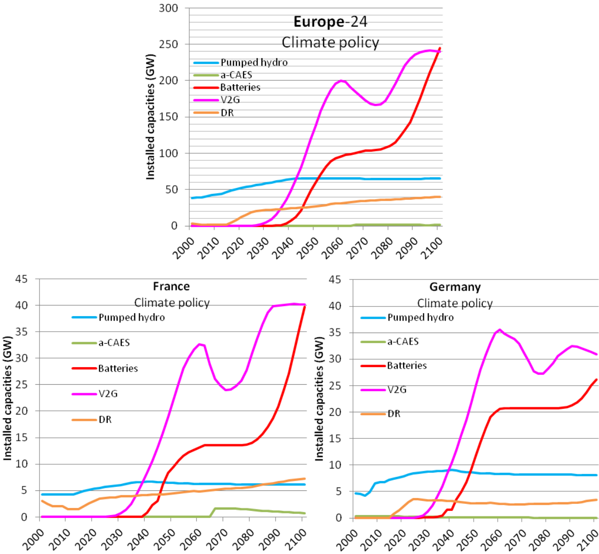
Figure L-5: Installed storage and DR capacities in Europe (top), France (left) and Germany (right), in the climate policy scenario (POLES+EUCAD).
