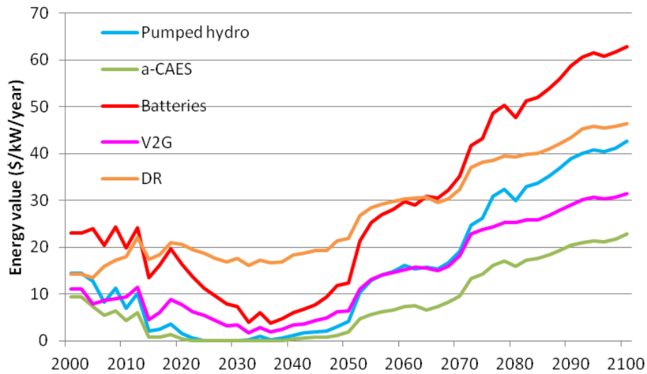
Figure 22: Energy value of a marginal storage as computed in the investment mechanism. France, baseline scenario (POLES only).
