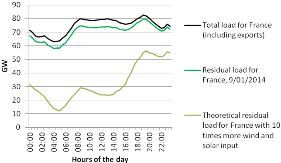
Figure 3: Temporal representation of the residual load for a winter day for two levels of wind and solar penetration in the French system (2.4% and 24.6%). Source: RTE data for January 9 th , 2014 [17].
