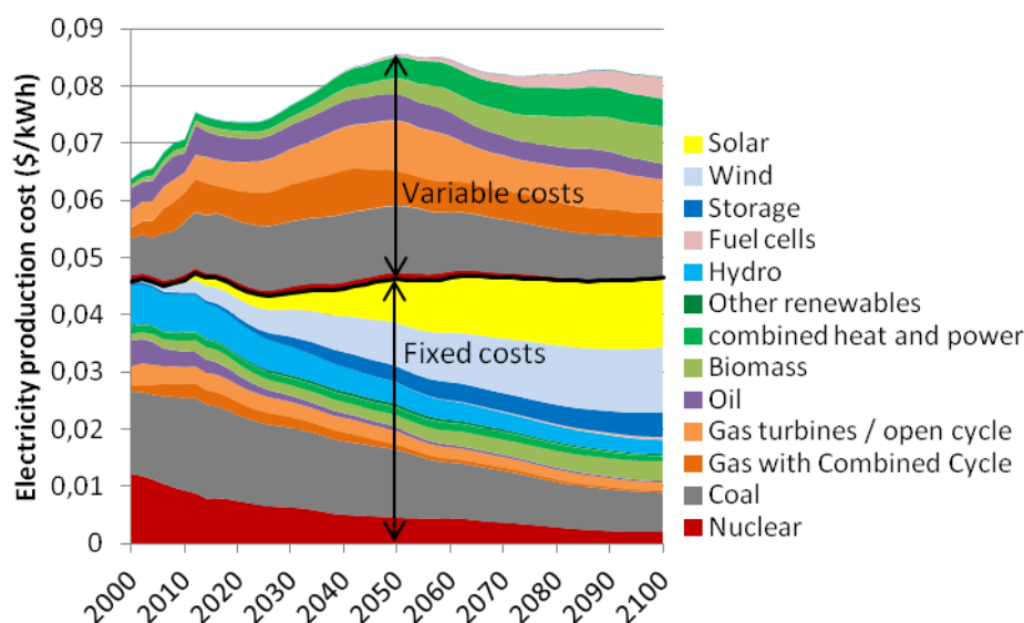
Figure 52: European average electricity production cost, separated in fixed and variable costs for each technology. Baseline scenario (POLES+EUCAD).
