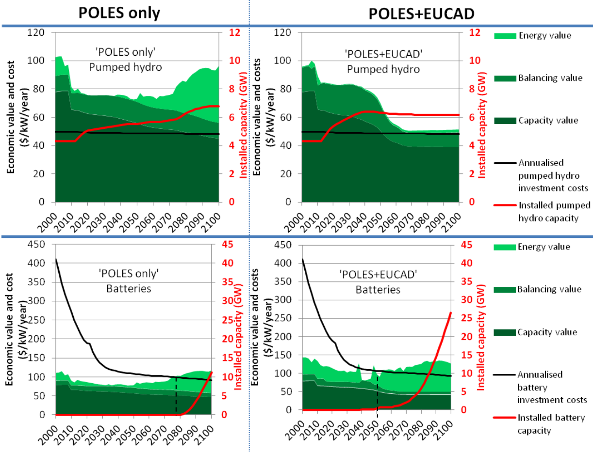
Figure 43: Investment mechanism for pumped hydro (top) and Lithium-ion batteries (bottom), without (left) and with coupling EUCAD to POLES (right). France, baseline scenario (POLES only vs. POLES+EUCAD).
