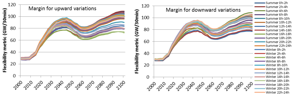
Figure E-1: Flexibility indicator in the upward (left) and downward directions (right) for the 24 two-hour blocks in France. Baseline scenario (POLES+EUCAD).
