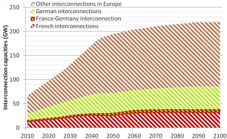
Figure 55: Installed grid capacities in Europe, France and Germany. Baseline scenario (POLES+EUCAD).
