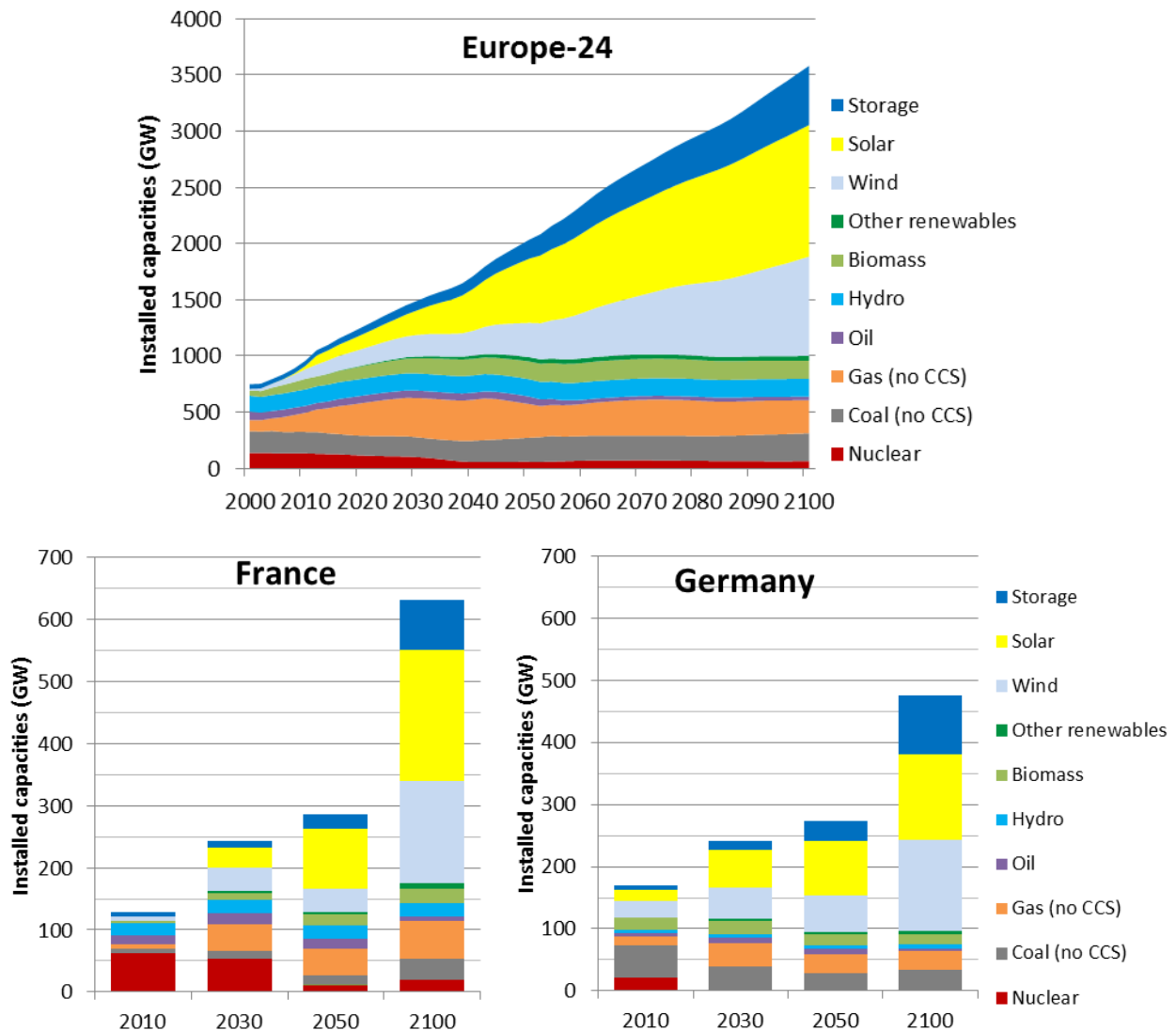
Figure 53: Installed capacities for Europe (top), France (bottom-left) and Germany (bottom-right). Baseline scenario (POLES+EUCAD).
