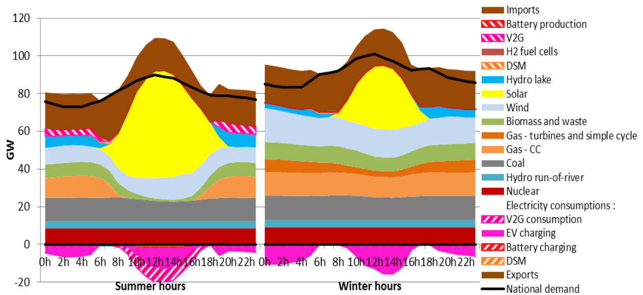
Figure 39: Aggregated dispatch from EUCAD based on 6 clustered production days for wind and solar per season. France, 2050, baseline scenario (POLES+EUCAD).
