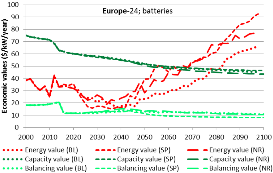
Figure 79: Economic values for batteries (energy, capacity and balancing values), averaged over Europe, for the scenarios Baseline (BL), Storage Performance (SP) and New Renewable (NR) (POLES+EUCAD).
