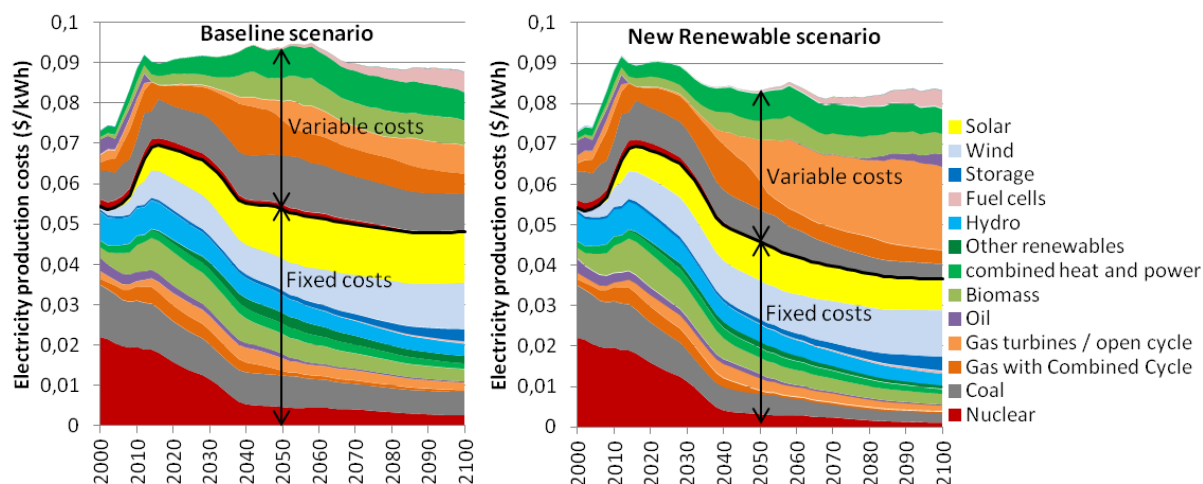
Figure 74: Average European cost structure in the Baseline (left) and in the New Renewable scenario (right) (POLES+EUCAD).
