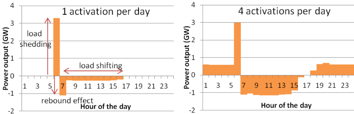
Figure 27: Example of DR production and consumption profile, as computed by EUCAD, with one activation per day (left) and four activations per day (right). France, one of the summer days, 2050, baseline scenario (EUCAD output).
