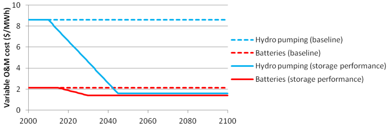
Figure K-3: Evolution of the variable O&M costs for the Storage Performance scenario, compared to the Baseline scenario (exogenous assumptions).
