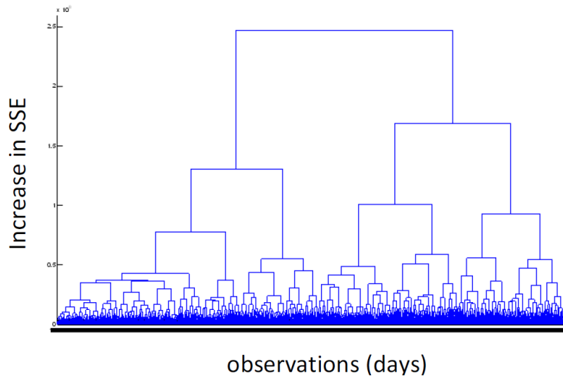
Figure 34: Dendrogram of the clustering algorithm showing the consecutive grouping of two clusters to a joint cluster and the resulting increase in the overall sum of squared errors (SSE, y-axis). All days (x-axis) are consecutively grouped together until only one cluster is left [133].
