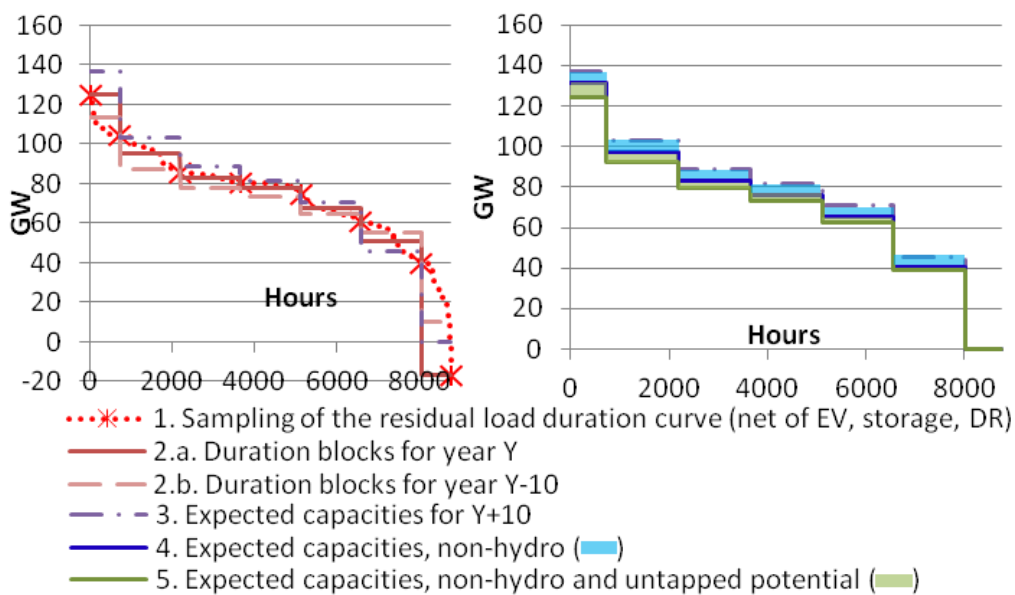
Figure 20: left : definition of the investment blocks based on the residual load duration curve (net of EV, storage and DR); right : the three steps of the investment mechanism (hydro, technologies with potential reached, others). France, 2050, baseline scenario (POLES only).
