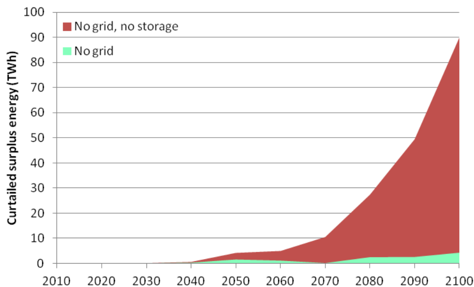
Figure J-1: Curtailed surplus energy in Europe in two hypothetical cases, with no grid and with no grid and no storage (based on the baseline scenario, which has no surplus energy).
