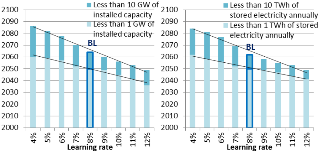
Figure 82: Sensitivity of battery development to the learning-by-doing coefficient, in terms of installed capacity (left) and stored electricity (right) in Europe (based on the baseline scenario; POLES+EUCAD).
