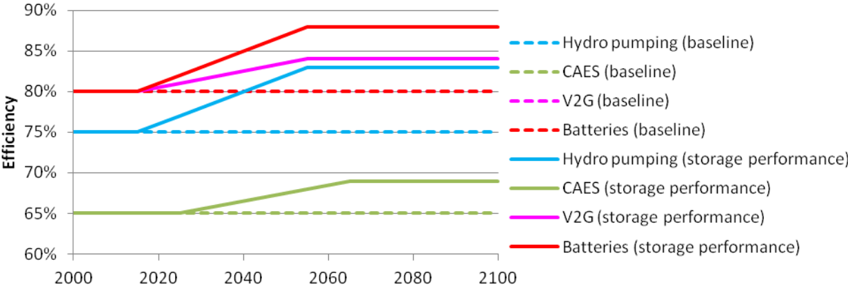
Figure K-1: Efficiency improvements of the Storage Performance scenario (exogenous assumptions)
