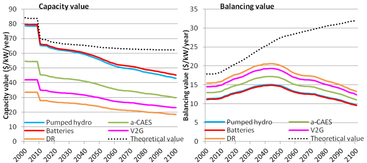
Figure 24: Capacity (left) and balancing value (right) of storage and DR technologies as computed in the investment mechanism. The dotted line indicates the total theoretical value. France, baseline scenario (POLES only).
