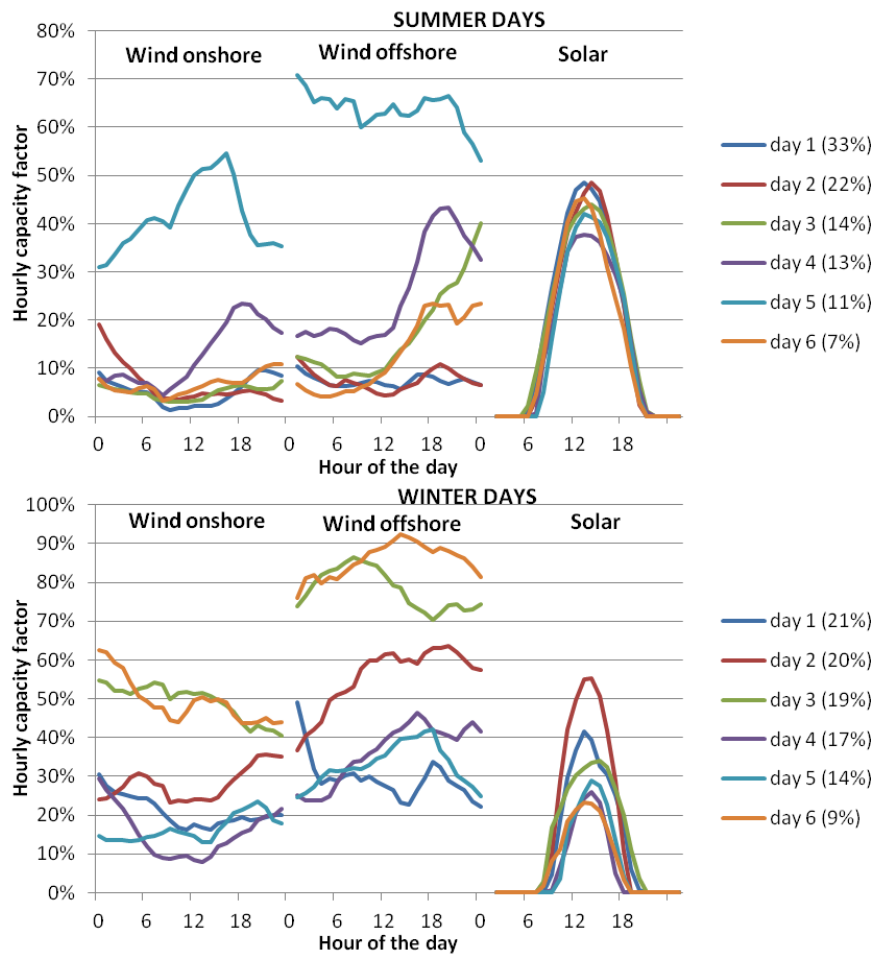
Figure H-4: Wind onshore, wind offshore and solar production profiles in France for six typical days per summer or winter season, based on clusters of the maximum production potential (based on 2006 meteorological data).
