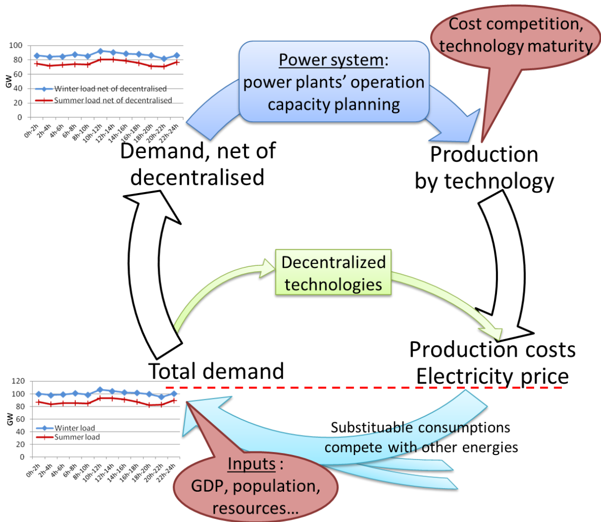
Figure 8: POLES power system diagram
