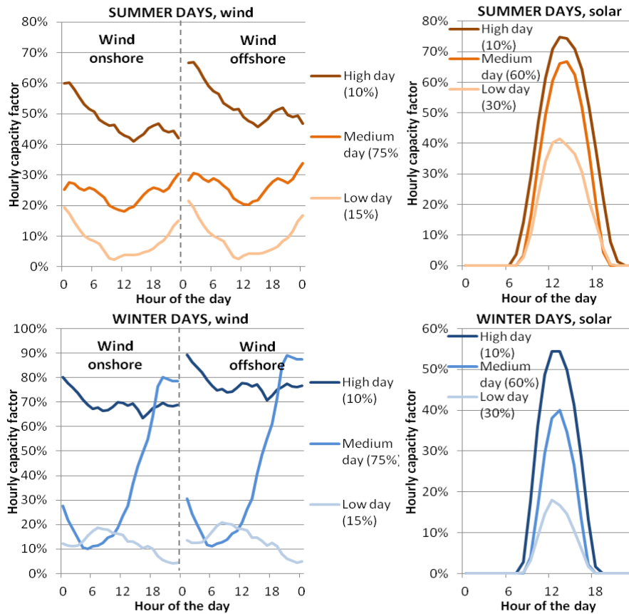
Figure 33: Three typical days of wind (left side) and solar (right side) production per season (summer on top, winter on bottom), with the probability of occurrence in parentheses.
