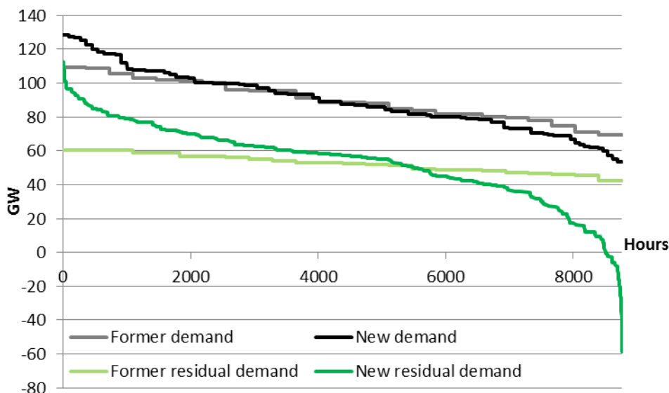
Figure 14: Load duration curve and residual load duration curve: former modelling (applied to the same scenario and year) and new modelling integrating the variability of demand and VRES. France, 2050, baseline scenario.
