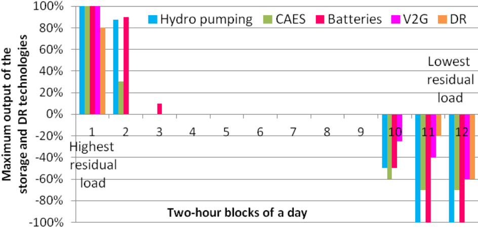
Figure C-1: Assumed maximum use of storage and DR for the 12 two-hour blocks of a day. A positive value indicates a production; a negative value indicates consumption (POLES only).
