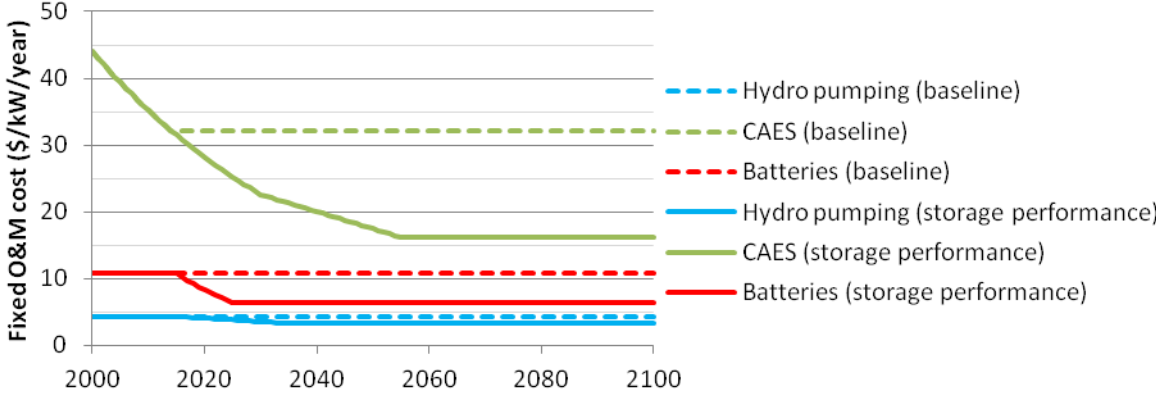
Figure K-2: Evolution of the fixed O&M costs for the Storage Performance scenario, compared to the Baseline scenario (exogenous assumptions).
