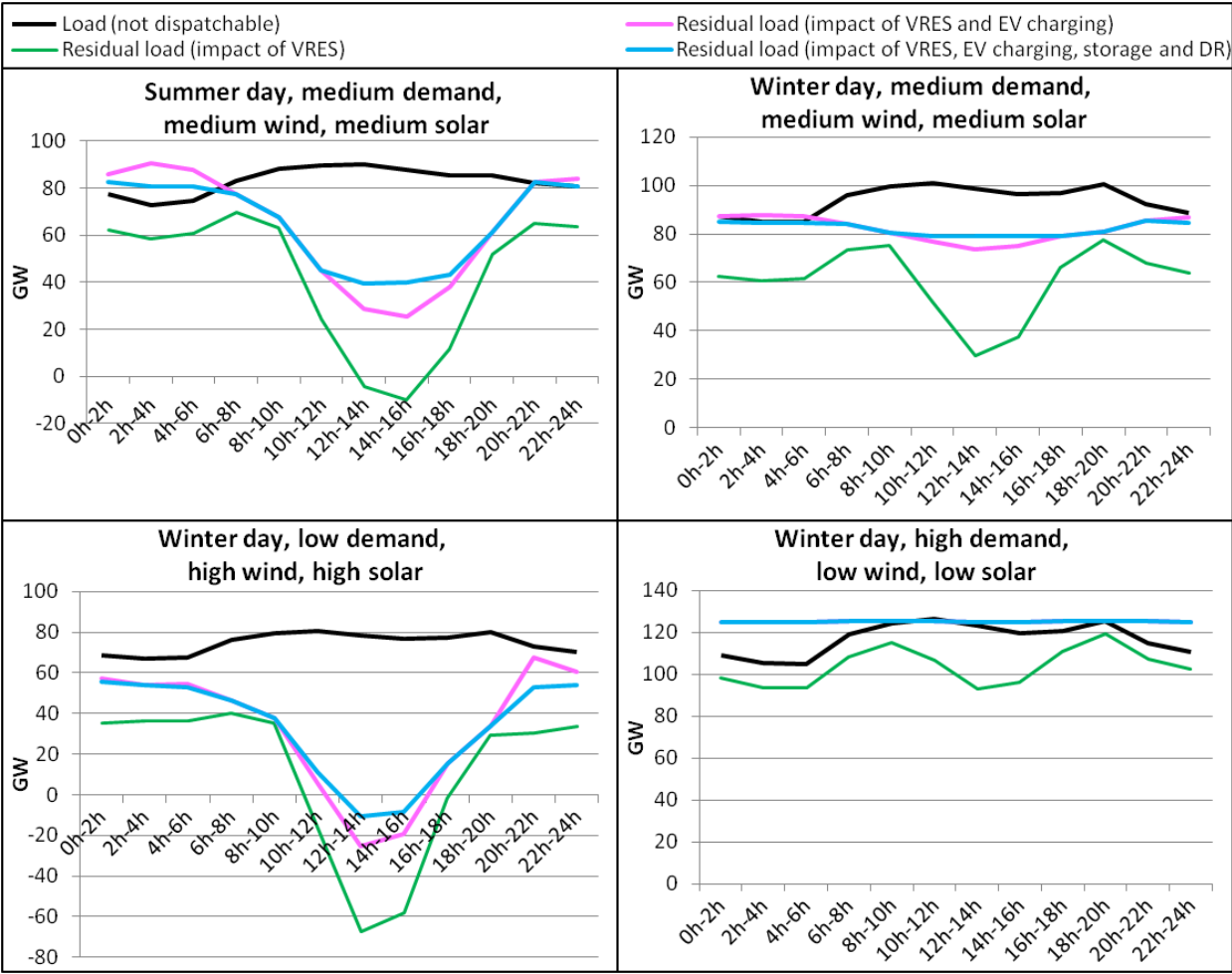
Figure 18: Effects of VRES, EV charging, storage and DR on the load on four different days. France, 2050, baseline scenario (POLES only).
