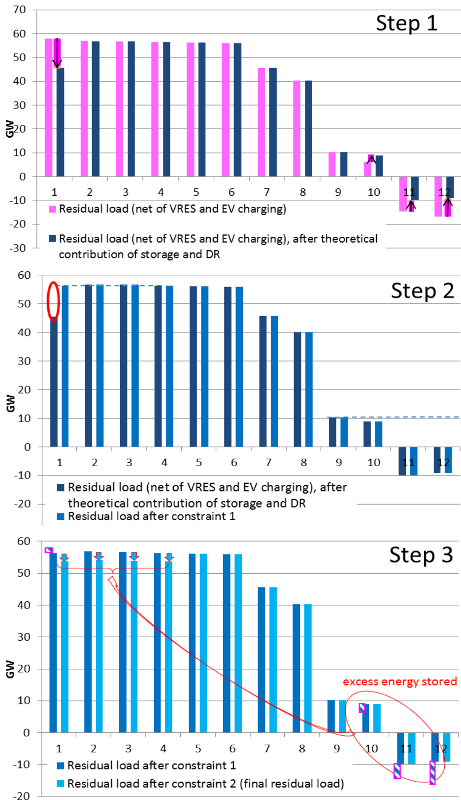
Figure C-2: Focus on the operation of storage and DR on a particular day (medium demand, low wind, and high solar). The different steps are shown: theoretical contribution of storage and DR (top), adding the constraint 1 (middle) and adding the constraint 2 (bottom). France, 2050, baseline scenario (POLES only).
