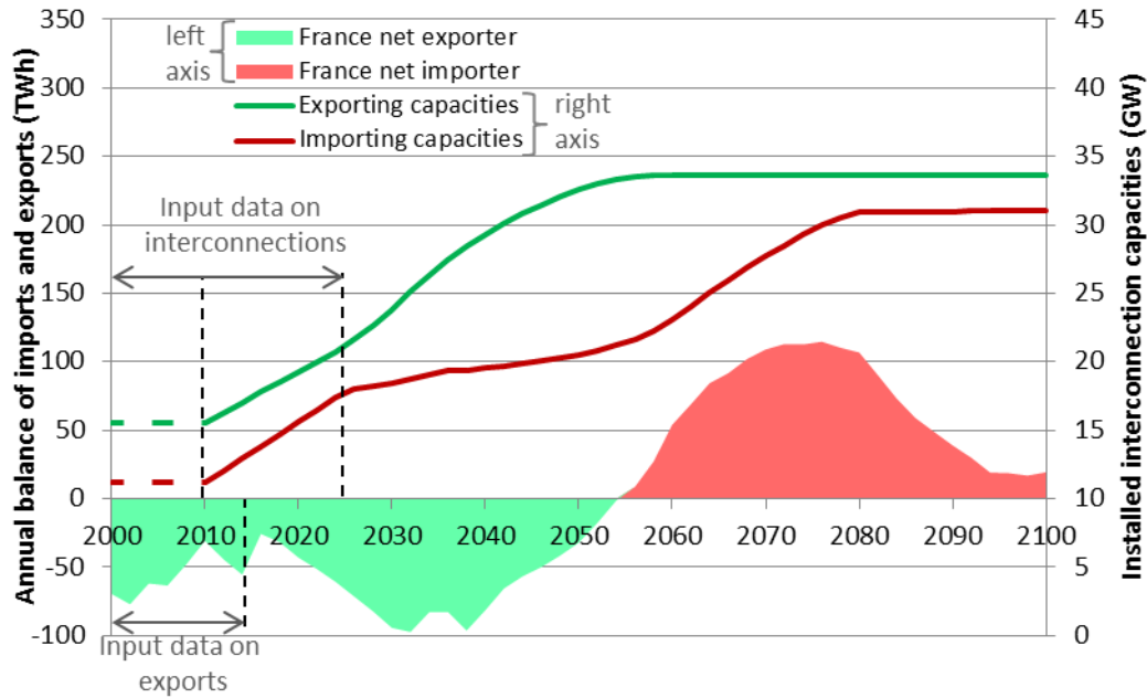
Figure 44: Importing and exporting capacities for France, in relation with net imports and exports. Baseline scenario (POLES+EUCAD).
