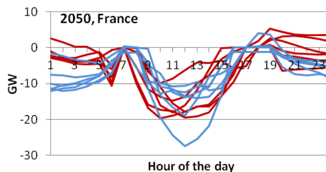
Figure 65: Net power production from EV charging and V2G (8.6 GW of installed V2G); a positive value indicates a net production. France, 2050, baseline scenario (POLES+EUCAD).
