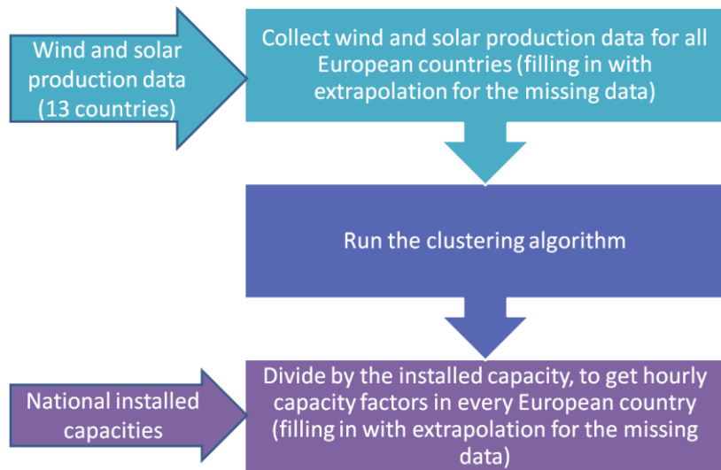
Figure H-5: Diagram of the computation process of the cluster algorithm based on the real production (based on 2012, 2013 and 2014).
