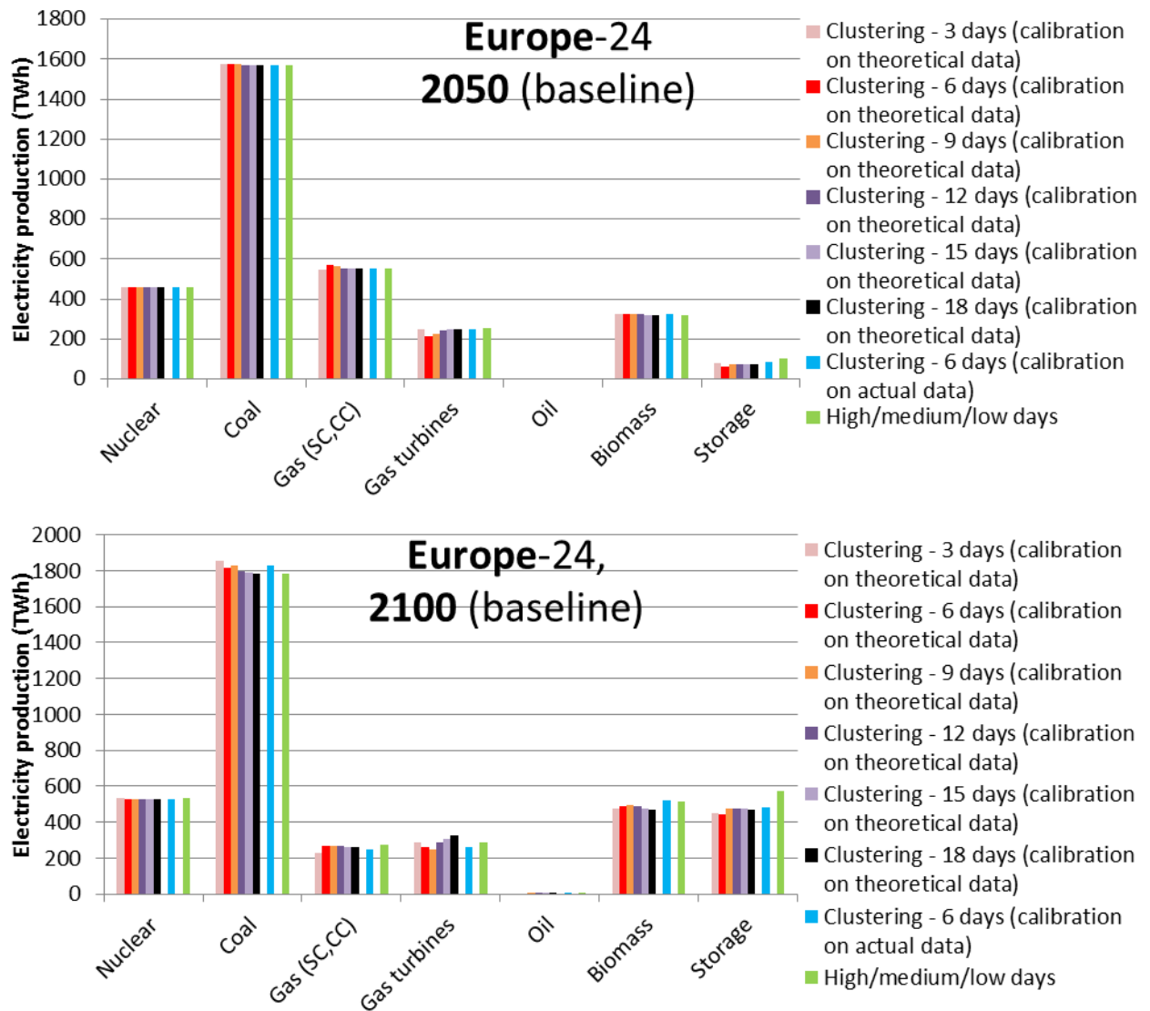
Figure H-7: Annual production by technology for different options of representation of the wind and solar production profiles, for the whole Europe in 2050 (top) and 2100 (bottom) in the baseline scenario (POLES+EUCAD).
