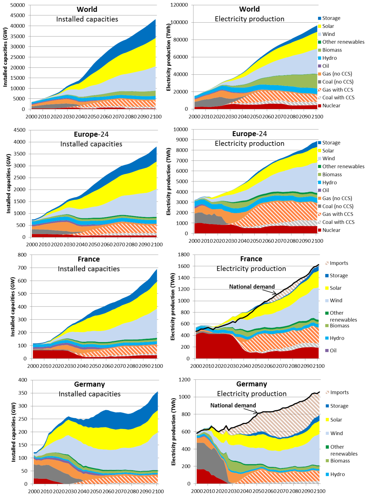
Figure L-4: Installed capacities (left) and electricity production (right) for the whole world, for Europe-24, for France and for Germany, in the climate policy scenario (POLES+EUCAD).
