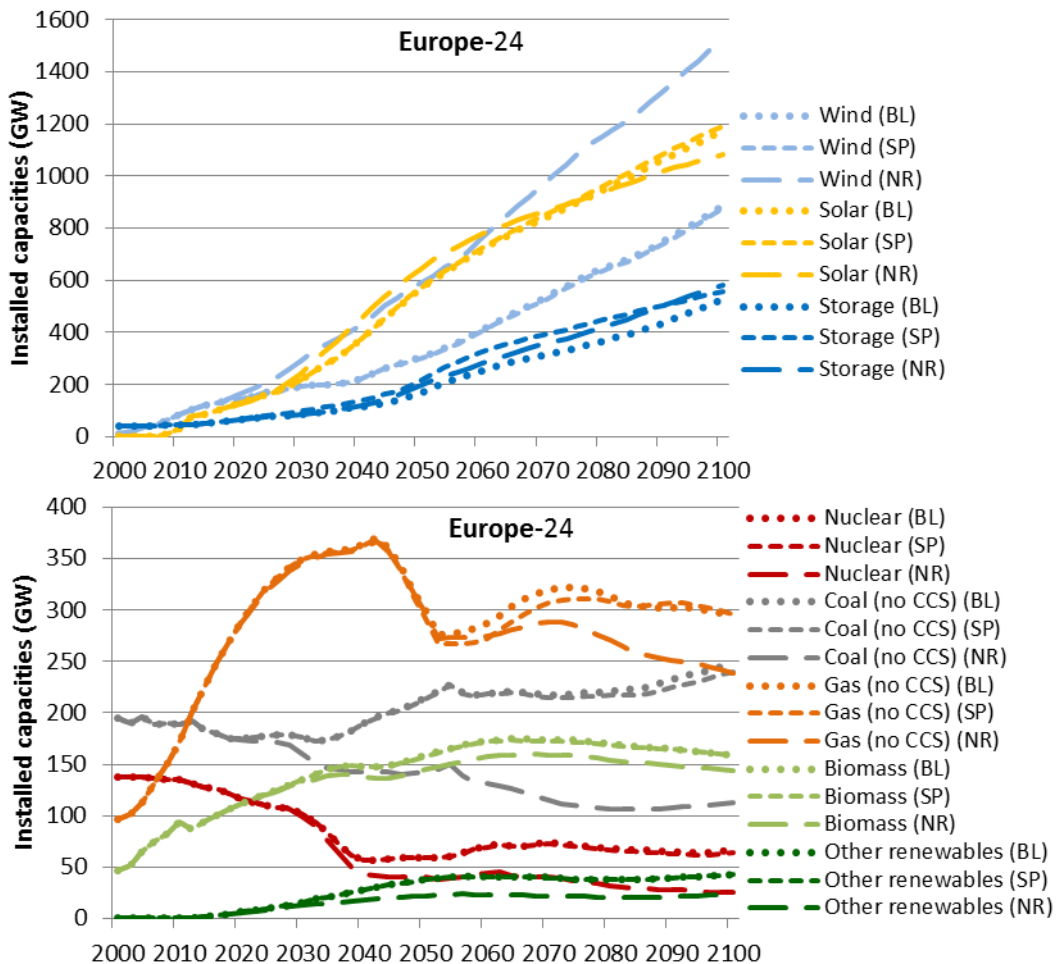
Figure 70: Installed capacities in Europe for the scenarios Baseline (BL), Storage Performance (SP) and New Renewable (NR). Wind, solar and storage power on top; nuclear, coal, gas, biomass and other renewable power on bottom (POLES+EUCAD).
