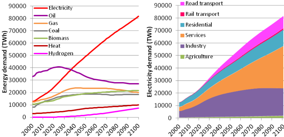
Figure 47: Global energy needs in the baseline scenario; decomposition by end-use fuel (left) and decomposition of electricity needs by sector (right) (POLES+EUCAD).
