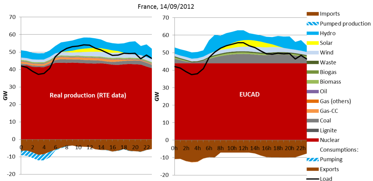
Figure 32: Comparison of the real production data (RTE data; on left) with EUCAD European computation (right). France, 14/09/2012.
