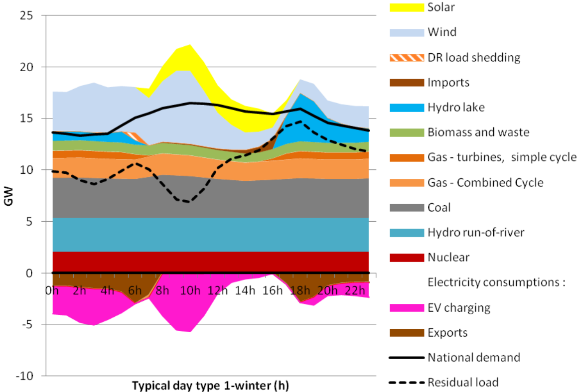
Figure I-1: Operation of the Swiss power system on a typical day of 2050 (day 1-winter), for the baseline scenario. Negative values indicate consumption (POLES+EUCAD).
