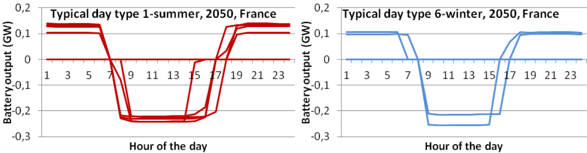
Figure 63: Battery operation (installed capacity of 0.36 GW) in the six typical days of summer (left) and in winter (right). France, 2050, baseline scenario (POLES+EUCAD).
