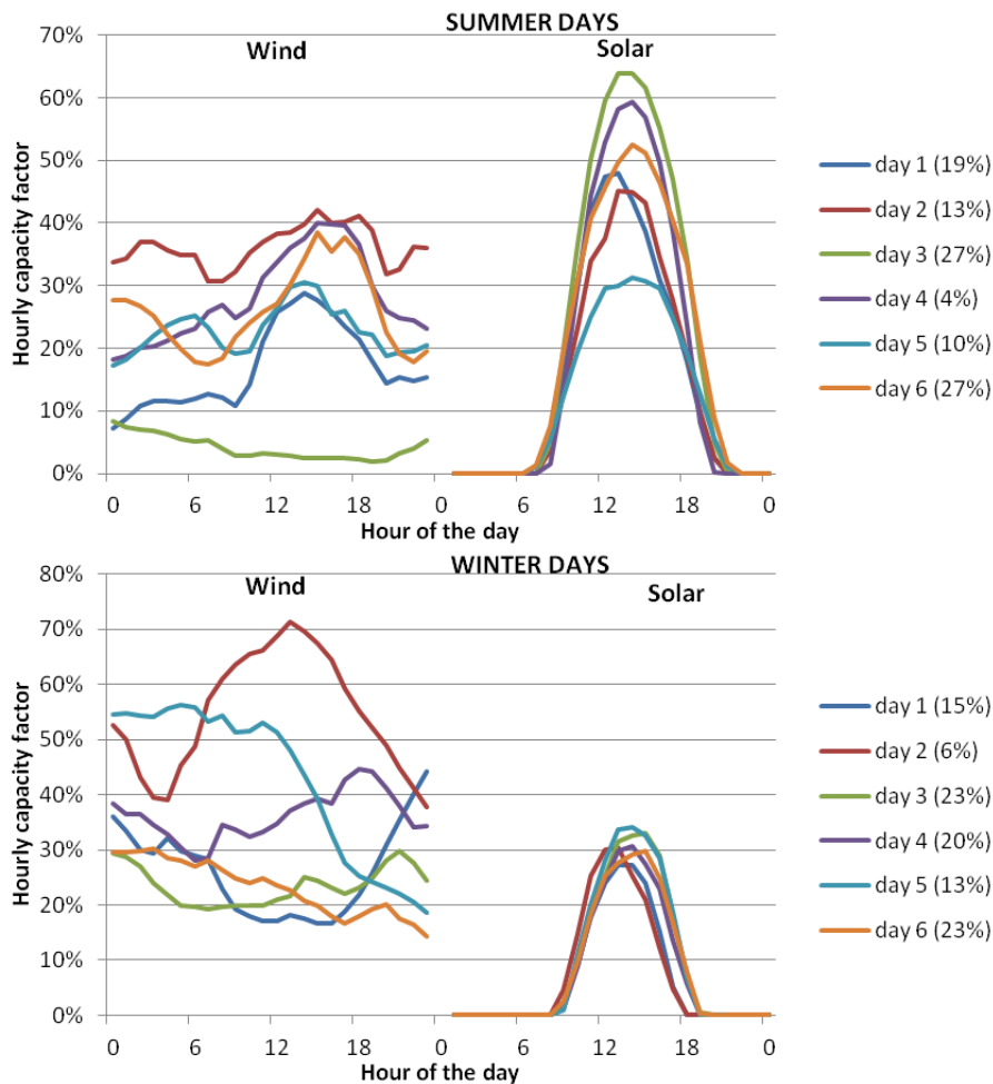
Figure H-6: Wind and solar production profiles in France for six typical days per summer or winter season, based on clusters of the real production (based on 2012, 2013 and 2014 actual productions).
