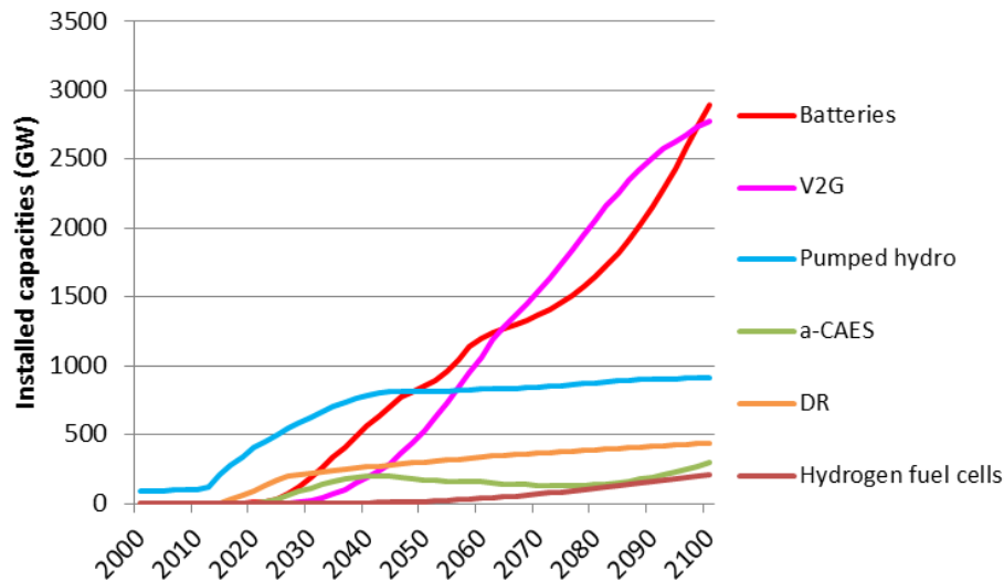
Figure 50: Global development of storage and demand response capacities in the baseline scenario (POLES+EUCAD).
