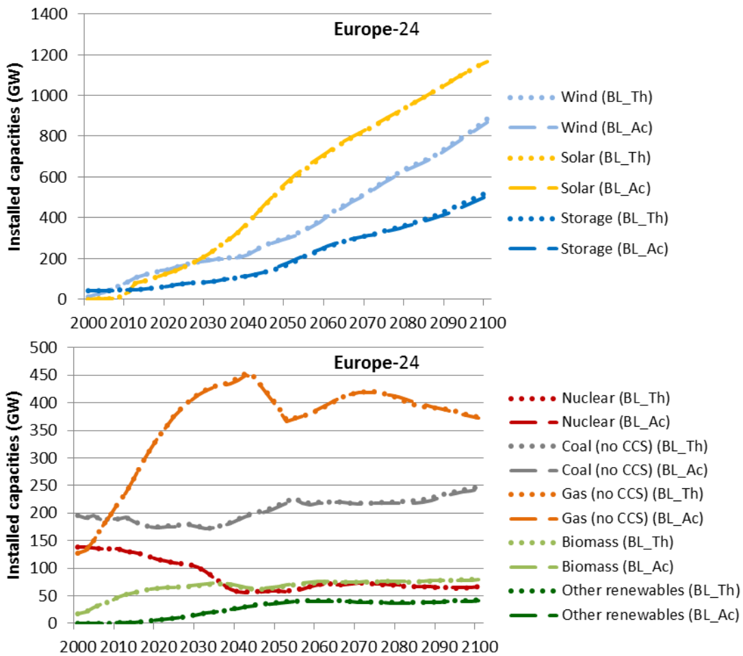
Figure H-8: Installed capacities of the main technologies in Europe, with 6 typical days based on two calibration methods (with theoretical potential BL_Th and with actual production data BL_Ac), for the baseline scenario (POLES+EUCAD).
