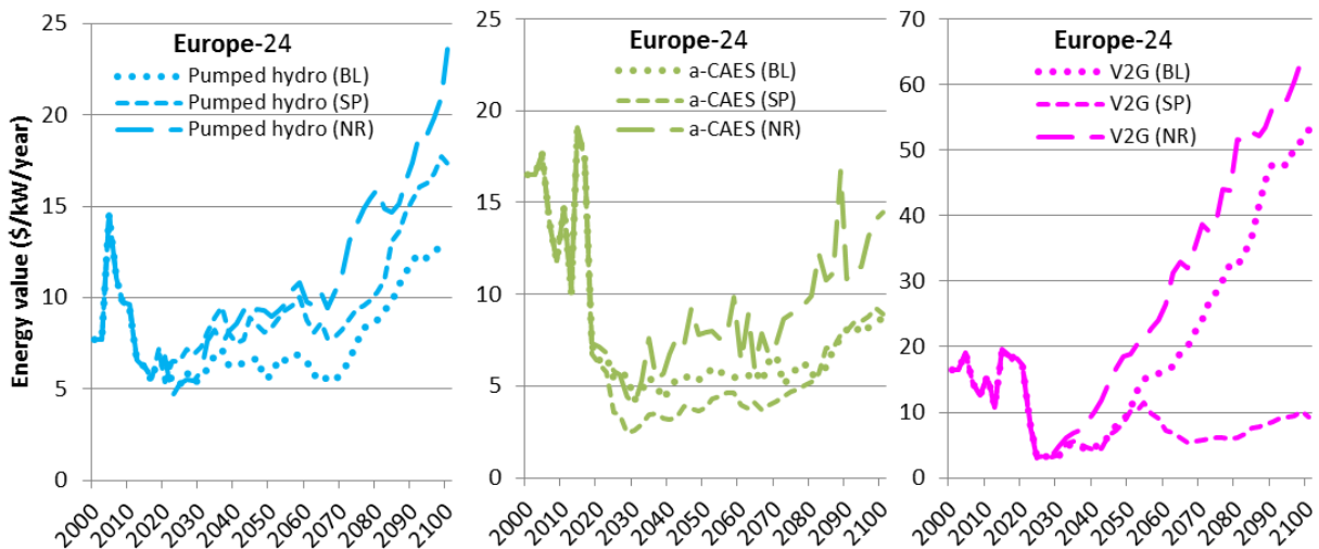
Figure 80: Energy value for pumped hydro (left), a-CAES (centre) and V2G (right), averaged over Europe, for the scenarios Baseline (BL), Storage Performance (SP) and New Renewable (NR) (POLES+EUCAD).
