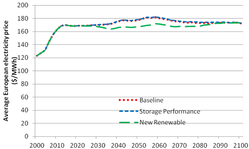
Figure 75: Average European electricity price for all consumption sectors, for the scenarios Baseline (BL), Storage Performance (SP) and New Renewable (NR) (POLES+EUCAD).
