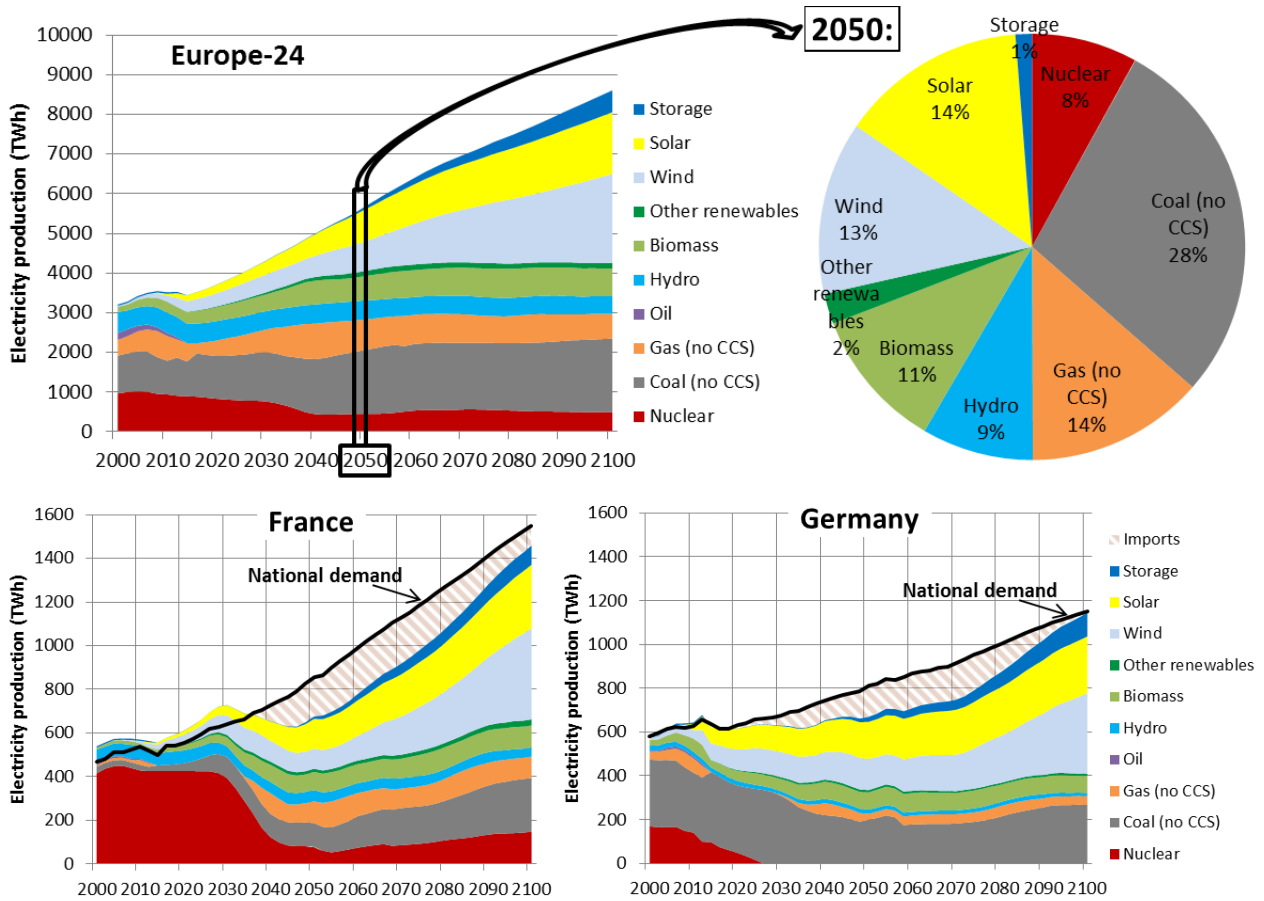
Figure 56: Electricity supply for Europe (top), France (bottom-left) and Germany (bottom-right). Baseline scenario (POLES+EUCAD).
