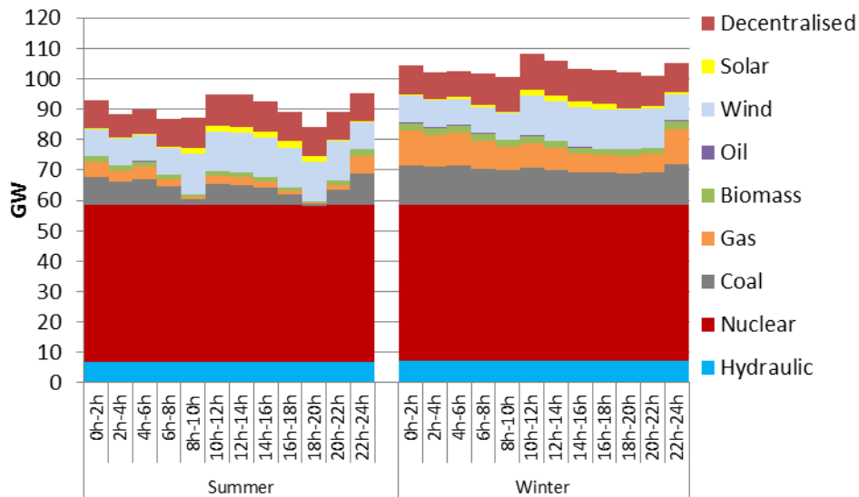
Figure 10: Power plant operation in POLES. The 41 technologies have been aggregated in the graphs in order to keep the representation simple. France, 2050, baseline scenario (former modelling).
