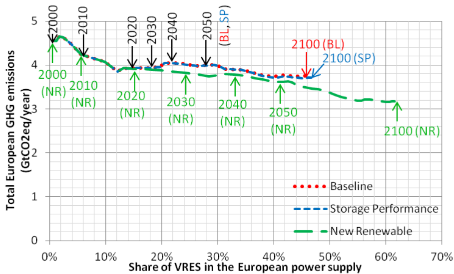
Figure 76: Total GHG emissions in Europe relative to the VRES share in the European power supply, for the scenarios Baseline (BL), Storage Performance (SP) and New Renewable (NR) (POLES+EUCAD).
