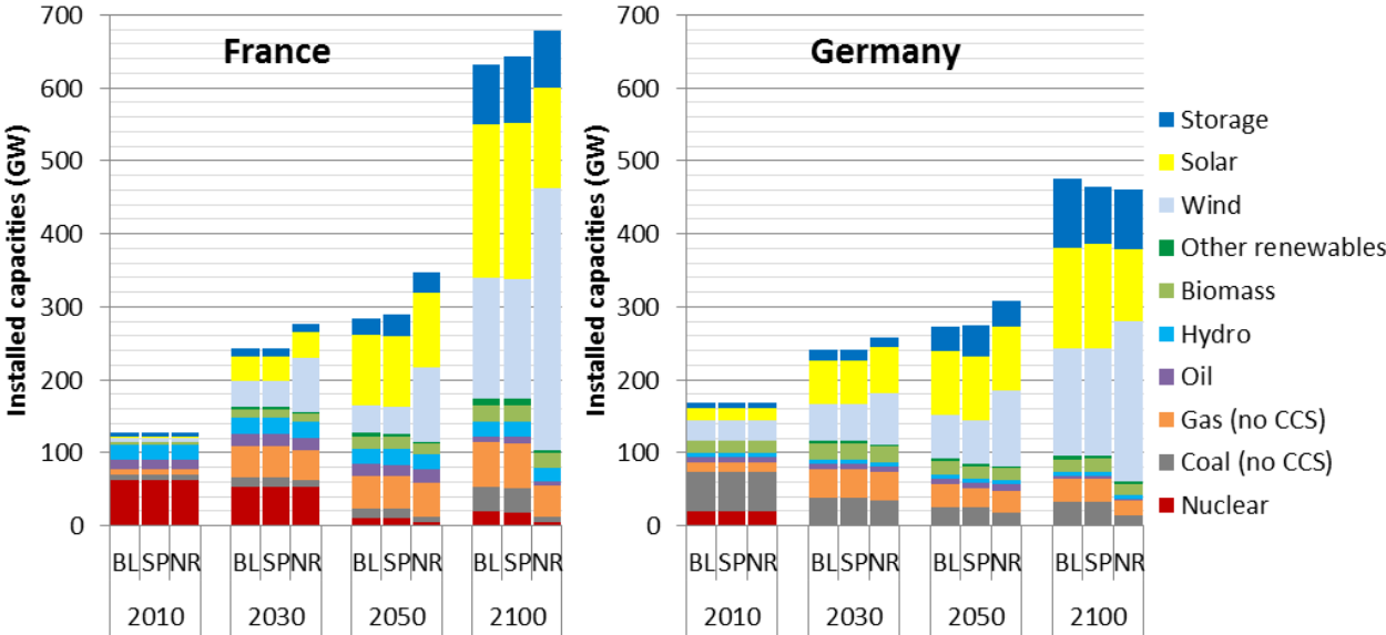
Figure 71: Installed capacities in France (left) and Germany (right), for the scenarios Baseline (BL), Storage Performance (SP) and New Renewable (NR) (POLES+EUCAD).
