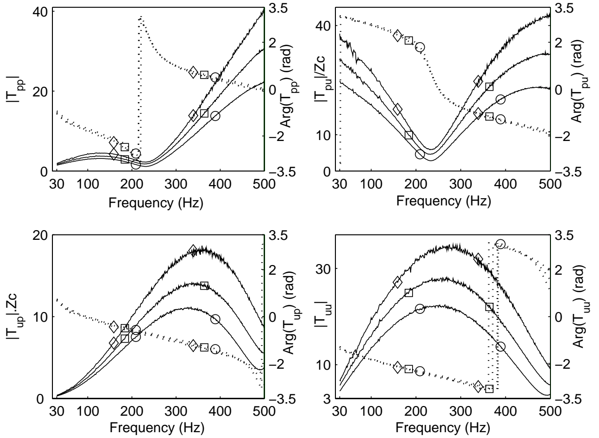
Figure 3.34: Stainless Steel Grids: amplitude (solid line) and phase (dotted line) of the T_{TAC} coefficients in the frequency domain for Q_H = 0 W (circle), Q_H = 36 W (square) and Q_H = 72 W (diamond) - Impedance Method.
