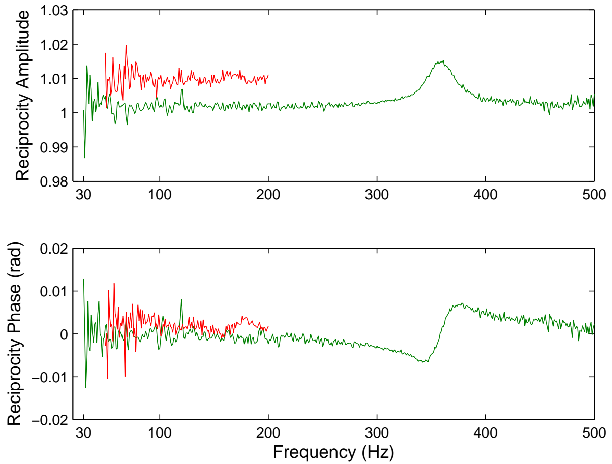
Figure 3.40: Ceramic Catalyst: amplitude and phase of the \mathbf{T}_{TAC} reciprocity in the frequency domain for Q_H = 0 W for the Impedance Method and for the Two-Load Method (lines of narrower frequency range).
