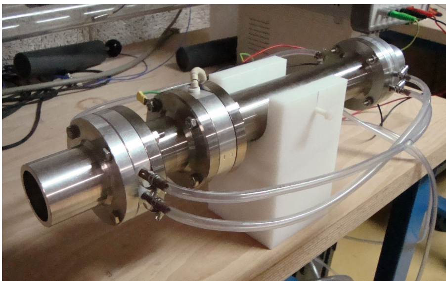
Figure 3.2: ThermoAcoustic Core.
