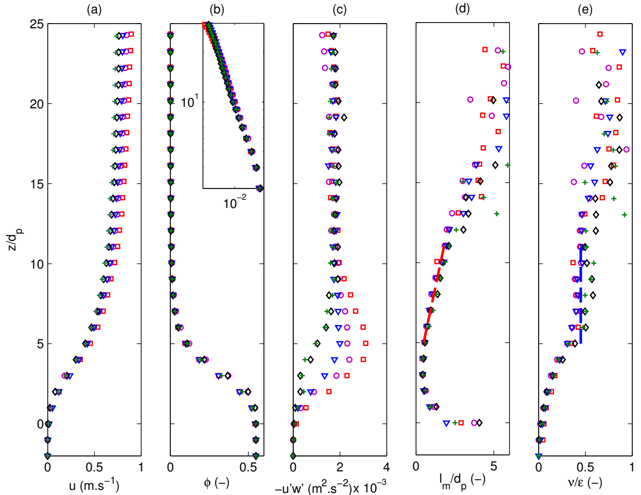
FIGURE 6.1 – Sensitivity to the non-uniformity of the flow. Mean profiles of velocity (a), concentration (b), turbulent shear stress (c), mixing length (d) and ratio between momentum and particulate diffusivities (e) evaluated on the intervals t \in [30 - 36] s (squares), t \in [40 - 46] s (circles), t \in [50 - 56] s (triangles), t \in [60 - 66] s (diamonds), t \in [70 - 76] s (pluses). The dashed line on panel (d) represents the slope \kappa = 0.2 . The dashed line on panel (e) represents the Schmidt number \sigma_s = 0.45 .
